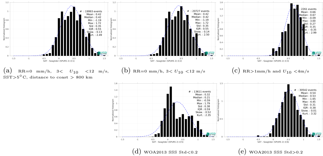
Figure 13: Normalized histogram of \Delta SSS (SMOS SSS L3 v2 - 9-Days (BEC) - Seaglider (SPURS 2)) for 5 different subdatasets corresponding to: RR=0 mm/h, 3 < U_{10} < 12 m/s, SST>5°C, distance to coast > 800 km (a), RR=0 mm/h, 3 < U_{10} < 12 m/s (b), RR>1mm/h and U_{10} < 4 m/s (c), WOA2013 SSS Std<0.2 (d), WOA2013 SSS Std>0.2 (e).
