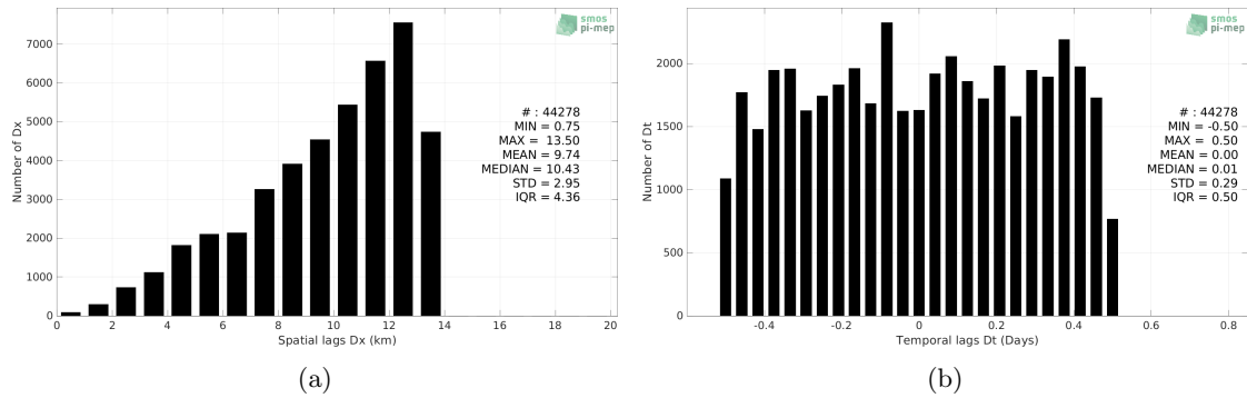
Figure 5: Histograms of the spatial (a) and temporal (b) lags between the location/time of the Seaglider (SPURS 2) measurement and the date of the corresponding SMOS SSS L3 v2 - 9-Days (BEC) SSS pixel.
