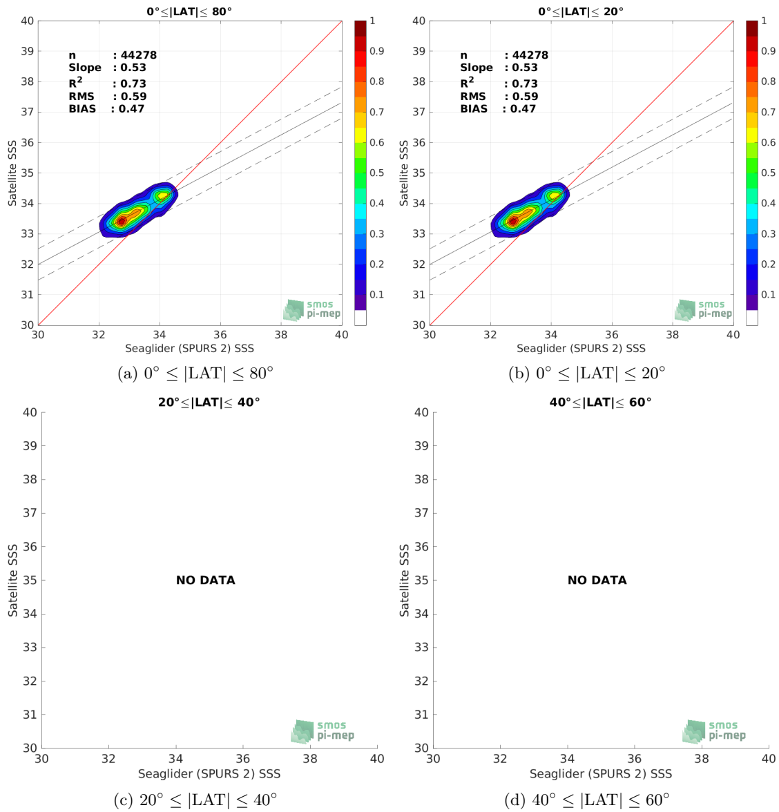
Figure 9: Contour maps of the concentration of SMOS SSS L3 v2 - 9-Days (BEC) SSS (y-axis) versus Seaglider (SPURS 2) SSS (x-axis) at match-up pairs for different latitude bands. For each plot, the red line shows x=y . The black thin and dashed lines indicate a linear fit through the data cloud and the \pm 95\% confidence levels, respectively. The number match-up pairs n , the slope and R^2 coefficient of the linear fit, the root mean square (RMS) and the mean bias between satellite and in situ data are indicated for each latitude band in each plots.
