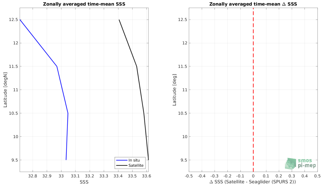
Figure 8: Left panel: Zonal mean SSS from SMOS SSS L3 v2 - 9-Days (BEC) satellite product (black) and from Seaglider (SPURS 2) (blue). Right panel: Zonal mean of \Delta SSS (Satellite - Seaglider (SPURS 2)) for all the collected Pi-MEP match-up pairs estimated over the full satellite product period.
