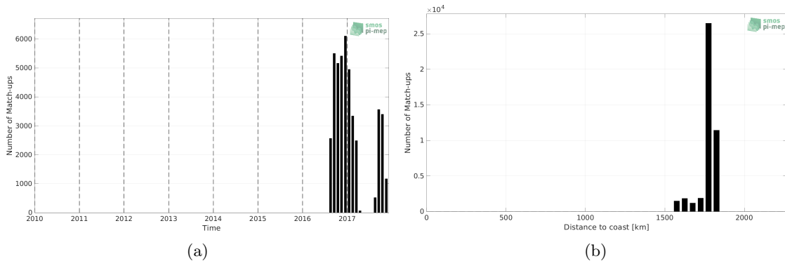
Figure 1: Number of match-ups between Seaglider (SPURS 2) and SMOS SSS L3 v2 - 9-Days (BEC) SSS as a function of time (a) and as function of the distance to coast (b) over the SPURS 2 Pi-MEP region and for the full satellite product period.
