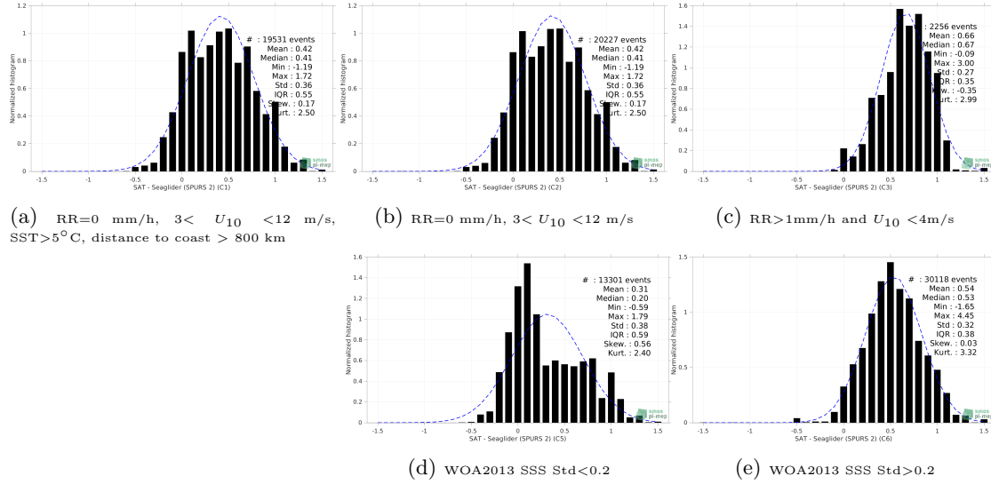
Figure 13: Normalized histogram of \Delta SSS (SMOS SSS L3 v2 - 9-Days (BEC) - Seaglider (SPURS 2)) for 5 different subdatasets corresponding to: RR=0 mm/h, 3 < U_{10} < 12 m/s, SST > 5°C, distance to coast > 800 km (a), RR=0 mm/h, 3 < U_{10} < 12 m/s (b), RR > 1mm/h and U_{10} < 4 m/s (c), WOA2013 SSS Std < 0.2 (d), WOA2013 SSS Std > 0.2 (e).
