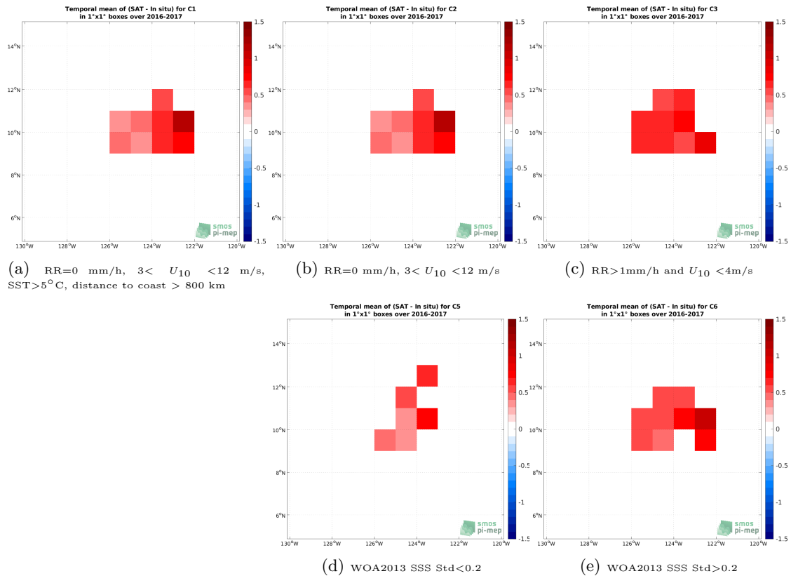
Figure 12: Temporal mean gridded over spatial boxes of size 1^\circ \times 1^\circ of \Delta SSS (SMOS SSS L3 v2 - 9-Days (BEC) - Seaglider (SPURS 2)) for 5 different subdatasets corresponding to:RR=0 mm/h, 3 < U_{10} < 12 m/s, SST >5^\circ C, distance to coast > 800 km (a), RR=0 mm/h, 3 < U_{10} < 12 m/s (b), RR >1 mm/h and U_{10} < 4 m/s (c), WOA2013 SSS Std <0.2 (d), WOA2013 SSS Std >0.2 (e).
