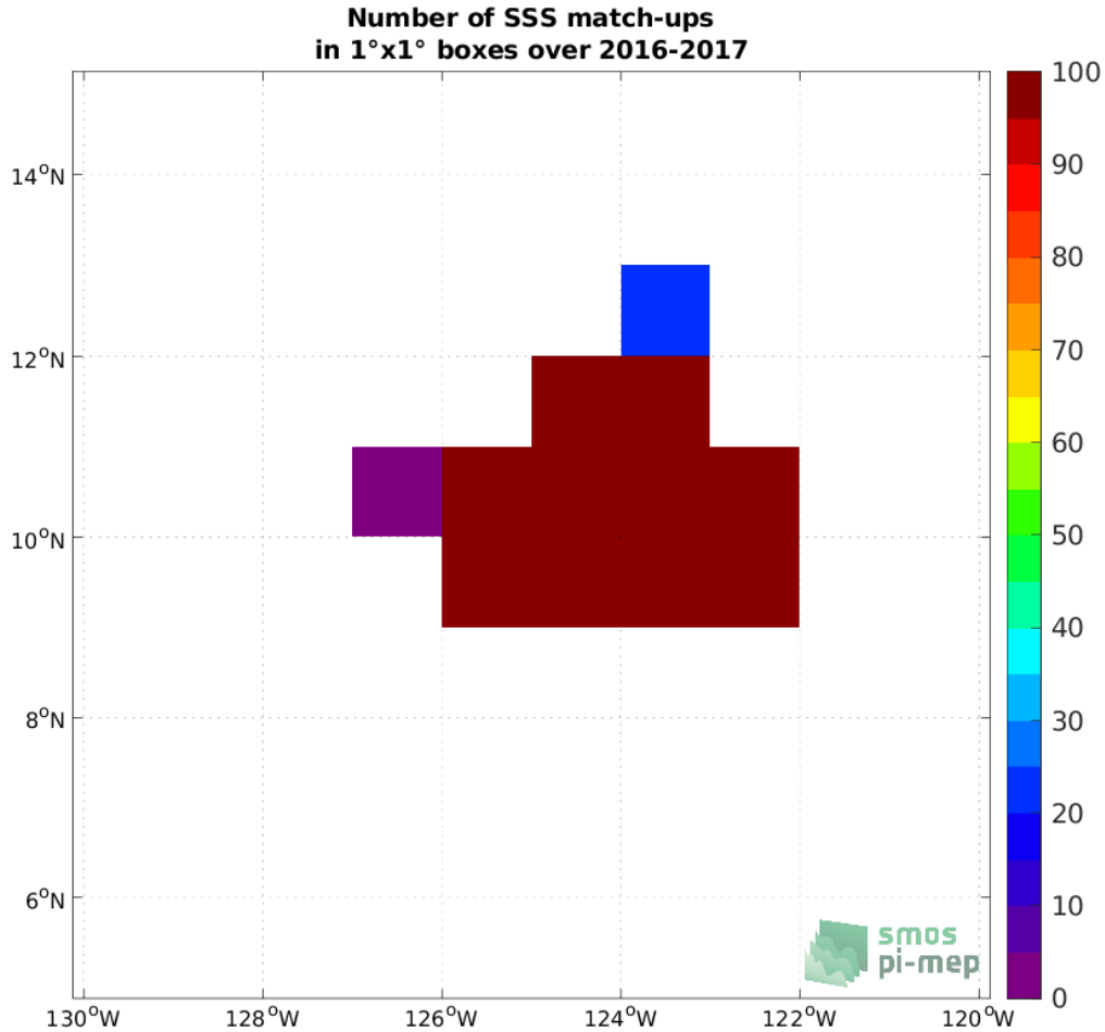
Figure 4: Number of SSS match-ups between Seaglider (SPURS 2) SSS and the SMOS SSS L3 v2 - 9-Days (BEC) SSS product for the SPURS 2 Pi-MEP region over 1^\circ \times 1^\circ boxes and for the full satellite product period.
