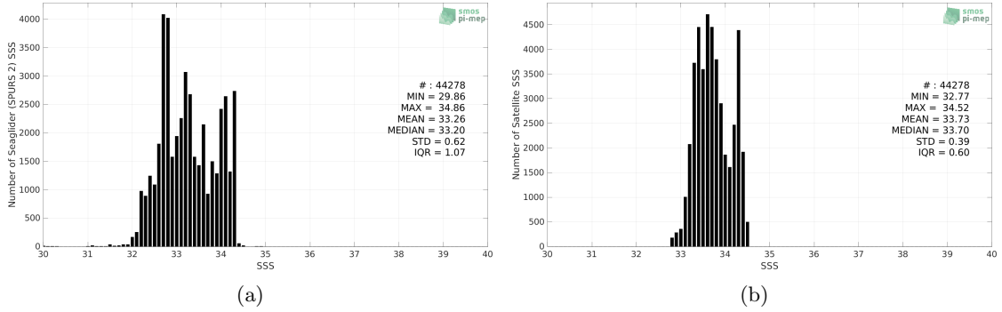
Figure 2: Histograms of SSS from Seaglider (SPURS 2) (a) and SMOS SSS L3 v2 - 9-Days (BEC) (b) considering all match-up pairs per bins of 0.1 over the SPURS 2 Pi-MEP region and for the full satellite product period.
