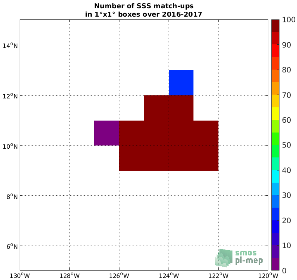
Figure 3: Number of SSS match-ups between Seagliders SSS and the SMOS SSS L3 v2 - 9-Days (BEC) SSS product for the SPURS 2 Pi-MEP region over 1°x1° boxes and for the full satellite product period.
