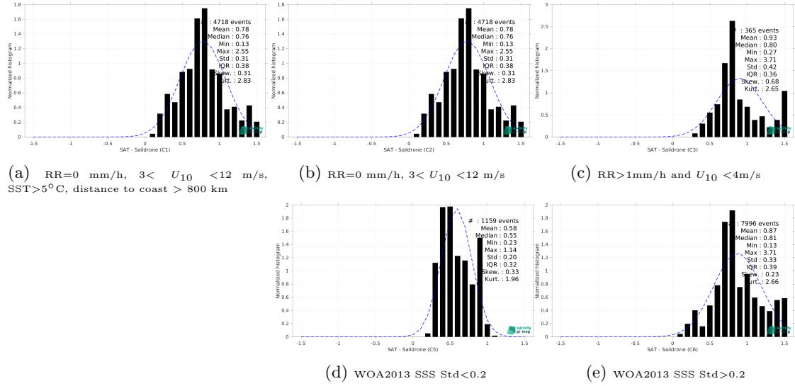
Figure 15: Normalized histogram of \Delta SSS (SMOS SSS L3 v2 - 9-Days (BEC) - Saildrone) for 5 different subdatasets corresponding to: RR=0 mm/h, 3 < U_{10} < 12 m/s, SST >5^{\circ} C, distance to coast > 800 km (a), RR=0 mm/h, 3 < U_{10} < 12 m/s (b), RR >1 mm/h and U_{10} < 4 m/s (c), WOA2013 SSS Std <0.2 (d), WOA2013 SSS Std >0.2 (e).
