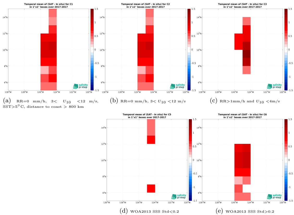
Figure 14: Temporal mean gridded over spatial boxes of size 1^\circ \times 1^\circ of \Delta SSS (SMOS SSS L3 v2 - 9-Days (BEC) - Saildrone) for 5 different subdatasets corresponding to:RR=0 mm/h, 3 < U_{10} < 12 m/s, SST >5^\circ C, distance to coast > 800 km (a), RR=0 mm/h, 3 < U_{10} < 12 m/s (b), RR >1 mm/h and U_{10} < 4 m/s (c), WOA2013 SSS Std <0.2 (d), WOA2013 SSS Std >0.2 (e).
