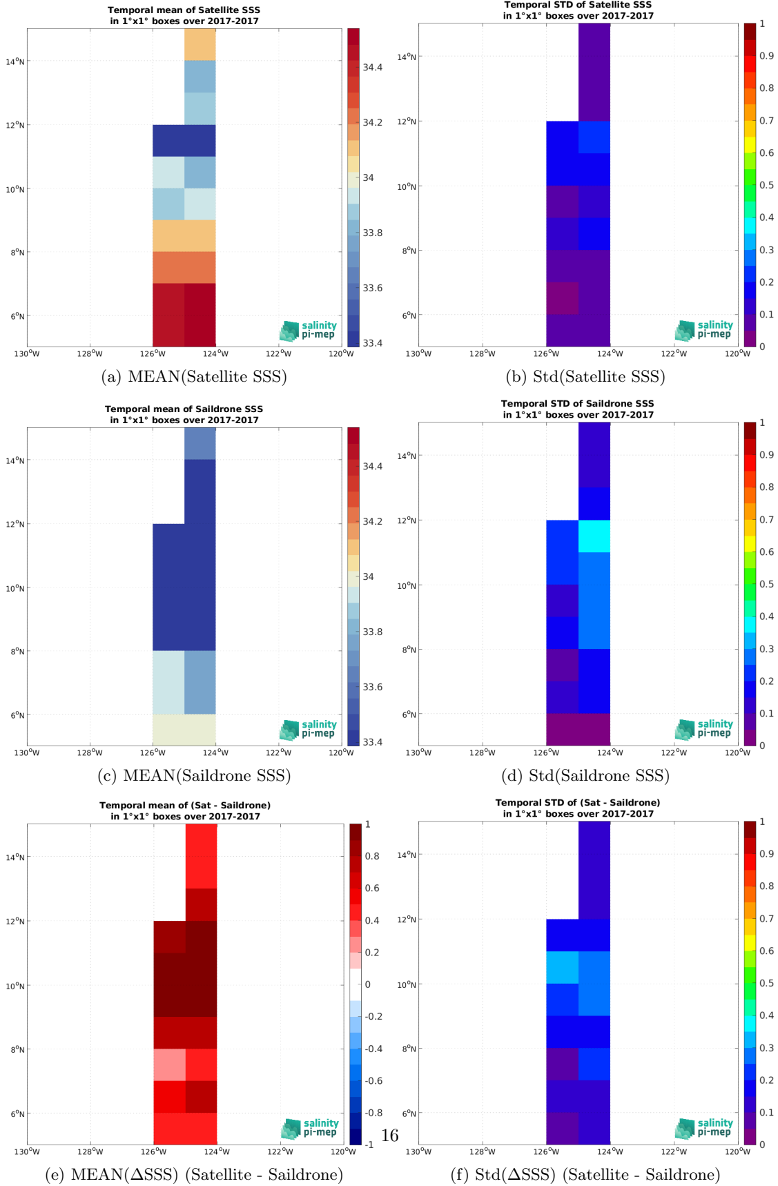
Figure 7: Temporal mean (left) and Std (right) of SSS from SMOS SSS L3 v2 - 9-Days (BEC) (top), Saildrone (middle), and of \Delta SSS (Satellite - Saildrone). Only match-up pairs are used to generate these maps.
