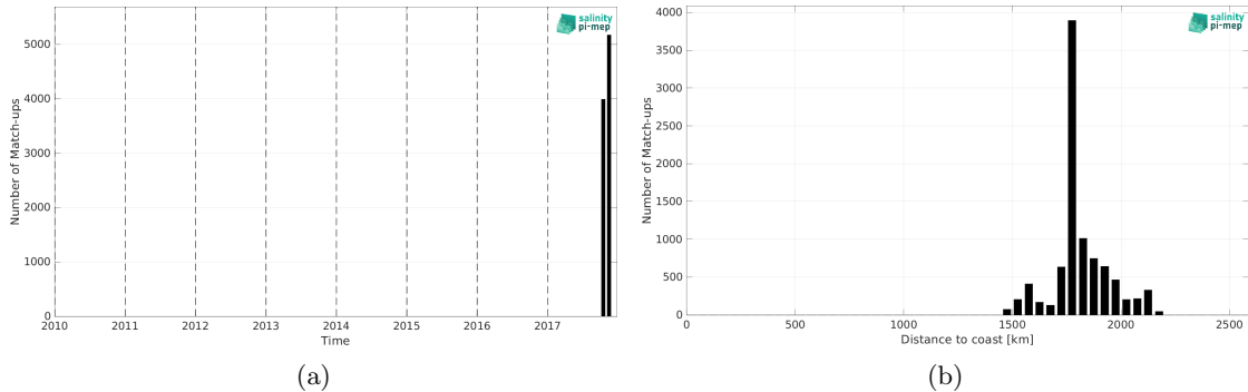
Figure 2: Number of match-ups between Saildrone and SMOS SSS L3 v2 - 9-Days (BEC) SSS as a function of time (a) and as function of the distance to coast (b) over the SPURS 2 Pi-MEP region and for the full satellite product period.
