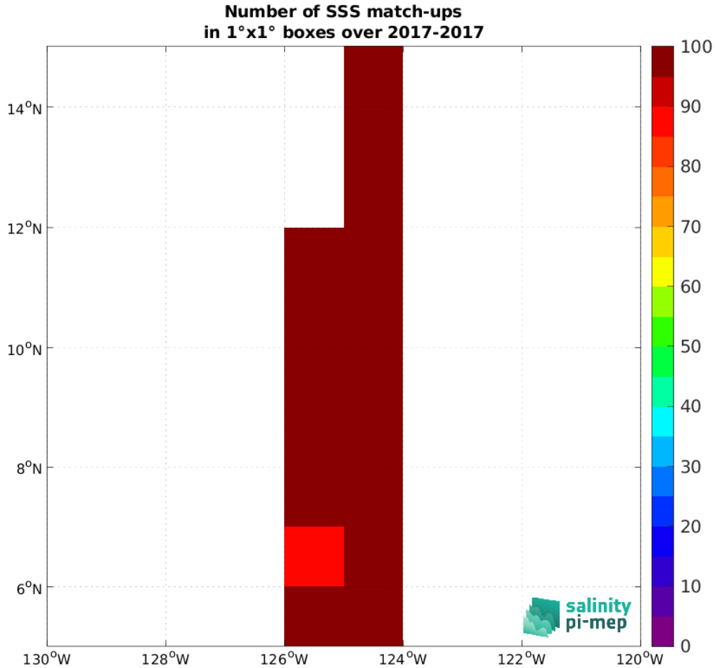
Figure 5: Number of SSS match-ups between Saildrone SSS and the SMOS SSS L3 v2 - 9-Days (BEC) SSS product for the SPURS 2 Pi-MEP region over 1^\circ \times 1^\circ boxes and for the full satellite product period.
