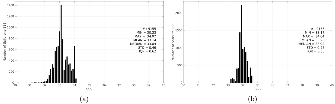
Figure 3: Histograms of SSS from Saildrone (a) and SMOS SSS L3 v2 - 9-Days (BEC) (b) considering all match-up pairs per bins of 0.1 over the SPURS 2 Pi-MEP region and for the full satellite product period.
