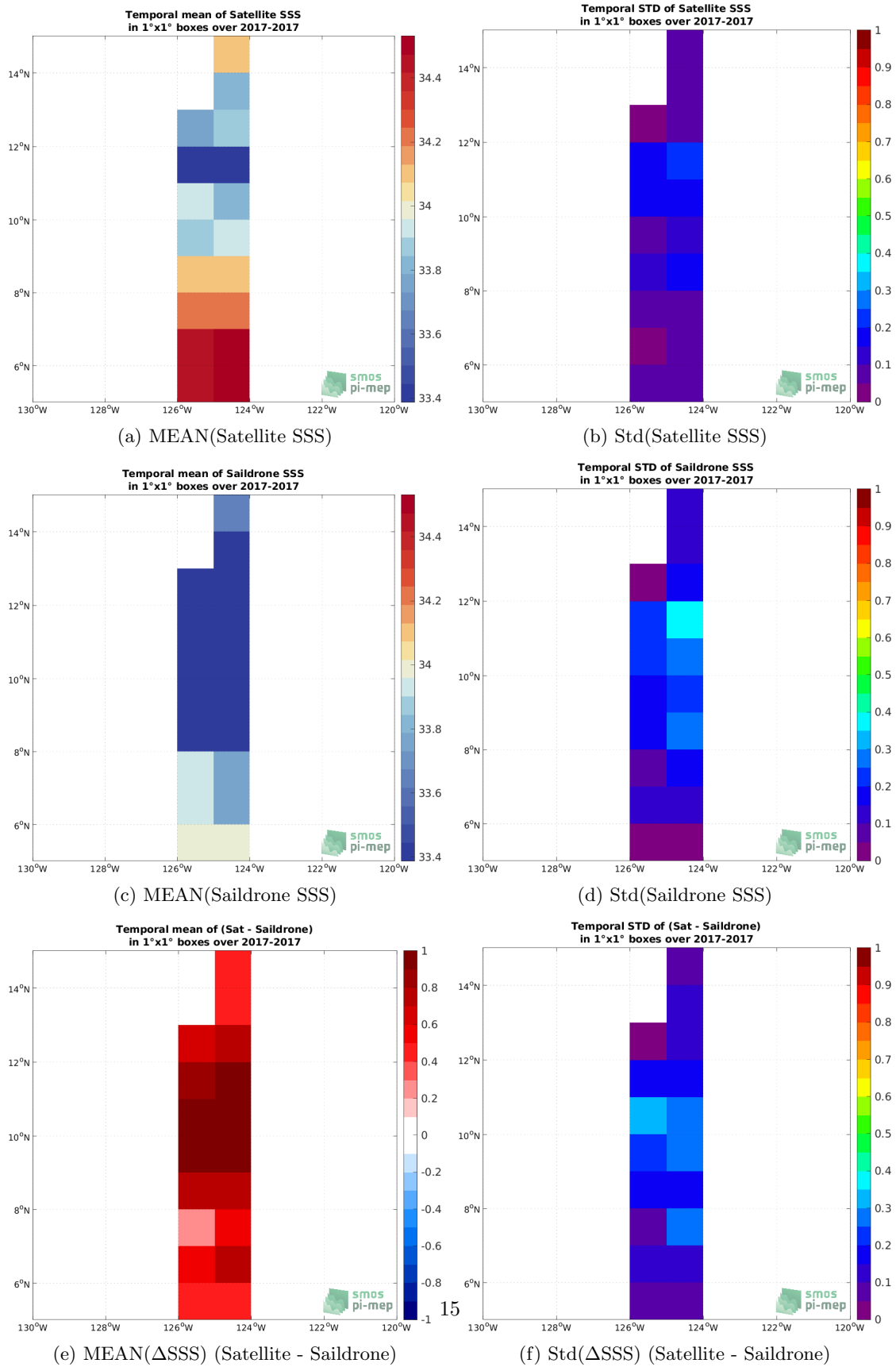
Figure 6: Temporal mean (left) and Std (right) of SSS from SMOS SSS L3 v2 - 9-Days (BEC) (top), Saildrone (middle), and of \Delta SSS (Satellite - Saildrone). Only match-up pairs are used to generate these maps.
