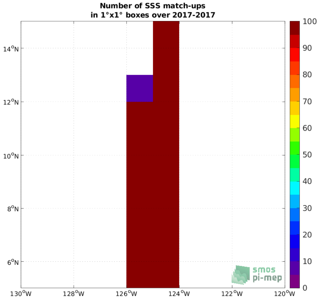
Figure 4: Number of SSS match-ups between Saildrone SSS and the SMOS SSS L3 v2 - 9-Days (BEC) SSS product for the SPURS 2 Pi-MEP region over 1^\circ \times 1^\circ boxes and for the full satellite product period.
