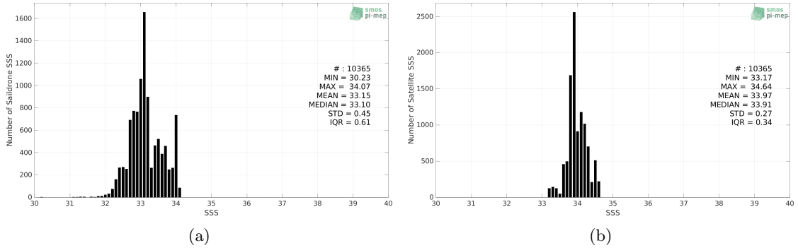
Figure 2: Histograms of SSS from Saildrone (a) and SMOS SSS L3 v2 - 9-Days (BEC) (b) considering all match-up pairs per bins of 0.1 over the SPURS 2 Pi-MEP region and for the full satellite product period.
