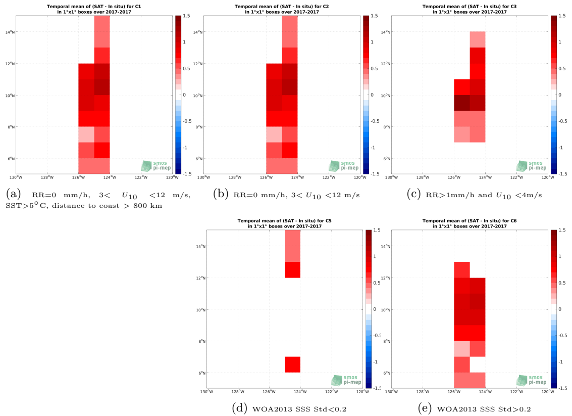
Figure 12: Temporal mean gridded over spatial boxes of size 1^\circ \times 1^\circ of \Delta SSS (SMOS SSS L3 v2 - 9-Days (BEC) - Saildrone) for 5 different subdatasets corresponding to:RR=0 mm/h, 3 < U_{10} < 12 m/s, SST >5^\circ\text{C} , distance to coast > 800 km (a), RR=0 mm/h, 3 < U_{10} < 12 m/s (b), RR >1 mm/h and U_{10} < 4 m/s (c), WOA2013 SSS Std <0.2 (d), WOA2013 SSS Std >0.2 (e).
