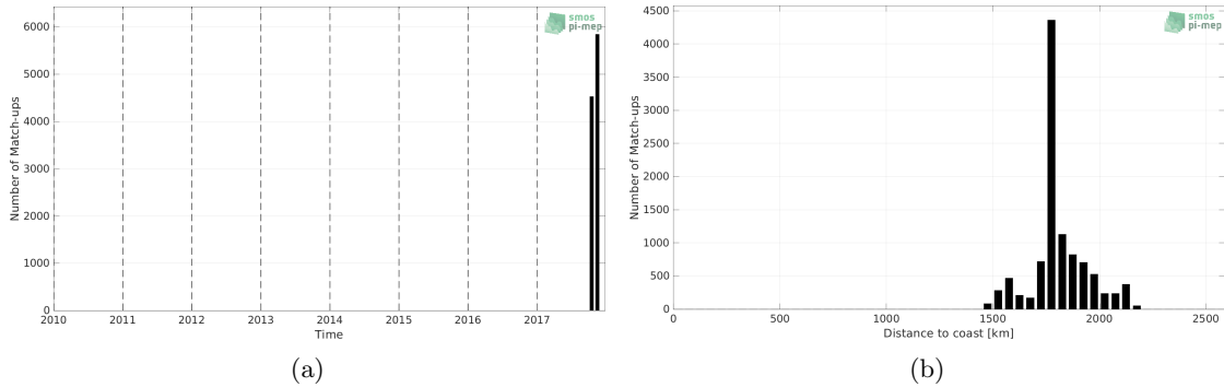
Figure 1: Number of match-ups between Saildrone and SMOS SSS L3 v2 - 9-Days (BEC) SSS as a function of time (a) and as function of the distance to coast (b) over the SPURS 2 Pi-MEP region and for the full satellite product period.
