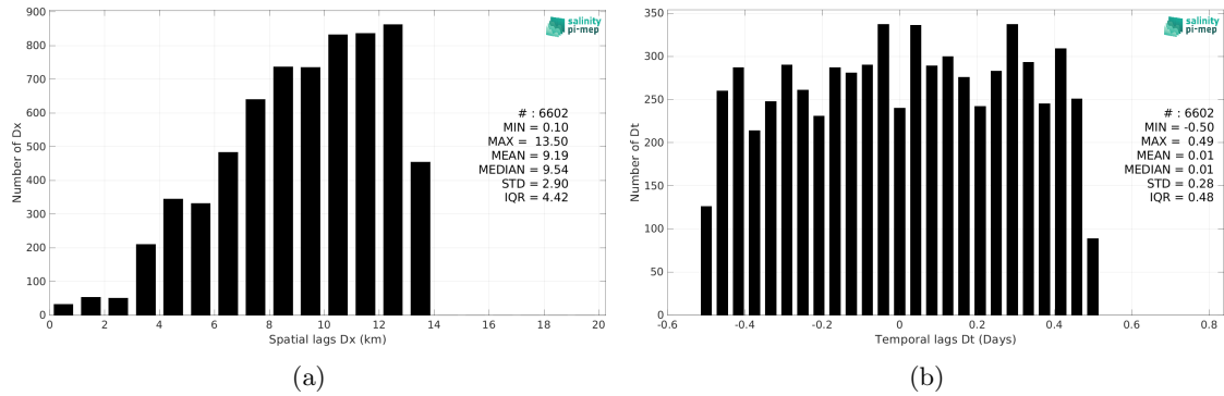
Figure 5: Histograms of the spatial (a) and temporal (b) lags between the location/time of the Saildrone (SPURS 2) measurement and the date of the corresponding SMOS SSS L3 v2 - 9-Days (BEC) SSS pixel.
