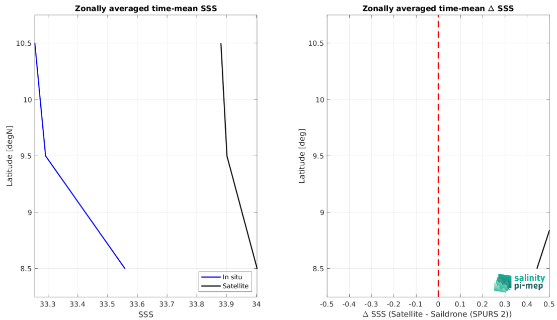
Figure 8: Left panel: Zonal mean SSS from SMOS SSS L3 v2 - 9-Days (BEC) satellite product (black) and from Sairdron (SPURS 2) (blue). Right panel: Zonal mean of \Delta SSS (Satellite - Sairdron (SPURS 2)) for all the collected Pi-MEP match-up pairs estimated over the full satellite product period.
