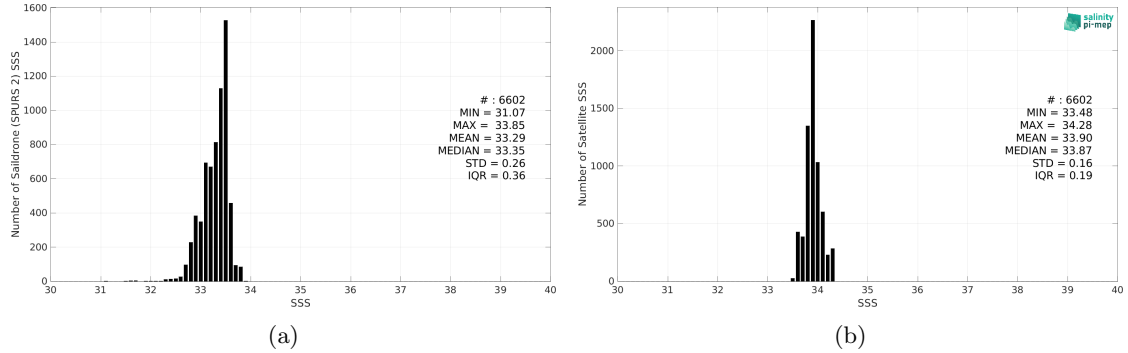
Figure 2: Histograms of SSS from Saildrone (SPURS 2) (a) and SMOS SSS L3 v2 - 9-Days (BEC) (b) considering all match-up pairs per bins of 0.1 over the SPURS 2 Pi-MEP region and for the full satellite product period.
