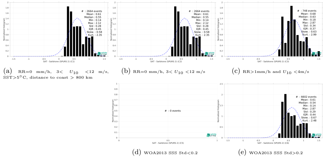
Figure 13: Normalized histogram of \Delta SSS (SMOS SSS L3 v2 - 9-Days (BEC) - Saildrone (SPURS 2)) for 5 different subdatasets corresponding to: RR=0 mm/h, 3 < U_{10} < 12 m/s, SST > 5°C, distance to coast > 800 km (a), RR=0 mm/h, 3 < U_{10} < 12 m/s (b), RR > 1mm/h and U_{10} < 4 m/s (c), WOA2013 SSS Std < 0.2 (d), WOA2013 SSS Std > 0.2 (e).
