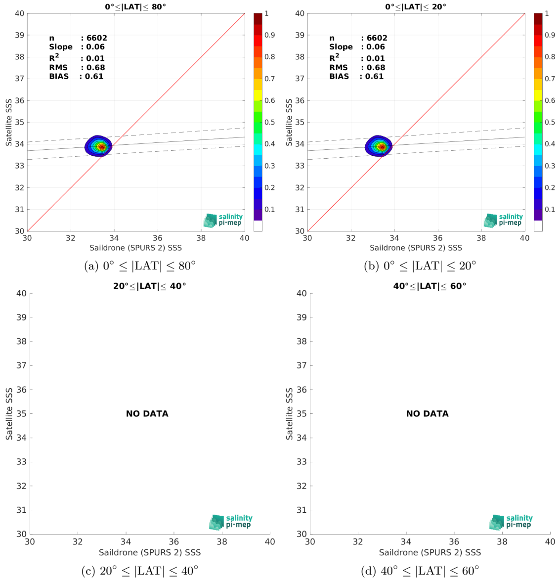
Figure 9: Contour maps of the concentration of SMOS SSS L3 v2 - 9-Days (BEC) SSS (y-axis) versus Saildrone (SPURS 2) SSS (x-axis) at match-up pairs for different latitude bands. For each plot, the red line shows x=y . The black thin and dashed lines indicate a linear fit through the data cloud and the \pm 95\% confidence levels, respectively. The number match-up pairs n , the slope and R^2 coefficient of the linear fit, the root mean square (RMS) and the mean bias between satellite and in situ data are indicated for each latitude band in each plots.
