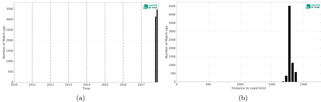
Figure 1: Number of match-ups between Saildrone (SPURS 2) and SMOS SSS L3 v2 - 9-Days (BEC) SSS as a function of time (a) and as function of the distance to coast (b) over the SPURS 2 Pi-MEP region and for the full satellite product period.
