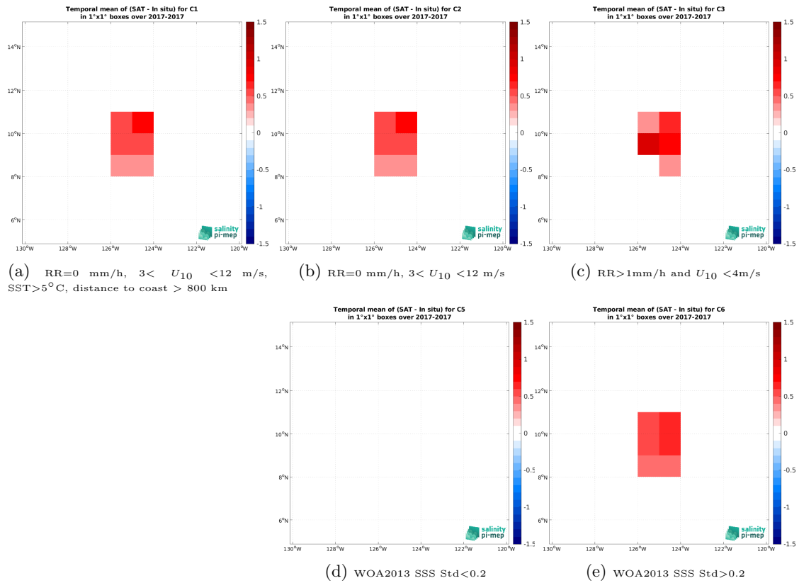
Figure 12: Temporal mean gridded over spatial boxes of size 1^\circ \times 1^\circ of \Delta SSS (SMOS SSS L3 v2 - 9-Days (BEC) - Sailability (SPURS 2)) for 5 different subdatasets corresponding to:RR=0 mm/h, 3 < U_{10} < 12 m/s, SST >5^\circ\text{C} , distance to coast > 800 km (a), RR=0 mm/h, 3 < U_{10} < 12 m/s (b), RR >1 mm/h and U_{10} < 4 m/s (c), WOA2013 SSS Std <0.2 (d), WOA2013 SSS Std >0.2 (e).
