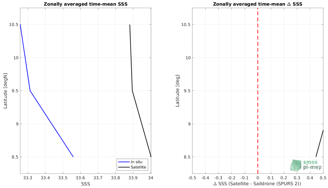
Figure 8: Left panel: Zonal mean SSS from SMOS SSS L3 v2 - 9-Days (BEC) satellite product (black) and from Sairdrone (SPURS 2) (blue). Right panel: Zonal mean of \Delta SSS (Satellite - Sairdrone (SPURS 2)) for all the collected Pi-MEP match-up pairs estimated over the full satellite product period.
