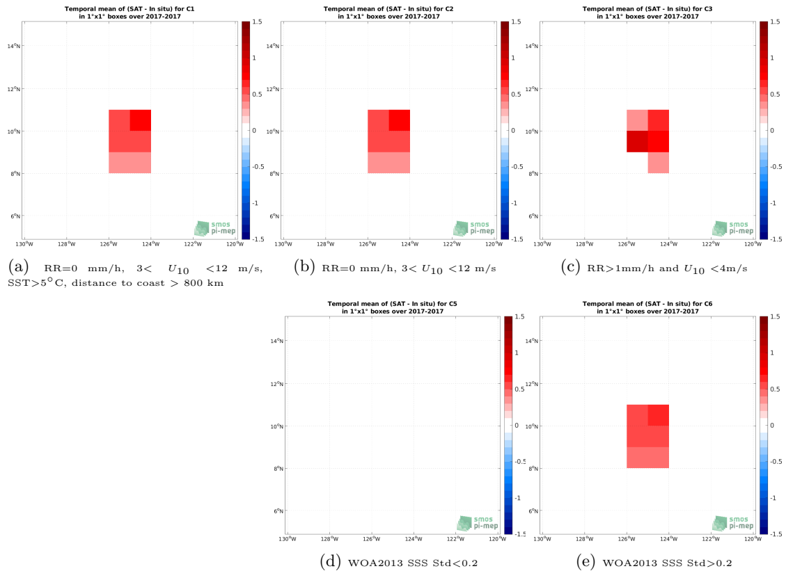
Figure 12: Temporal mean gridded over spatial boxes of size 1^\circ \times 1^\circ of \Delta SSS (SMOS SSS L3 v2 - 9-Days (BEC) - Saildrone (SPURS 2)) for 5 different subdatasets corresponding to:RR=0 mm/h, 3 < U_{10} < 12 m/s, SST >5^\circ C, distance to coast > 800 km (a), RR=0 mm/h, 3 < U_{10} < 12 m/s (b), RR >1 mm/h and U_{10} < 4 m/s (c), WOA2013 SSS Std <0.2 (d), WOA2013 SSS Std >0.2 (e).
