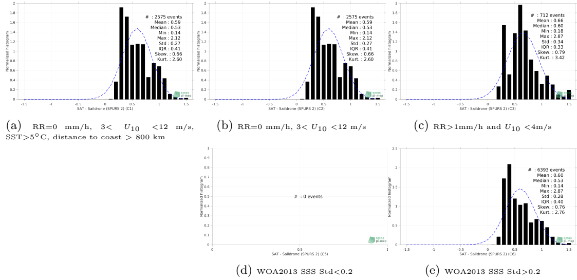
Figure 13: Normalized histogram of \Delta SSS (SMOS SSS L3 v2 - 9-Days (BEC) - Sairdroné (SPURS 2)) for 5 different subdatasets corresponding to: RR=0 mm/h, 3 < U_{10} < 12 m/s, SST > 5°C, distance to coast > 800 km (a), RR=0 mm/h, 3 < U_{10} < 12 m/s (b), RR > 1mm/h and U_{10} < 4 m/s (c), WOA2013 SSS Std < 0.2 (d), WOA2013 SSS Std > 0.2 (e).
