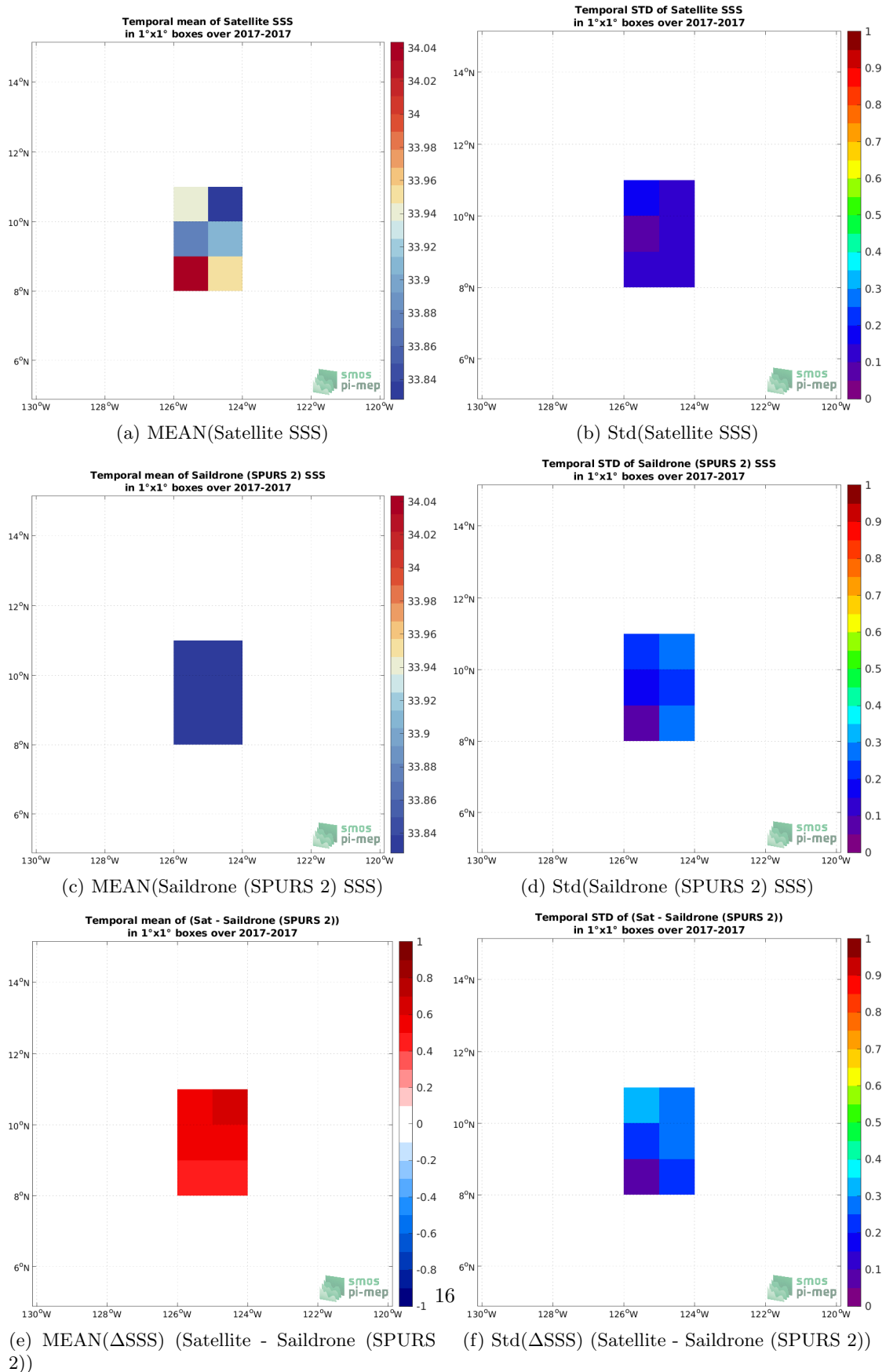
Figure 6: Temporal mean (left) and Std (right) of SSS from SMOS SSS L3 v2 - 9-Days (BEC) (top), Saildrone (SPURS 2) (middle), and of \Delta SSS (Satellite - Saildrone (SPURS 2)). Only match-up pairs are used to generate these maps.
