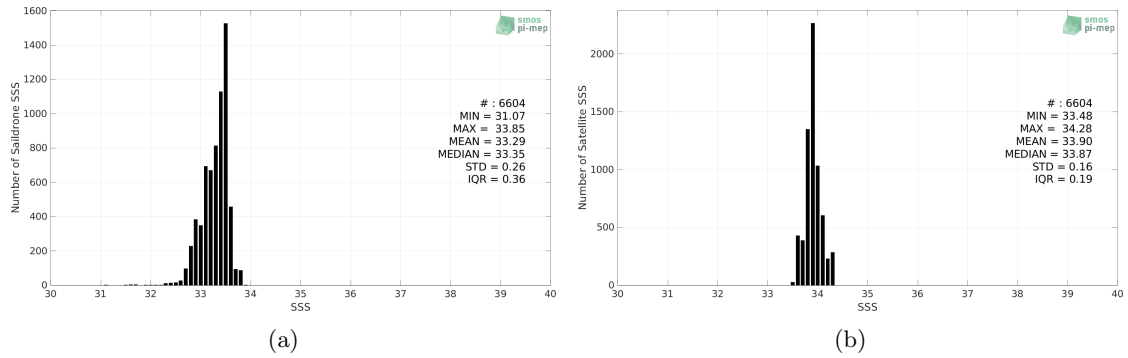
Figure 2: Histograms of SSS from Sairdrone (a) and SMOS SSS L3 v2 - 9-Days (BEC) (b) considering all match-up pairs per bins of 0.1 over the SPURS 2 Pi-MEP region and for the full satellite product period.
