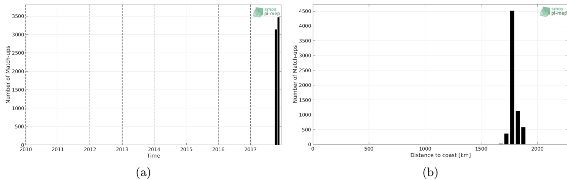
Figure 1: Number of match-ups between Saifdrone and SMOS SSS L3 v2 - 9-Days (BEC) SSS as a function of time (a) and as function of the distance to coast (b) over the SPURS 2 Pi-MEP region and for the full satellite product period.
