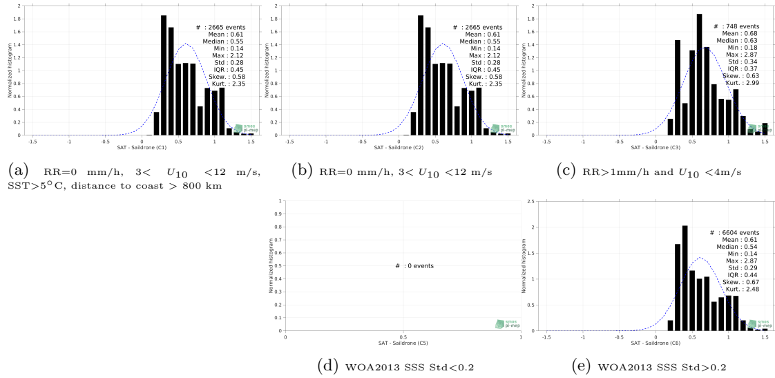
Figure 12: Normalized histogram of \Delta SSS (SMOS SSS L3 v2 - 9-Days (BEC) - Saildrone) for 5 different subdatasets corresponding to: RR=0 mm/h, 3 < U_{10} < 12 m/s, SST>5°C, distance to coast > 800 km (a), RR=0 mm/h, 3 < U_{10} < 12 m/s (b), RR>1mm/h and U_{10} < 4 m/s (c), WOA2013 SSS Std<0.2 (d), WOA2013 SSS Std>0.2 (e).
