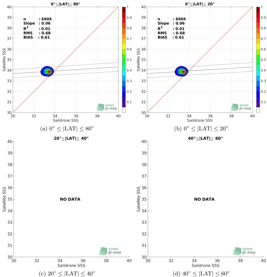
Figure 8: Contour maps of the concentration of SMOS SSS L3 v2 - 9-Days (BEC) SSS (y-axis) versus Saildrone SSS (x-axis) at match-up pairs for different latitude bands. For each plot, the red line shows x=y . The black thin and dashed lines indicate a linear fit through the data cloud and the \pm 95\% confidence levels, respectively. The number match-up pairs n , the slope and R^2 coefficient of the linear fit, the root mean square (RMS) and the mean bias between satellite and in situ data are indicated for each latitude band in each plots.
