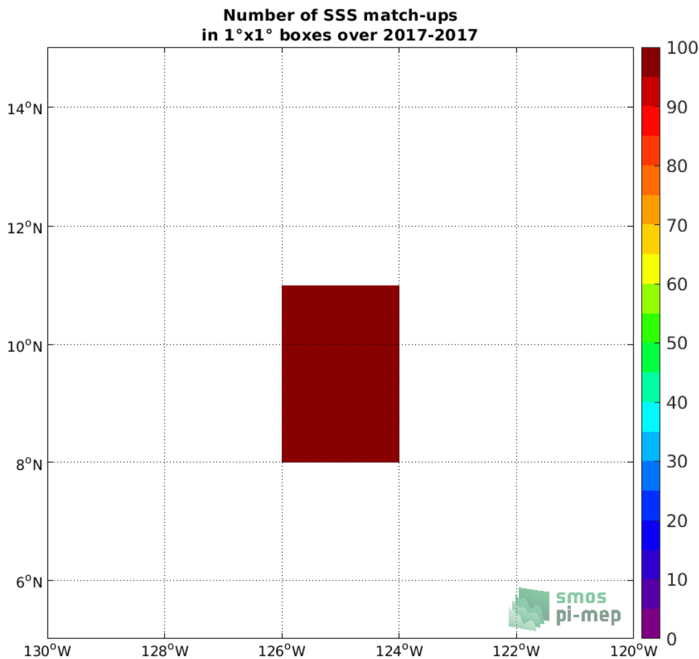
Figure 3: Number of SSS match-ups between Saildrone SSS and the SMOS SSS L3 v2 - 9-Days (BEC) SSS product for the SPURS 2 Pi-MEP region over 1°×1° boxes and for the full satellite product period.
