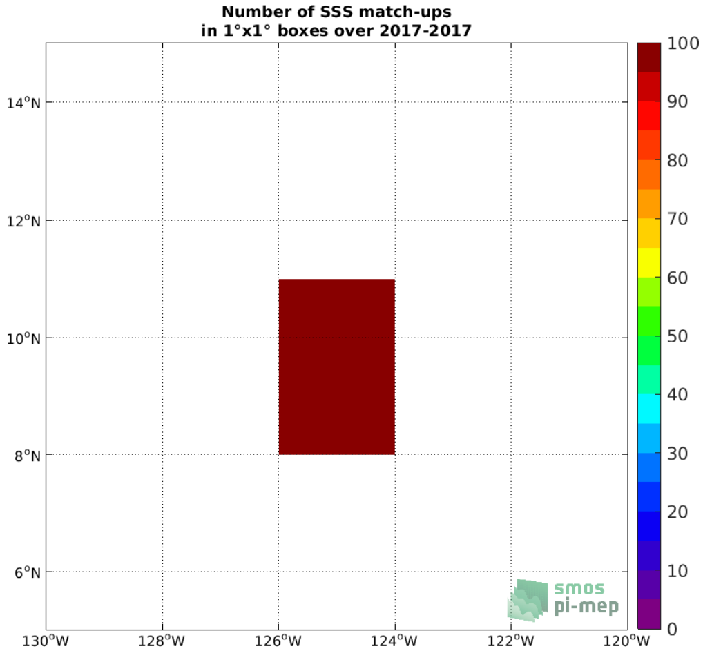
Figure 4: Number of SSS match-ups between Sairdron SSS and the SMOS SSS L3 v2 - 9-Days (BEC) SSS product for the SPURS 2 Pi-MEP region over 1°x1° boxes and for the full satellite product period.
