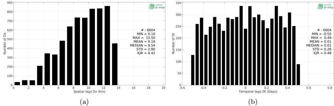
Figure 5: Histograms of the spatial (a) and temporal (b) lags between the time of the Saildrone measurements and the date of the corresponding SMOS SSS L3 v2 - 9-Days (BEC) SSS product.
