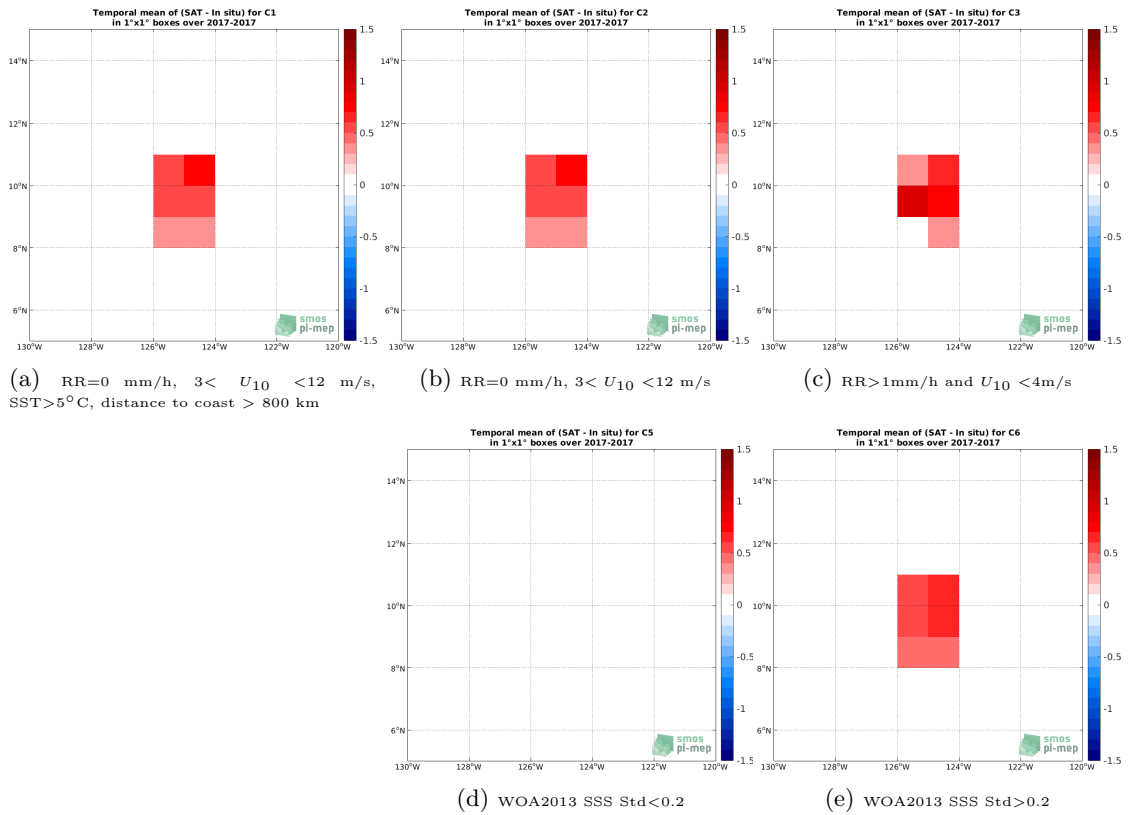
Figure 12: Temporal mean gridded over spatial boxes of size 1°x1° of \Delta SSS (SMOS SSS L3 v2 - 9-Days (BEC) - Saldrone) for 5 different subdatasets corresponding to:RR=0 mm/h, 3 < U_{10} < 12 m/s, SST>5°C, distance to coast > 800 km (a), RR=0 mm/h, 3 < U_{10} < 12 m/s (b), RR>1mm/h and U_{10} < 4 m/s (c), WOA2013 SSS Std<0.2 (d), WOA2013 SSS Std>0.2 (e).
