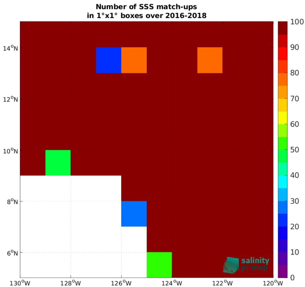
Figure 4: Number of SSS match-ups between Surface drifters SSS and the SMOS SSS L3 v2 - 9-Days (BEC) SSS product for the SPURS 2 Pi-MEP region over 1°x1° boxes and for the full satellite product period.
