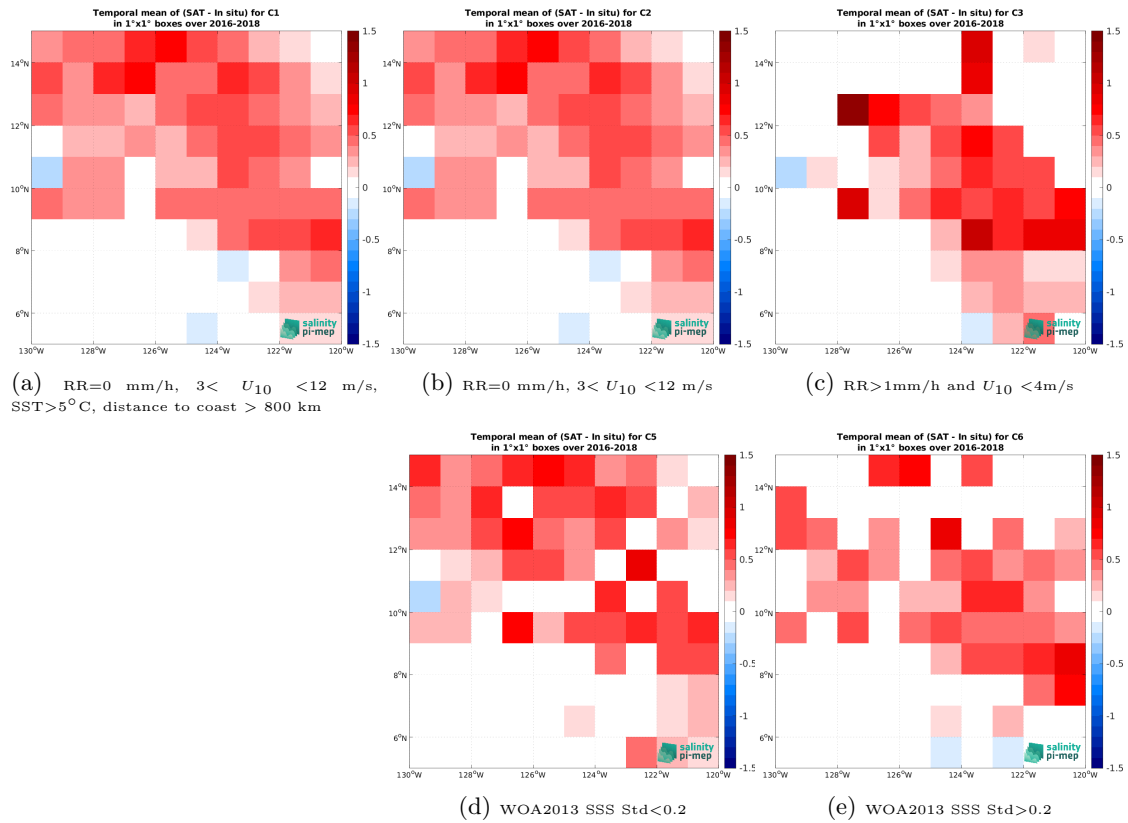
Figure 13: Temporal mean gridded over spatial boxes of size 1^\circ \times 1^\circ of \Delta\text{SSS} (SMOS SSS L3 v2 - 9-Days (BEC) - Surface drifters) for 5 different subdatasets corresponding to:RR=0 mm/h, 3 < U_{10} < 12 m/s, SST >5^\circ\text{C} , distance to coast > 800 km (a), RR=0 mm/h, 3 < U_{10} < 12 m/s (b), RR >1 mm/h and U_{10} < 4 m/s (c), WOA2013 SSS Std <0.2 (d), WOA2013 SSS Std >0.2 (e).
