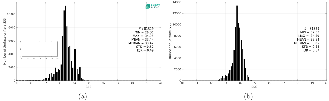
Figure 3: Histograms of SSS from Surface drifters (a) and SMOS SSS L3 v2 - 9-Days (BEC) (b) considering all match-up pairs per bins of 0.1 over the SPURS 2 Pi-MEP region and for the full satellite product period.
