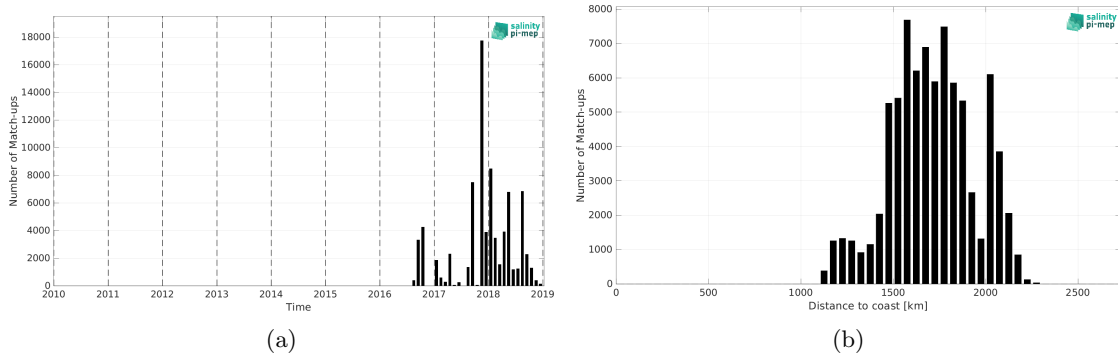
Figure 2: Number of match-ups between Surface drifters and SMOS SSS L3 v2 - 9-Days (BEC) SSS as a function of time (a) and as function of the distance to coast (b) over the SPURS 2 Pi-MEP region and for the full satellite product period.
