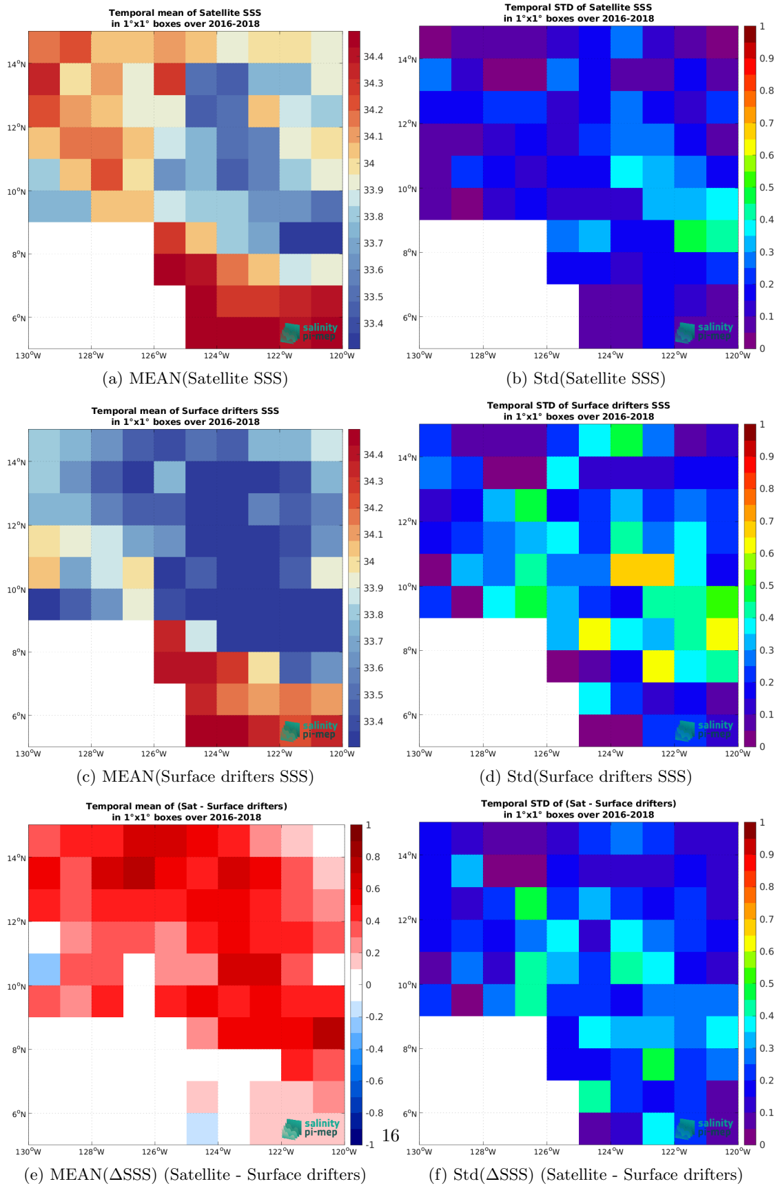
Figure 6: Temporal mean (left) and Std (right) of SSS from SMOS SSS L3 v2 - 9-Days (BEC) (top), Surface drifters (middle), and of \Delta SSS (Satellite - Surface drifters). Only match-up pairs are used to generate these maps.
