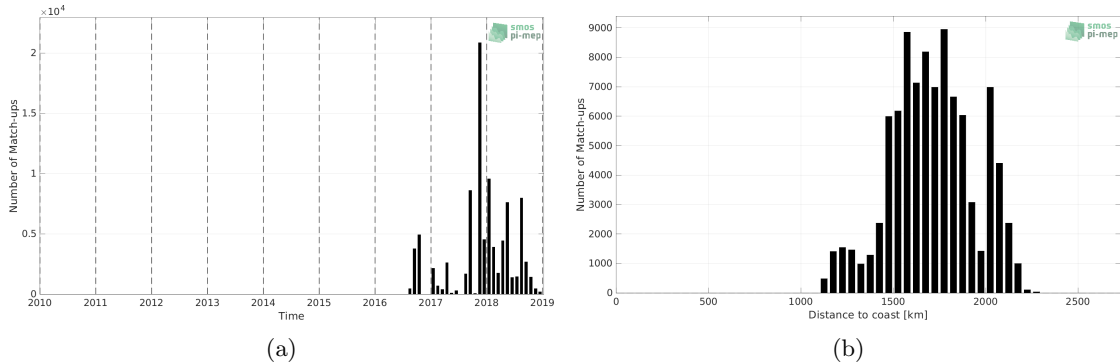
Figure 1: Number of match-ups between Surface drifters and SMOS SSS L3 v2 - 9-Days (BEC) SSS as a function of time (a) and as function of the distance to coast (b) over the SPURS 2 Pi-MEP region and for the full satellite product period.
