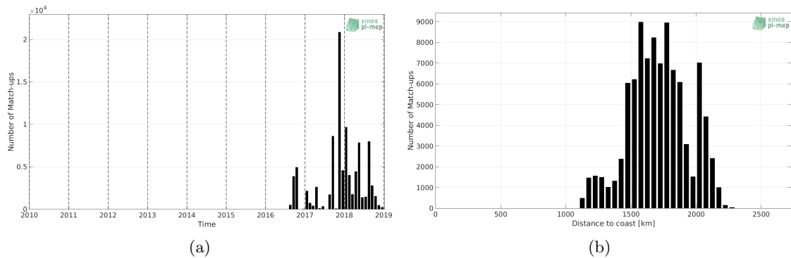
Figure 1: Number of match-ups between Surface drifters and SMOS L3 v2 - 9-Days (BEC) SSS as a function of time (a) and as function of the distance to coast (b) over the SPURS 2 Pi-MEP region and for the full satellite product period.
