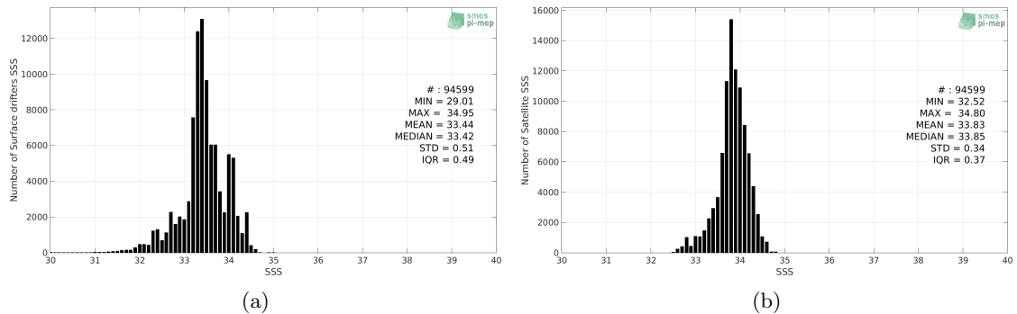
Figure 2: Histograms of SSS from Surface drifters (a) and SMOS L3 v2 - 9-Days (BEC) (b) considering all match-up pairs per bins of 0.1 over the SPURS 2 Pi-MEP region and for the full satellite product period.
