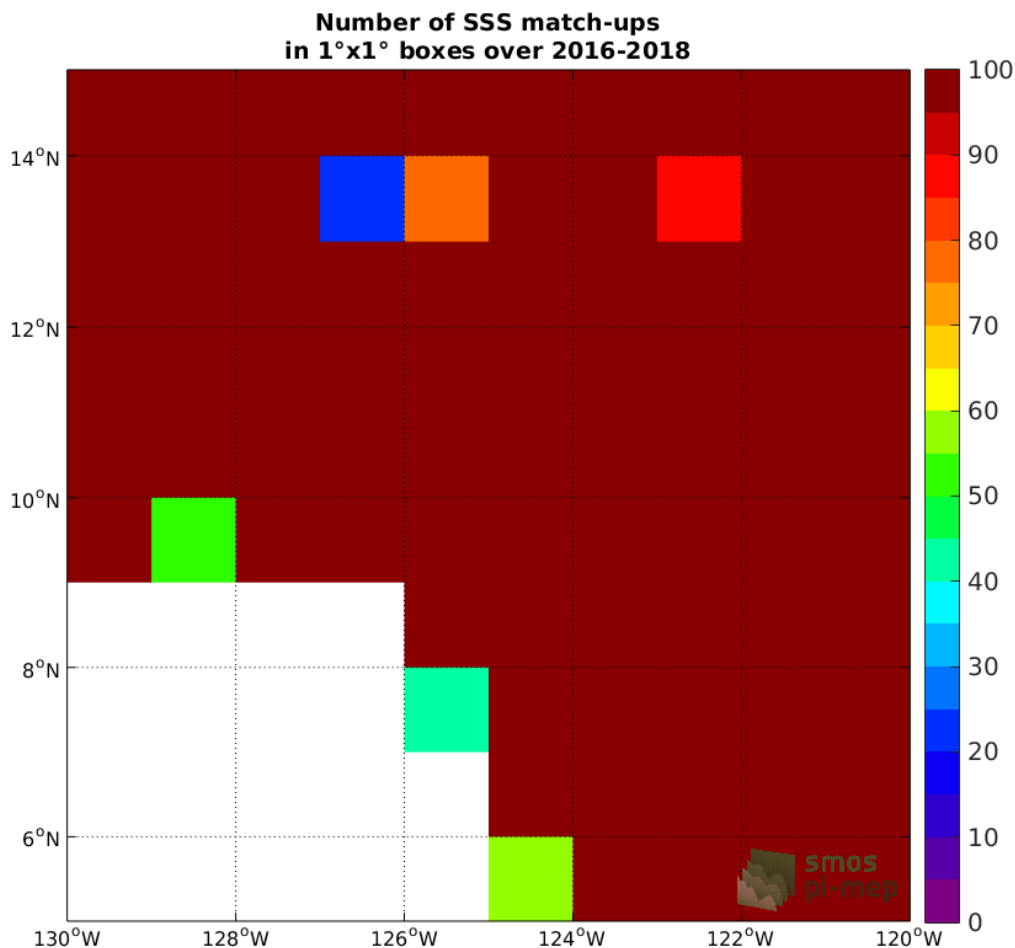
Figure 3: Number of SSS match-ups between Surface drifters SSS and the SMOS L3 v2 - 9-Days (BEC) SSS product for the SPURS 2 Pi-MEP region over 1°x1° boxes and for the full satellite product period.
