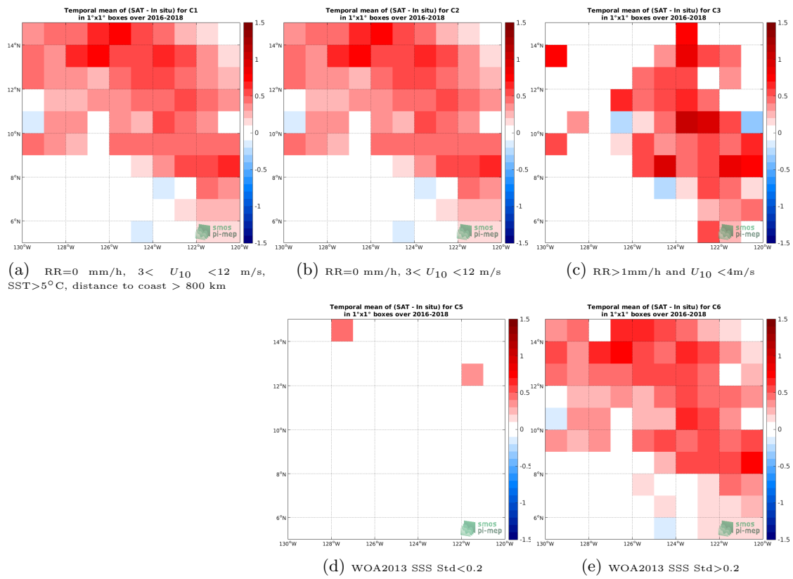
Figure 11: Temporal mean gridded over spatial boxes of size 1^\circ \times 1^\circ of \Delta\text{SSS} (SMOS L3 v2 - 9-Days (BEC) - Surface drifters) for 5 different subdatasets corresponding to:RR=0 mm/h, 3 < U_{10} < 12 m/s, SST >5^\circ\text{C} , distance to coast > 800 km (a), RR=0 mm/h, 3 < U_{10} < 12 m/s (b), RR >1 mm/h and U_{10} < 4 m/s (c), WOA2013 SSS Std <0.2 (d), WOA2013 SSS Std >0.2 (e).
