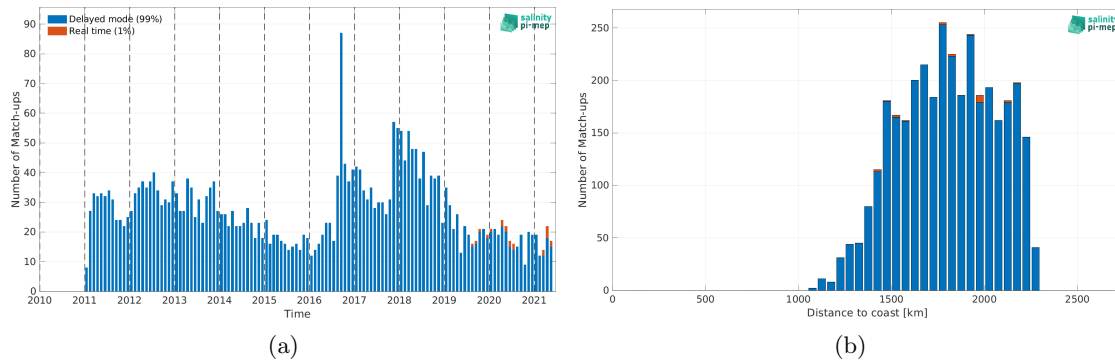
Figure 2: Number of match-ups between Argo and SMOS SSS L3 v2 - 9-Days (BEC) SSS as a function of time (a) and as function of the distance to coast (b) over the SPURS 2 Pi-MEP region and for the full satellite product period.
