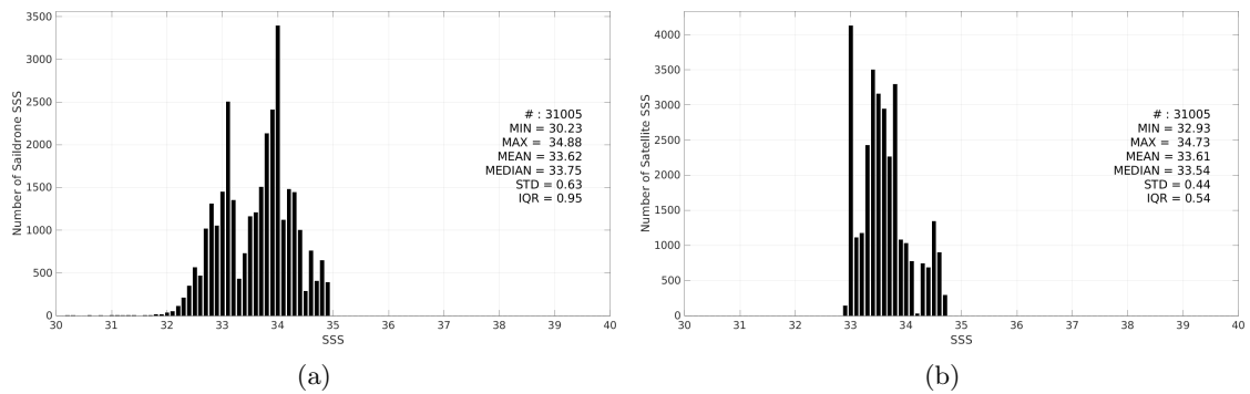
Figure 3: Histograms of SSS from Saildrone (a) and SMAP SSS L3 v6 - Monthly (RSS) (b) considering all match-up pairs per bins of 0.1 over the SPURS 2 Pi-MEP region and for the full satellite product period.
