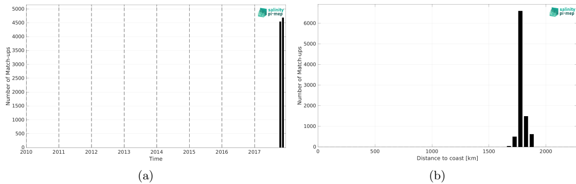
Figure 2: Number of match-ups between Saildrone (SPURS 2) and SMAP SSS L3 v6 - Monthly (RSS) SSS as a function of time (a) and as function of the distance to coast (b) over the SPURS 2 Pi-MEP region and for the full satellite product period.
