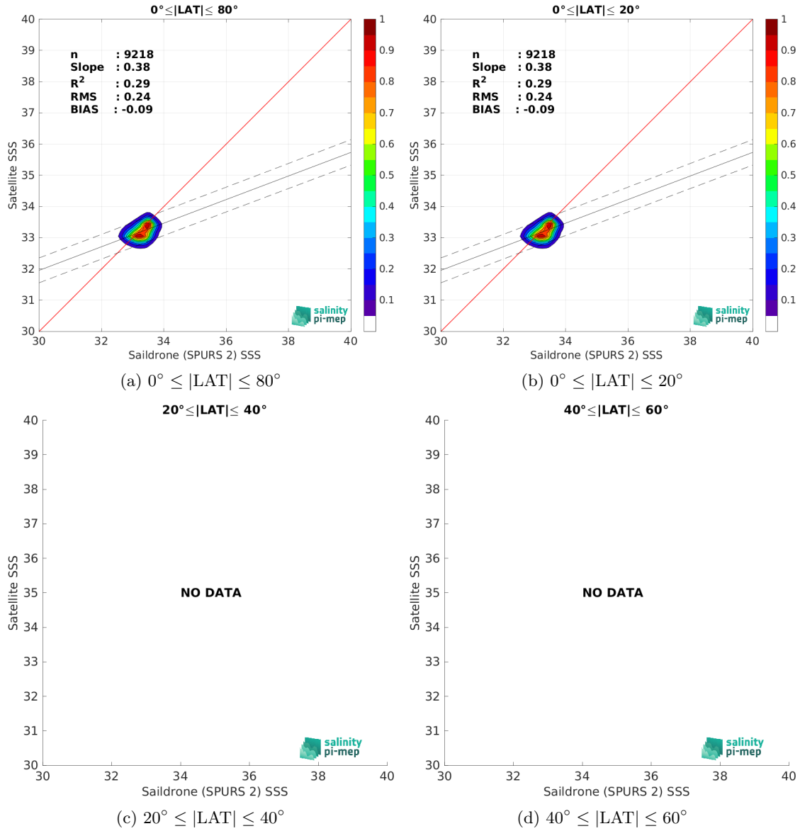
Figure 10: Contour maps of the concentration of SMAP SSS L3 v6 - Monthly (RSS) SSS (y-axis) versus Saildrone (SPURS 2) SSS (x-axis) at match-up pairs for different latitude bands. For each plot, the red line shows x=y . The black thin and dashed lines indicate a linear fit through the data cloud and the \pm 95\% confidence levels, respectively. The number match-up pairs n , the slope and R^2 coefficient of the linear fit, the root mean square (RMS) and the mean bias between satellite and in situ data are indicated for each latitude band in each plots.
