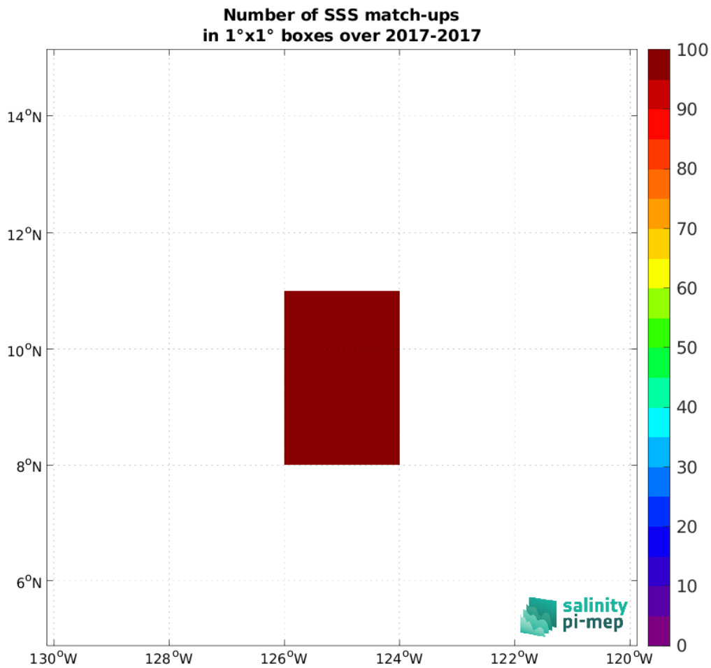
Figure 5: Number of SSS match-ups between SAILDRONE (SPURS 2) SSS and the SMAP SSS L3 v6 - Monthly (RSS) SSS product for the SPURS 2 Pi-MEP region over 1°×1° boxes and for the full satellite product period.
