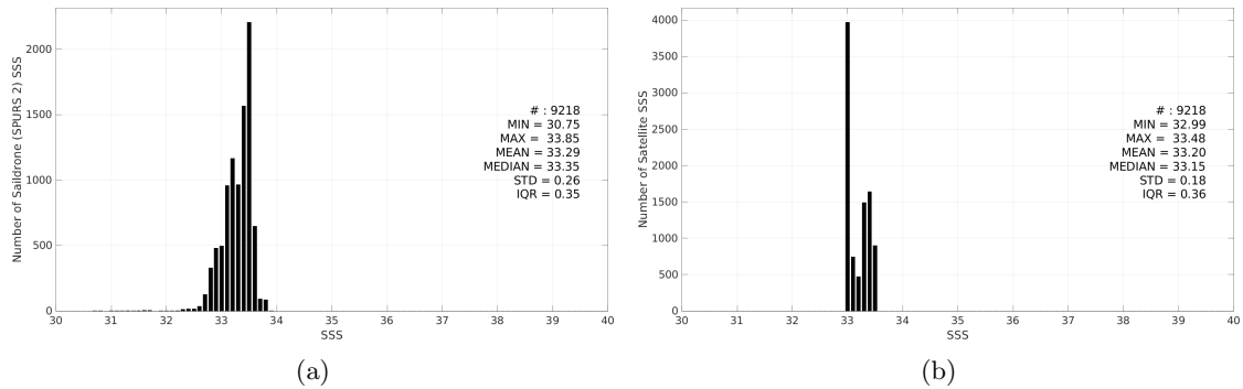
Figure 3: Histograms of SSS from Saildrone (SPURS 2) (a) and SMAP SSS L3 v6 - Monthly (RSS) (b) considering all match-up pairs per bins of 0.1 over the SPURS 2 Pi-MEP region and for the full satellite product period.
