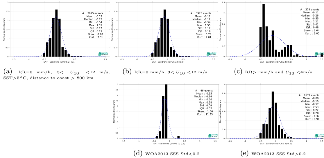
Figure 15: Normalized histogram of \Delta SSS (SMAP SSS L3 v6 - Monthly (RSS) - Sallidrone (SPURS 2)) for 5 different subdatasets corresponding to: RR=0 mm/h, 3 < U_{10} < 12 m/s, SST > 5°C, distance to coast > 800 km (a), RR=0 mm/h, 3 < U_{10} < 12 m/s (b), RR > 1mm/h and U_{10} < 4 m/s (c), WOA2013 SSS Std < 0.2 (d), WOA2013 SSS Std > 0.2 (e).
