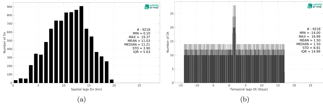
Figure 6: Histograms of the spatial (a) and temporal (b) lags between the location/time of the Saildrone (SPURS 2) measurement and the date of the corresponding SMAP SSS L3 v6 - Monthly (RSS) SSS pixel.
