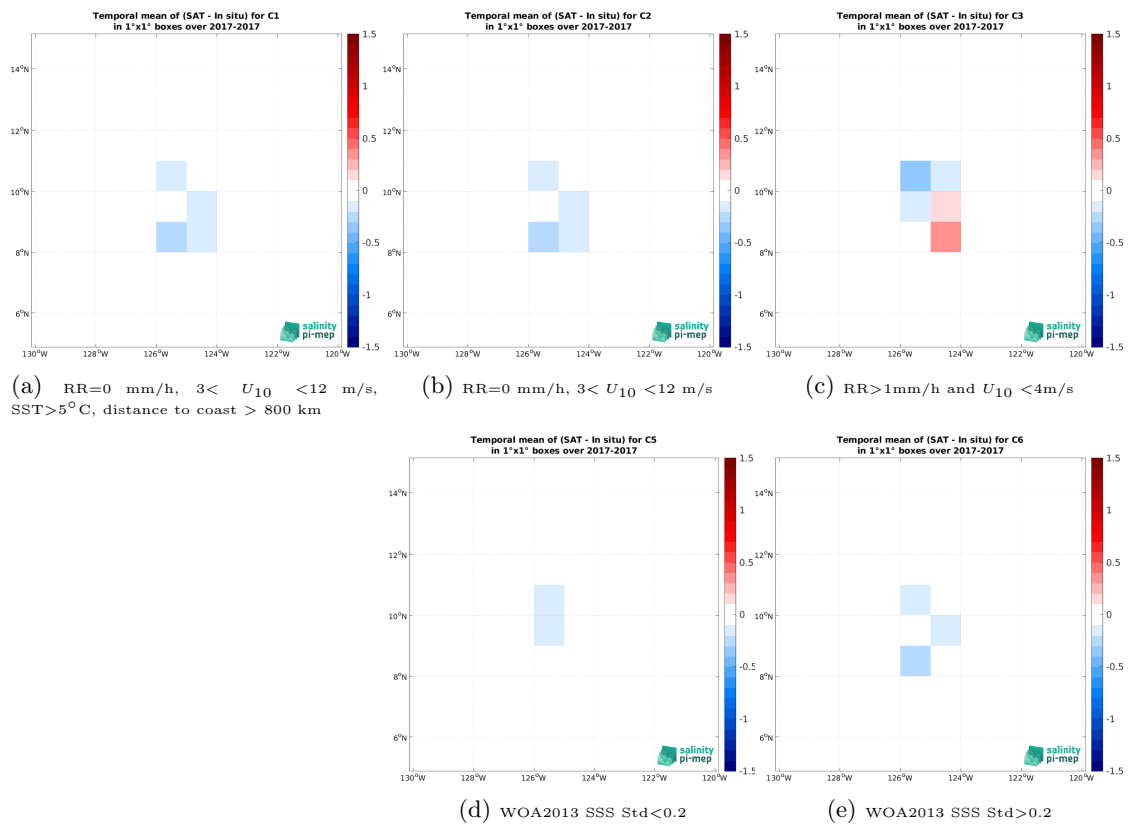
Figure 14: Temporal mean gridded over spatial boxes of size 1^\circ \times 1^\circ of \Delta SSS (SMAP SSS L3 v6 - Monthly (RSS) - Saildrone (SPURS 2)) for 5 different subdatasets corresponding to:RR=0 mm/h, 3 < U_{10} < 12 m/s, SST >5^\circ C, distance to coast > 800 km (a), RR=0 mm/h, 3 < U_{10} < 12 m/s (b), RR >1 mm/h and U_{10} < 4 m/s (c), WOA2013 SSS Std <0.2 (d), WOA2013 SSS Std >0.2 (e).
