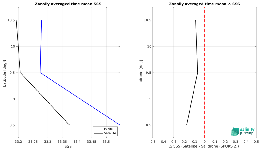
Figure 9: Left panel: Zonal mean SSS from SMAP SSS L3 v6 - Monthly (RSS) satellite product (black) and from Sairdrone (SPURS 2) (blue). Right panel: Zonal mean of \Delta SSS (Satellite - Sairdrone (SPURS 2)) for all the collected Pi-MEP match-up pairs estimated over the full satellite product period.
