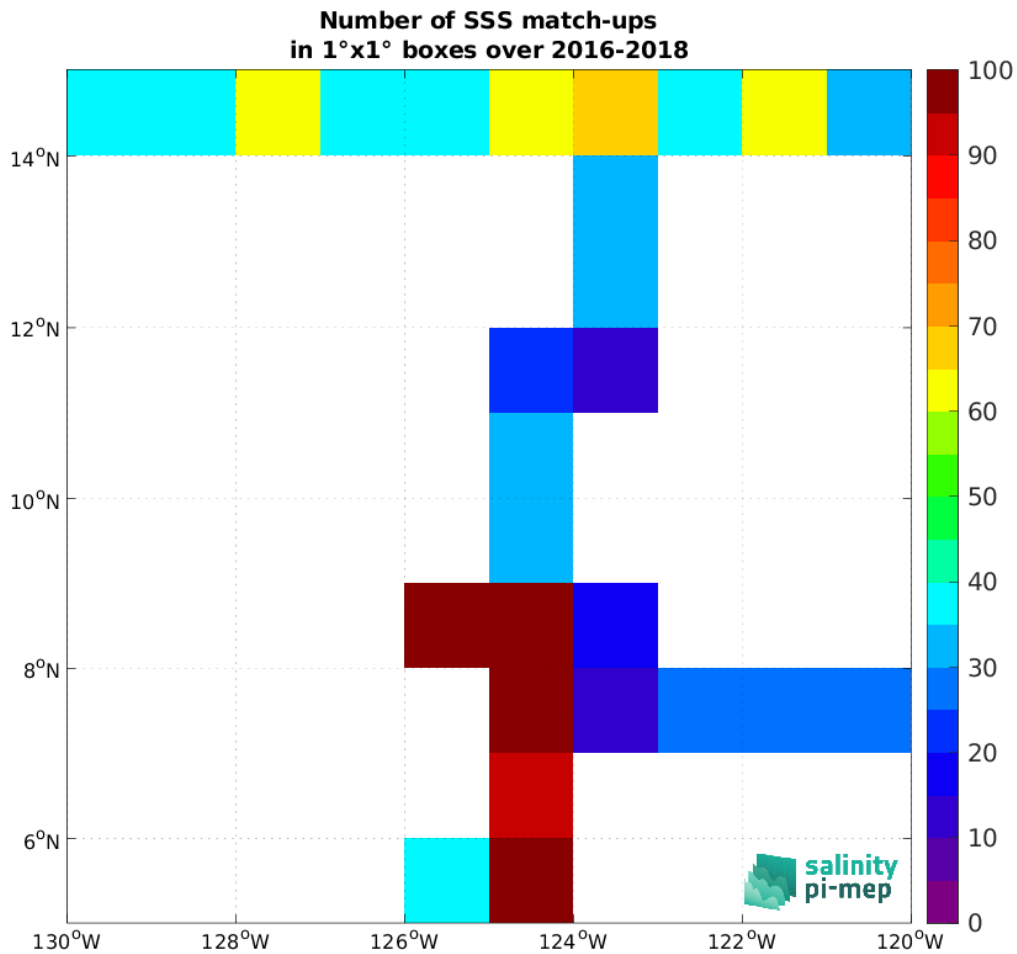
Figure 5: Number of SSS match-ups between TSG (SAMOS) SSS and the SMAP SSS L3 v5.3 - 8-Day running (RSS) SSS product for the SPURS 2 Pi-MEP region over 1°x1° boxes and for the full satellite product period.
