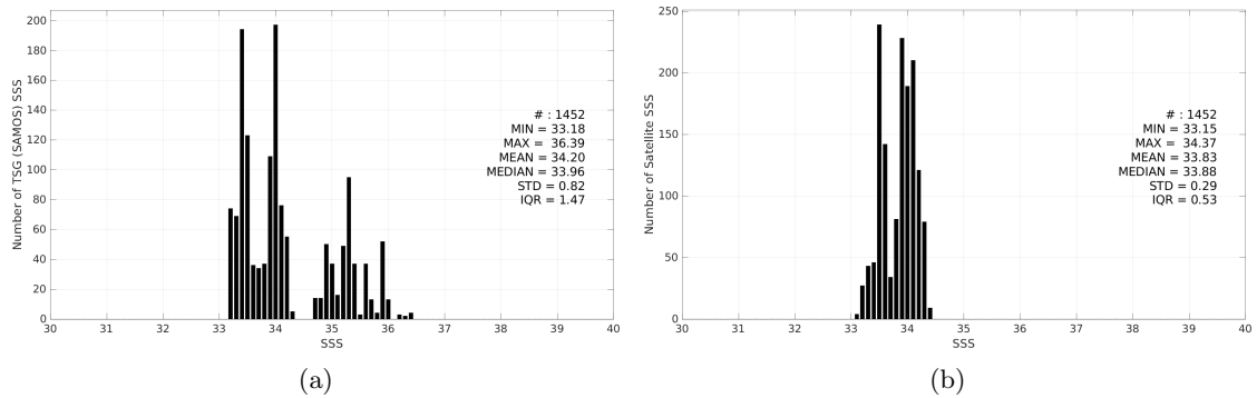
Figure 3: Histograms of SSS from TSG (SAMOS) (a) and SMAP SSS L3 v5.3 - 8-Day running (RSS) (b) considering all match-up pairs per bins of 0.1 over the SPURS 2 Pi-MEP region and for the full satellite product period.
