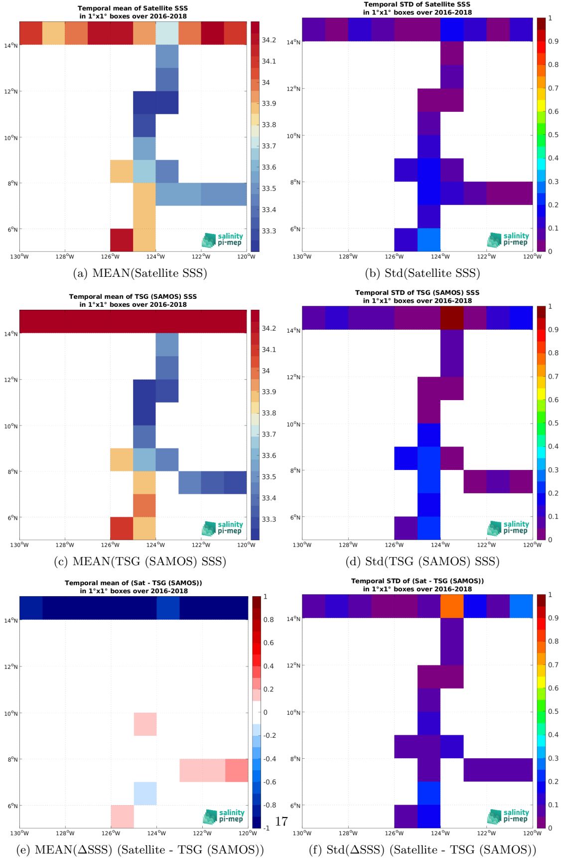
Figure 7: Temporal mean (left) and Std (right) of SSS from SMAP SSS L3 v5.3 - 8-Day running (RSS) (top), TSG (SAMOS) (middle), and of \Delta SSS (Satellite - TSG (SAMOS)). Only match-up pairs are used to generate these maps.
