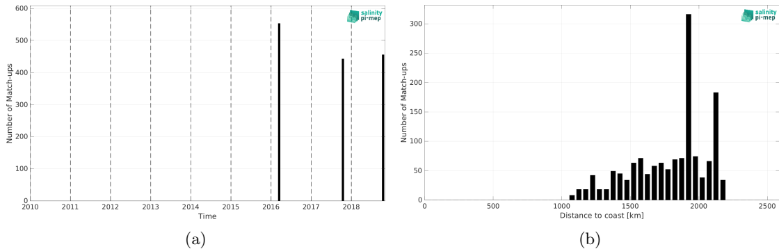
Figure 2: Number of match-ups between TSG (SAMOS) and SMAP SSS L3 v5.3 - 8-Day running (RSS) SSS as a function of time (a) and as function of the distance to coast (b) over the SPURS 2 Pi-MEP region and for the full satellite product period.
