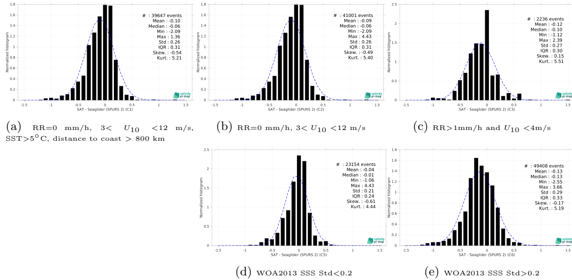
Figure 15: Normalized histogram of \Delta SSS (SMAP SSS L3 v5.3 - 8-Day running (RSS) - Seaglider (SPURS 2)) for 5 different subdatasets corresponding to: RR=0 mm/h, 3 < U_{10} < 12 m/s, SST>5°C, distance to coast > 800 km (a), RR=0 mm/h, 3 < U_{10} < 12 m/s (b), RR>1mm/h and U_{10} < 4 m/s (c), WOA2013 SSS Std<0.2 (d), WOA2013 SSS Std>0.2 (e).
