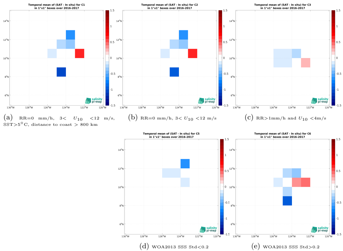
Figure 14: Temporal mean gridded over spatial boxes of size 1^\circ \times 1^\circ of \Delta SSS (SMAP SSS L3 v5.3 - 8-Day running (RSS) - Seaglider (SPURS 2)) for 5 different subdatasets corresponding to:RR=0 mm/h, 3 < U_{10} < 12 m/s, SST>5°C, distance to coast > 800 km (a), RR=0 mm/h, 3 < U_{10} < 12 m/s (b), RR>1mm/h and U_{10} < 4 m/s (c), WOA2013 SSS Std<0.2 (d), WOA2013 SSS Std>0.2 (e).
