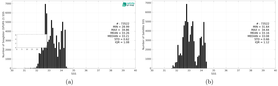
Figure 3: Histograms of SSS from Seaglider (SPURS 2) (a) and SMAP SSS L3 v5.3 - 8-Day running (RSS) (b) considering all match-up pairs per bins of 0.1 over the SPURS 2 Pi-MEP region and for the full satellite product period.
