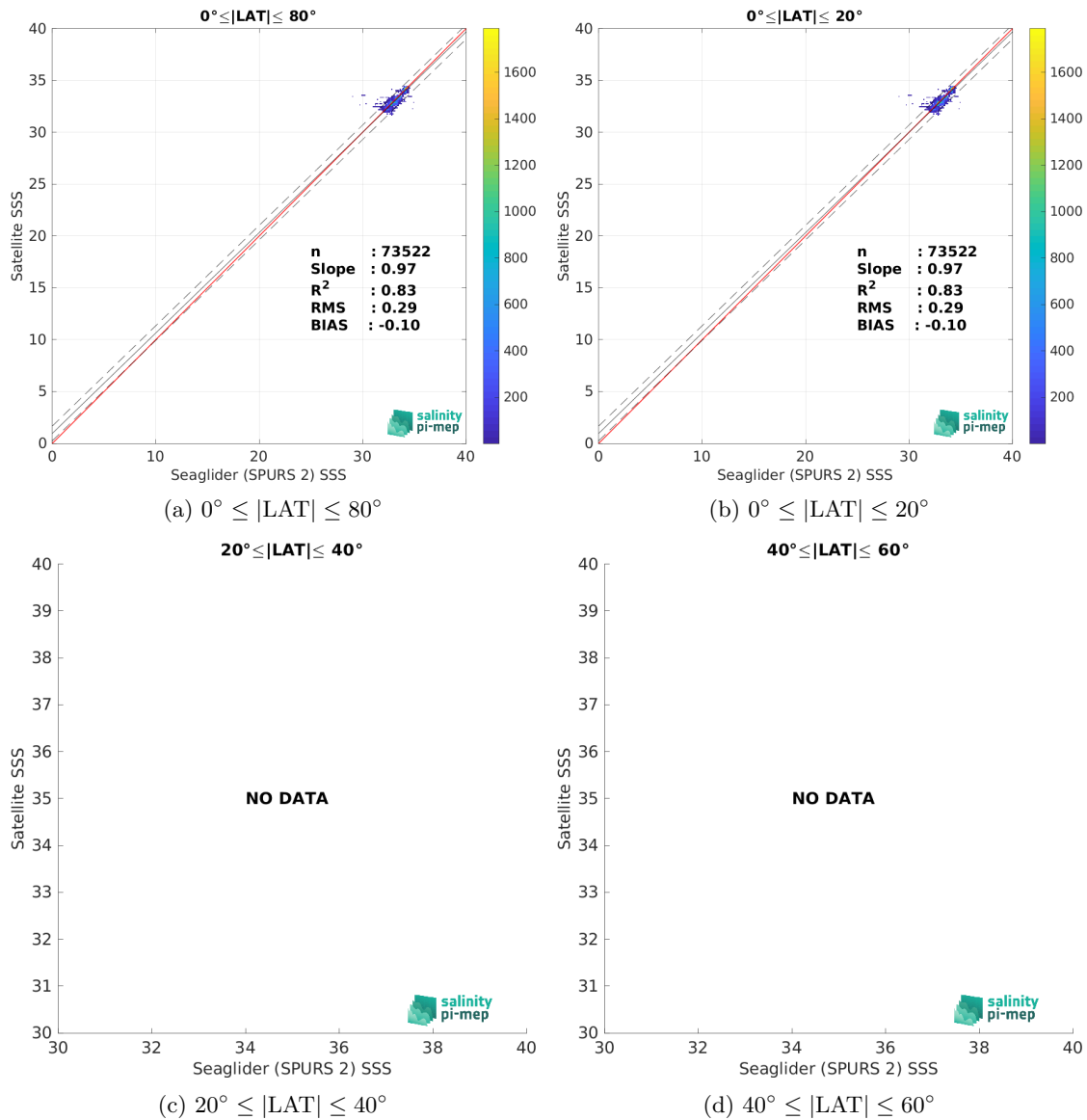
Figure 10: Contour maps of the concentration of SMAP SSS L3 v5.3 - 8-Day running (RSS) SSS (y-axis) versus Seaglider (SPURS 2) SSS (x-axis) at match-up pairs for different latitude bands. For each plot, the red line shows x=y . The black thin and dashed lines indicate a linear fit through the data cloud and the \pm 95\% confidence levels, respectively. The number match-up pairs n , the slope and R^2 coefficient of the linear fit, the root mean square (RMS) and the mean bias between satellite and in situ data are indicated for each latitude band in each plots.
