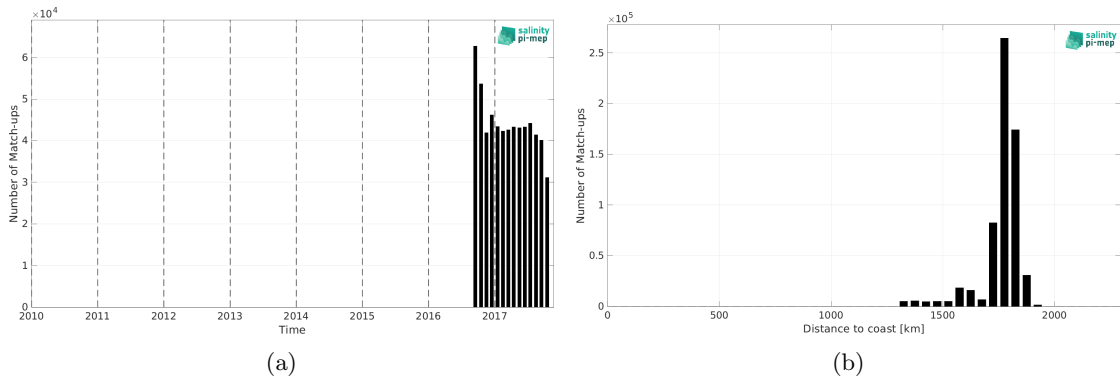
Figure 2: Number of match-ups between Waveglider (SPURS 2) and SMAP SSS L3 v5.3 - Monthly (RSS) SSS as a function of time (a) and as function of the distance to coast (b) over the SPURS 2 Pi-MEP region and for the full satellite product period.
