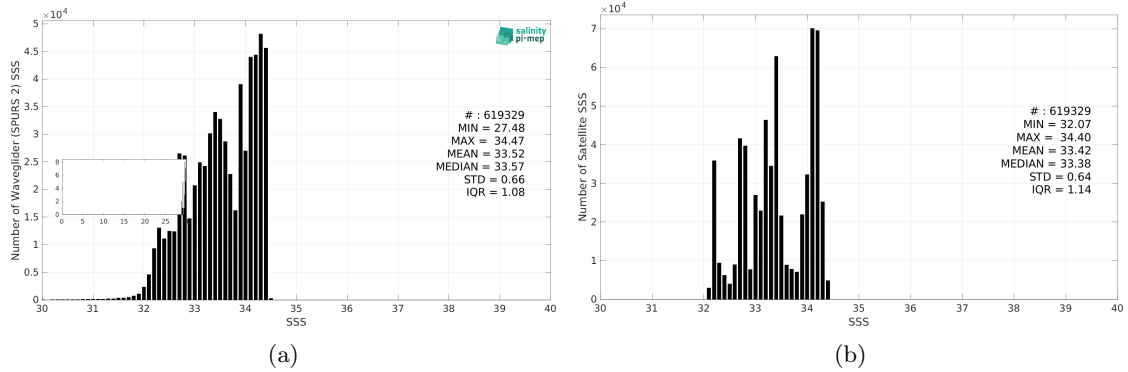
Figure 3: Histograms of SSS from Waveglider (SPURS 2) (a) and SMAP SSS L3 v5.3 - Monthly (RSS) (b) considering all match-up pairs per bins of 0.1 over the SPURS 2 Pi-MEP region and for the full satellite product period.
