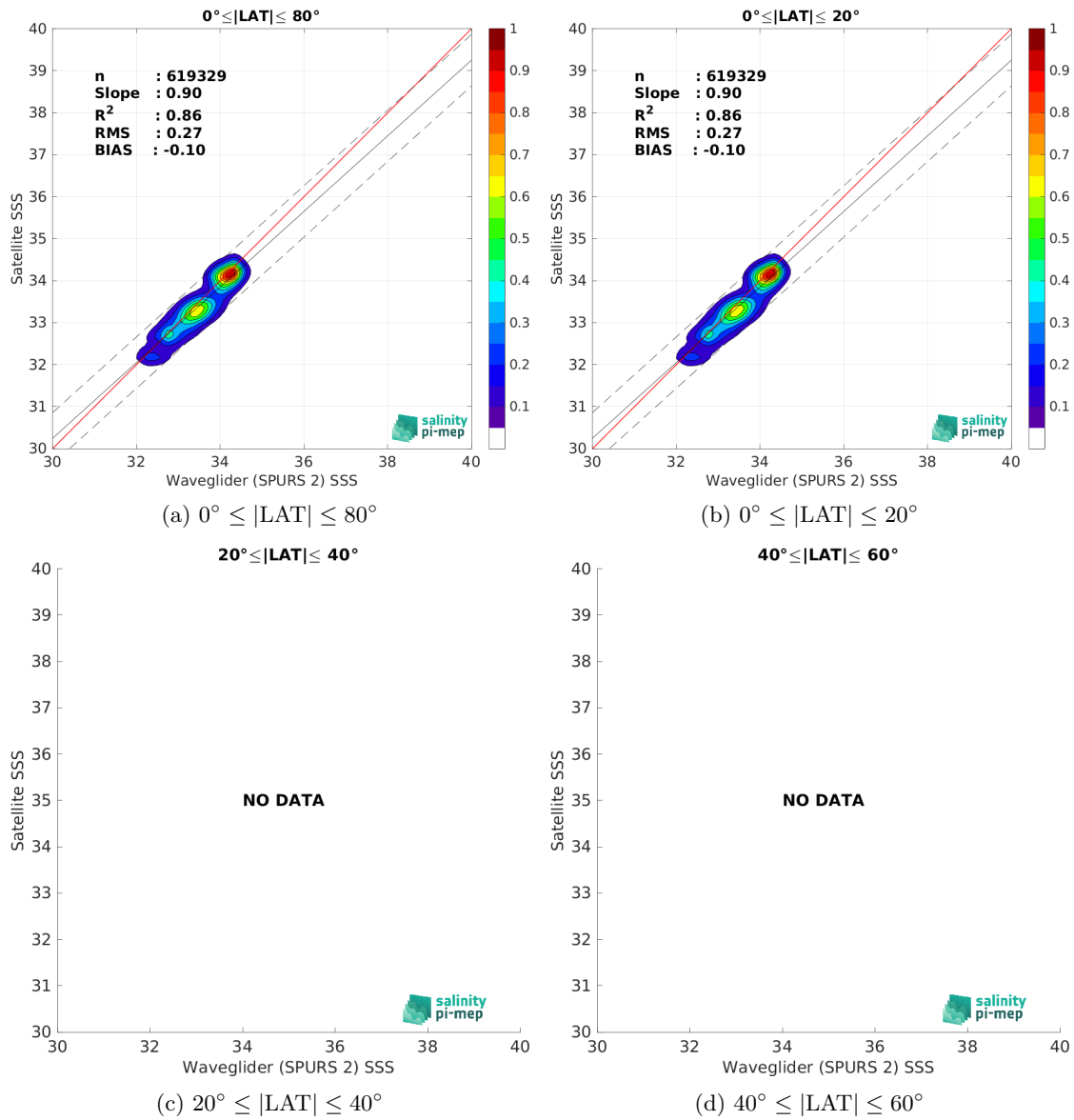
Figure 10: Contour maps of the concentration of SMAP SSS L3 v5.3 - Monthly (RSS) SSS (y-axis) versus Waveglider (SPURS 2) SSS (x-axis) at match-up pairs for different latitude bands. For each plot, the red line shows x=y . The black thin and dashed lines indicate a linear fit through the data cloud and the \pm 95\% confidence levels, respectively. The number match-up pairs n , the slope and R^2 coefficient of the linear fit, the root mean square (RMS) and the mean bias between satellite and in situ data are indicated for each latitude band in each plots.
