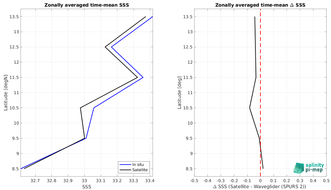
Figure 9: Left panel: Zonal mean SSS from SMAP SSS L3 v5.3 - Monthly (RSS) satellite product (black) and from Waveglider (SPURS 2) (blue). Right panel: Zonal mean of \Delta SSS (Satellite - Waveglider (SPURS 2)) for all the collected Pi-MEP match-up pairs estimated over the full satellite product period.
