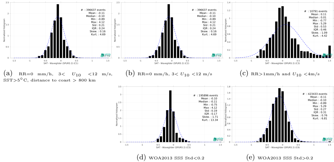
Figure 15: Normalized histogram of \Delta SSS (SMAP SSS L3 v5.3 - Monthly (RSS) - Waveglider (SPURS 2)) for 5 different subdatasets corresponding to: RR=0 mm/h, 3 < U_{10} < 12 m/s, SST > 5°C, distance to coast > 800 km (a), RR=0 mm/h, 3 < U_{10} < 12 m/s (b), RR > 1mm/h and U_{10} < 4 m/s (c), WOA2013 SSS Std < 0.2 (d), WOA2013 SSS Std > 0.2 (e).
