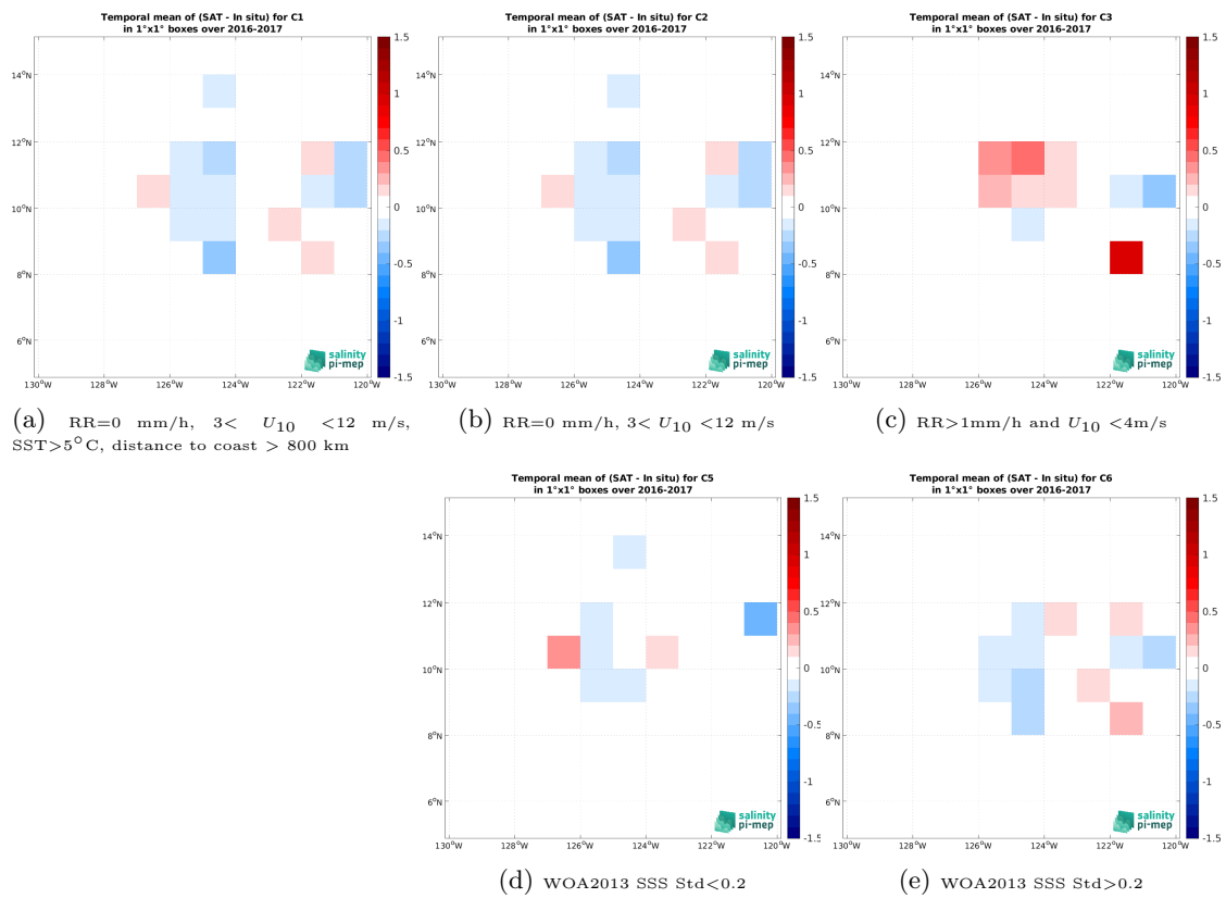
Figure 14: Temporal mean gridded over spatial boxes of size 1^\circ \times 1^\circ of \Delta\text{SSS} (SMAP SSS L3 v5.3 - Monthly (RSS) - Waveglider (SPURS 2)) for 5 different subdatasets corresponding to:RR=0 mm/h, 3 < U_{10} < 12 m/s, SST>5°C, distance to coast > 800 km (a), RR=0 mm/h, 3 < U_{10} < 12 m/s (b), RR>1mm/h and U_{10} < 4 m/s (c), WOA2013 SSS Std<0.2 (d), WOA2013 SSS Std>0.2 (e).
