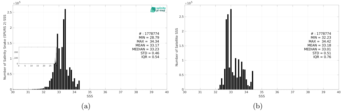
Figure 3: Histograms of SSS from Salinity Snake (SPURS 2) (a) and SMAP SSS L3 v5.3 - Monthly (RSS) (b) considering all match-up pairs per bins of 0.1 over the SPURS 2 Pi-MEP region and for the full satellite product period.
