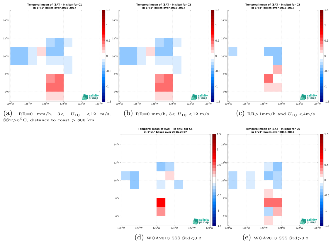
Figure 14: Temporal mean gridded over spatial boxes of size 1^\circ \times 1^\circ of \Delta\text{SSS} (SMAP SSS L3 v5.3 - Monthly (RSS) - Salinity Snake (SPURS 2)) for 5 different subdatasets corresponding to:RR=0 mm/h, 3 < U_{10} < 12 m/s, SST>5°C, distance to coast > 800 km (a), RR=0 mm/h, 3 < U_{10} < 12 m/s (b), RR>1mm/h and U_{10} < 4 m/s (c), WOA2013 SSS Std<0.2 (d), WOA2013 SSS Std>0.2 (e).
