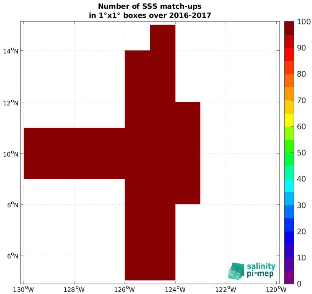
Figure 5: Number of SSS match-ups between Salinity Snake (SPURS 2) SSS and the SMAP SSS L3 v5.3 - Monthly (RSS) SSS product for the SPURS 2 Pi-MEP region over 1^\circ \times 1^\circ boxes and for the full satellite product period.
