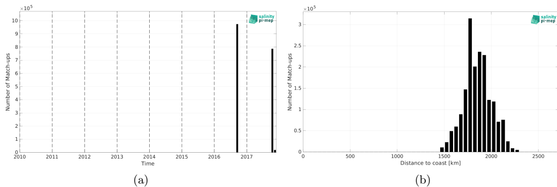
Figure 2: Number of match-ups between Salinity Snake (SPURS 2) and SMAP SSS L3 v5.3 - Monthly (RSS) SSS as a function of time (a) and as function of the distance to coast (b) over the SPURS 2 Pi-MEP region and for the full satellite product period.
