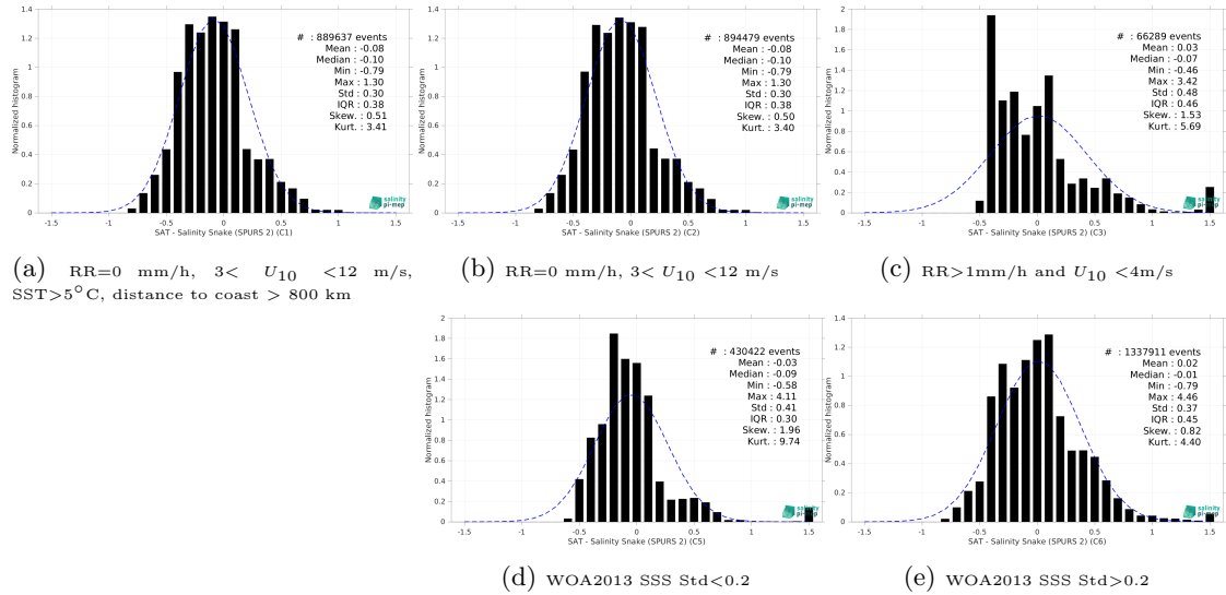
Figure 15: Normalized histogram of \Delta\text{SSS} (SMAP SSS L3 v5.3 - Monthly (RSS) - Salinity Snake (SPURS 2)) for 5 different subdatasets corresponding to: RR=0 mm/h, 3 < U_{10} < 12 m/s, SST>5°C, distance to coast > 800 km (a), RR=0 mm/h, 3 < U_{10} < 12 m/s (b), RR>1mm/h and U_{10} < 4 m/s (c), WOA2013 SSS Std<0.2 (d), WOA2013 SSS Std>0.2 (e).
