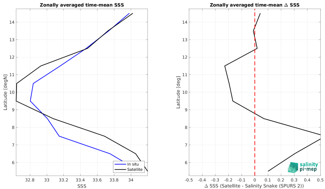
Figure 9: Left panel: Zonal mean SSS from SMAP SSS L3 v5.3 - Monthly (RSS) satellite product (black) and from Salinity Snake (SPURS 2) (blue). Right panel: Zonal mean of \Delta SSS (Satellite - Salinity Snake (SPURS 2)) for all the collected Pi-MEP match-up pairs estimated over the full satellite product period.
