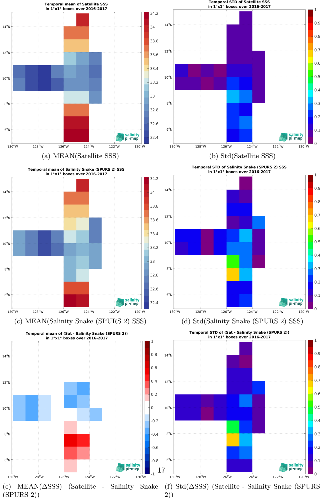
Figure 7: Temporal mean (left) and Std (right) of SSS from SMAP SSS L3 v5.3 - Monthly (RSS) (top), Salinity Snake (SPURS 2) (middle), and of \Delta SSS (Satellite - Salinity Snake (SPURS 2)). Only match-up pairs are used to generate these maps.
