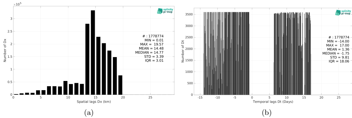
Figure 6: Histograms of the spatial (a) and temporal (b) lags between the location/time of the Salinity Snake (SPURS 2) measurement and the date of the corresponding SMAP SSS L3 v5.3 - Monthly (RSS) SSS pixel.
