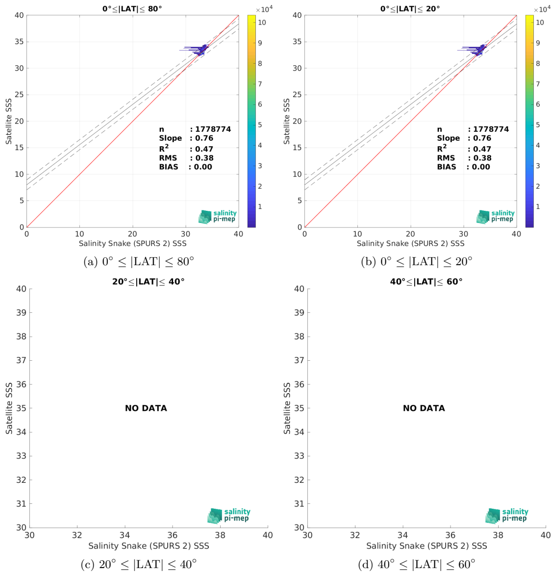
Figure 10: Contour maps of the concentration of SMAP SSS L3 v5.3 - Monthly (RSS) SSS (y-axis) versus Salinity Snake (SPURS 2) SSS (x-axis) at match-up pairs for different latitude bands. For each plot, the red line shows x=y . The black thin and dashed lines indicate a linear fit through the data cloud and the \pm 95\% confidence levels, respectively. The number match-up pairs n , the slope and R^2 coefficient of the linear fit, the root mean square (RMS) and the mean bias between satellite and in situ data are indicated for each latitude band in each plots.
