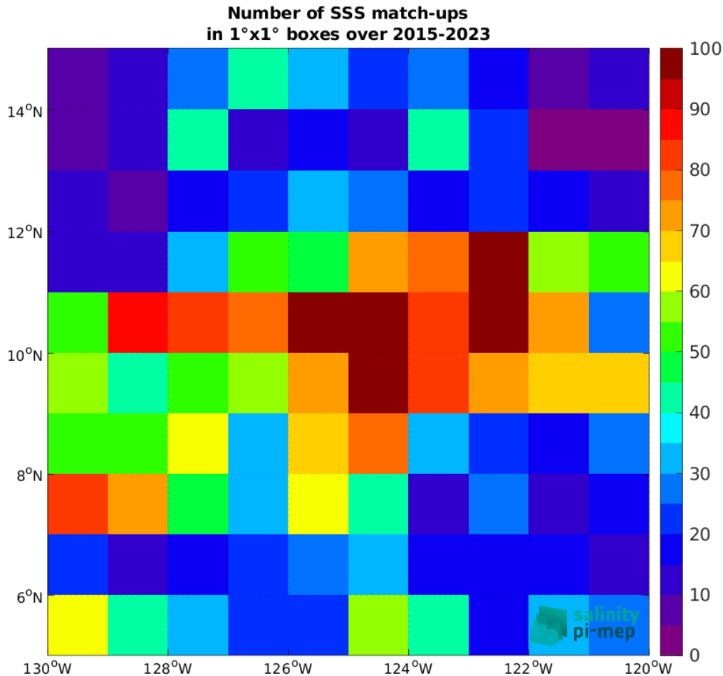
Figure 5: Number of SSS match-ups between Argo SSS and the SMAP SSS L3 v5.3 - Monthly (RSS) SSS product for the SPURS 2 Pi-MEP region over 1^\circ \times 1^\circ boxes and for the full satellite product period.
