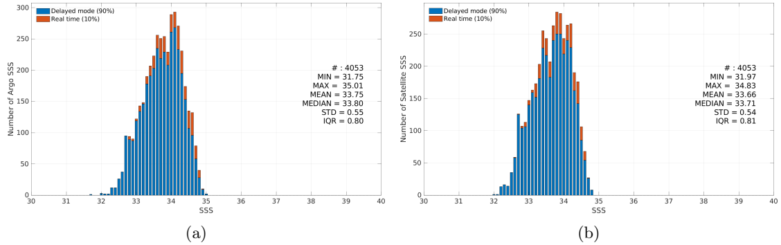
Figure 3: Histograms of SSS from Argo (a) and SMAP SSS L3 v5.3 - Monthly (RSS) (b) considering all match-up pairs per bins of 0.1 over the SPURS 2 Pi-MEP region and for the full satellite product period.
