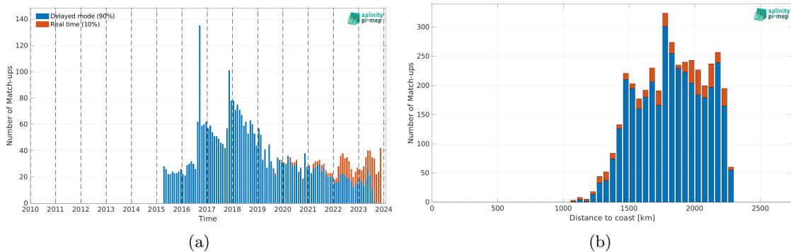
Figure 2: Number of match-ups between Argo and SMAP SSS L3 v5.3 - Monthly (RSS) SSS as a function of time (a) and as function of the distance to coast (b) over the SPURS 2 Pi-MEP region and for the full satellite product period.
