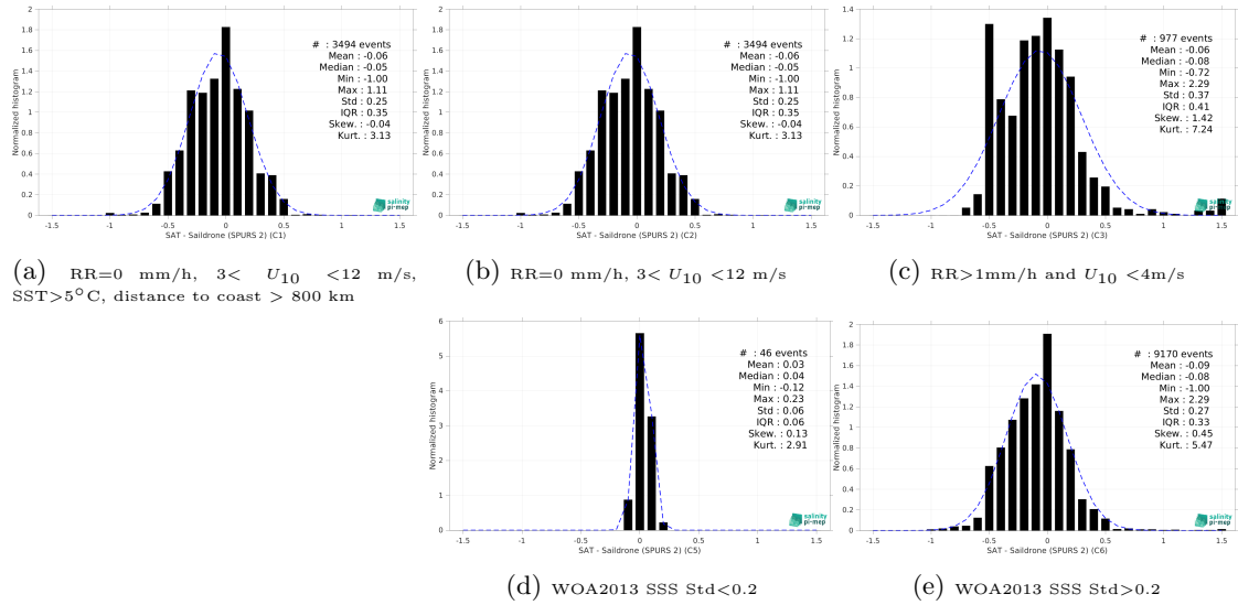
Figure 13: Normalized histogram of \Delta SSS (SMAP SSS L3 v5 - 8-Day running (RSS) - Sailability (SPURS 2)) for 5 different subdatasets corresponding to: RR=0 mm/h, 3 < U_{10} < 12 m/s, SST>5°C, distance to coast > 800 km (a), RR=0 mm/h, 3 < U_{10} < 12 m/s (b), RR>1mm/h and U_{10} < 4 m/s (c), WOA2013 SSS Std<0.2 (d), WOA2013 SSS Std>0.2 (e).
