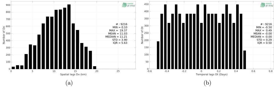
Figure 5: Histograms of the spatial (a) and temporal (b) lags between the location/time of the Saildrone (SPURS 2) measurement and the date of the corresponding SMAP SSS L3 v5 - 8-Day running (RSS) SSS pixel.
