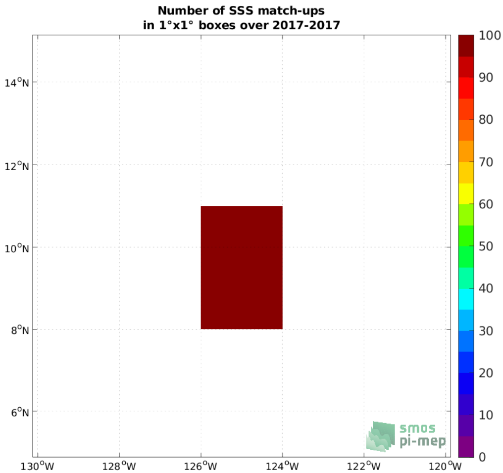
Figure 4: Number of SSS match-ups between SAILDRONE (SPURS 2) SSS and the SMAP SSS L3 v5 - 8-Day running (RSS) SSS product for the SPURS 2 Pi-MEP region over 1°x1° boxes and for the full satellite product period.
