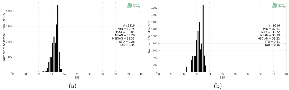
Figure 2: Histograms of SSS from Saildrone (SPURS 2) (a) and SMAP SSS L3 v5 - 8-Day running (RSS) (b) considering all match-up pairs per bins of 0.1 over the SPURS 2 Pi-MEP region and for the full satellite product period.
