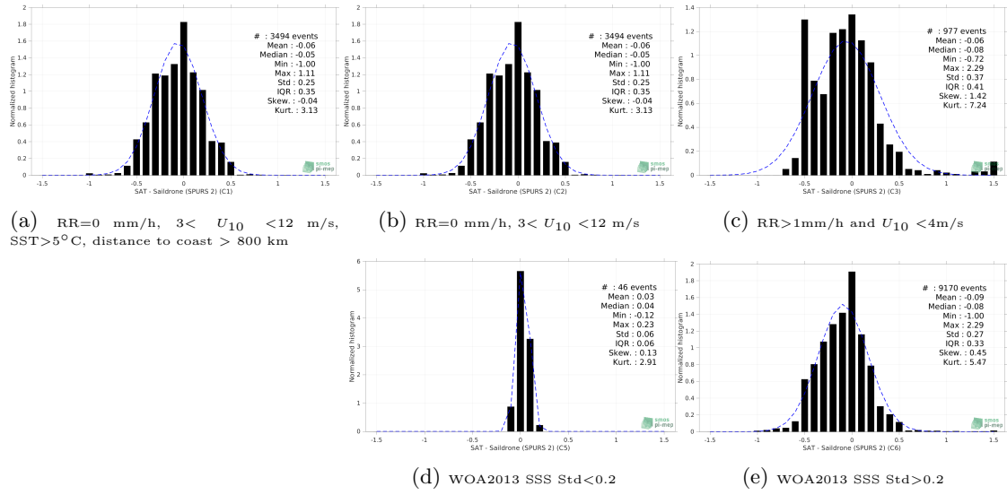
Figure 13: Normalized histogram of \Delta SSS (SMAP SSS L3 v5 - 8-Day running (RSS) - Saldrone (SPURS 2)) for 5 different subdatasets corresponding to: RR=0 mm/h, 3 < U_{10} < 12 m/s, SST > 5°C, distance to coast > 800 km (a), RR=0 mm/h, 3 < U_{10} < 12 m/s (b), RR > 1mm/h and U_{10} < 4 m/s (c), WOA2013 SSS Std < 0.2 (d), WOA2013 SSS Std > 0.2 (e).
