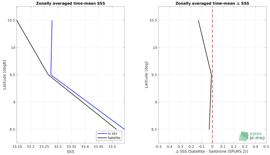
Figure 8: Left panel: Zonal mean SSS from SMAP SSS L3 v5 - 8-Day running (RSS) satellite product (black) and from Sairdron (SPURS 2) (blue). Right panel: Zonal mean of \Delta SSS (Satellite - Sairdron (SPURS 2)) for all the collected Pi-MEP match-up pairs estimated over the full satellite product period.
