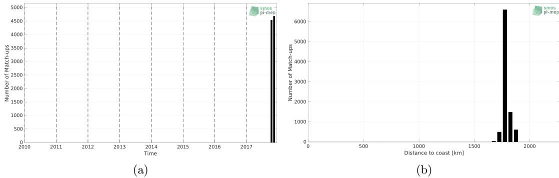
Figure 1: Number of match-ups between Saildrone (SPURS 2) and SMAP SSS L3 v5 - 8-Day running (RSS) SSS as a function of time (a) and as function of the distance to coast (b) over the SPURS 2 Pi-MEP region and for the full satellite product period.
