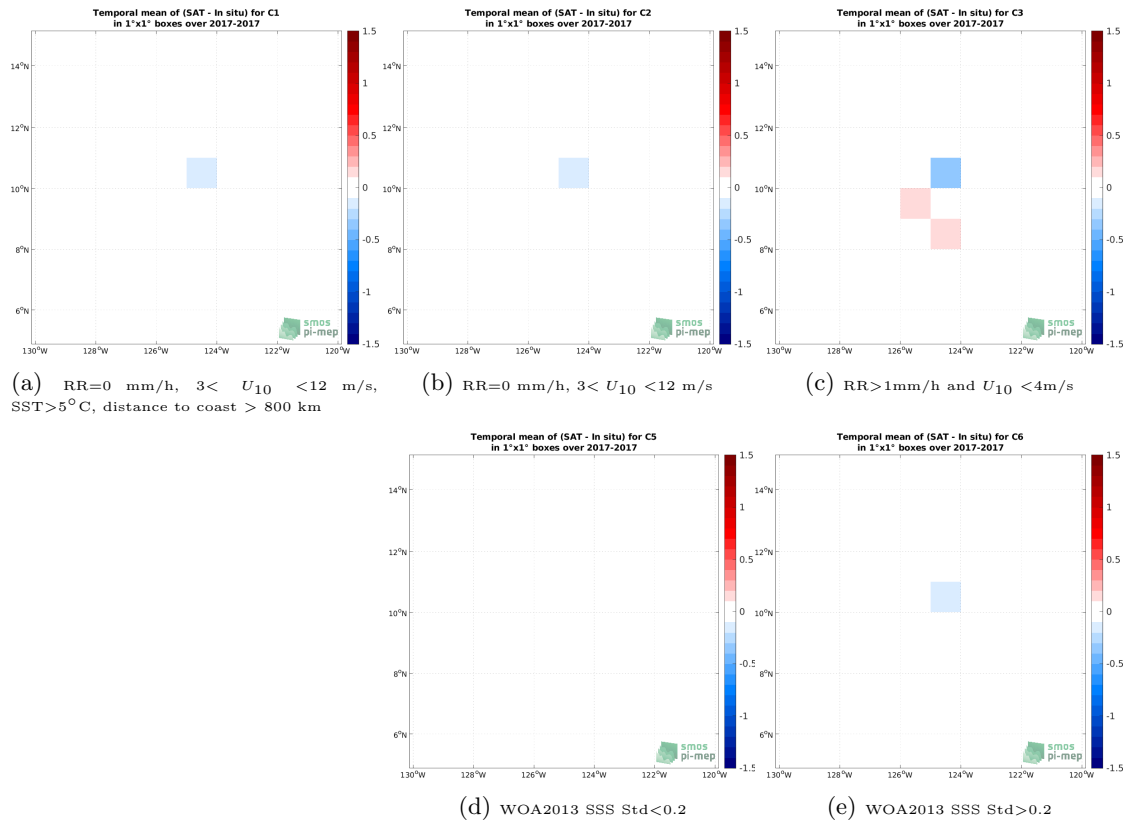
Figure 12: Temporal mean gridded over spatial boxes of size 1^\circ \times 1^\circ of \Delta SSS (SMAP SSS L3 v5 - 8-Day running (RSS) - Sairdron (SPURS 2)) for 5 different subdatasets corresponding to:RR=0 mm/h, 3 < U_{10} < 12 m/s, SST >5^\circ C, distance to coast > 800 km (a), RR=0 mm/h, 3 < U_{10} < 12 m/s (b), RR >1 mm/h and U_{10} < 4 m/s (c), WOA2013 SSS Std <0.2 (d), WOA2013 SSS Std >0.2 (e).
