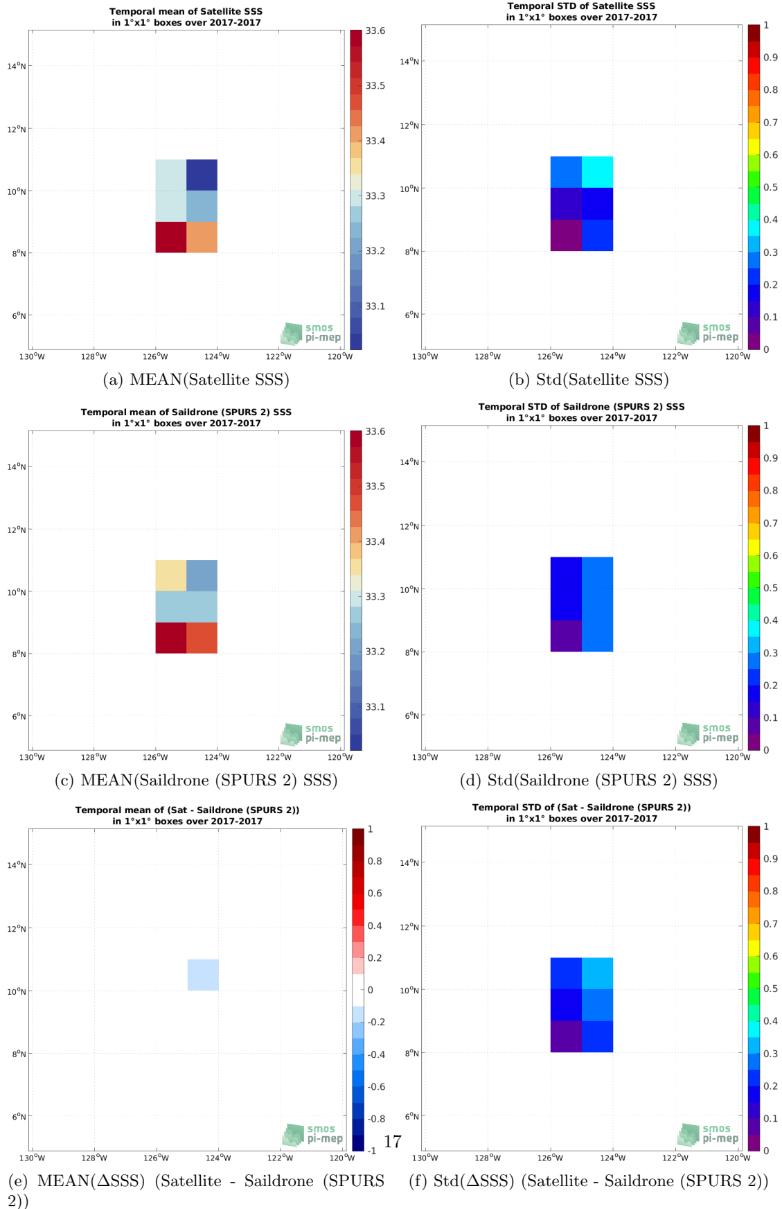
Figure 6: Temporal mean (left) and Std (right) of SSS from SMAP SSS L3 v5 - 8-Day running (RSS) (top), Saildrone (SPURS 2) (middle), and of \Delta SSS (Satellite - Saildrone (SPURS 2)). Only match-up pairs are used to generate these maps.
