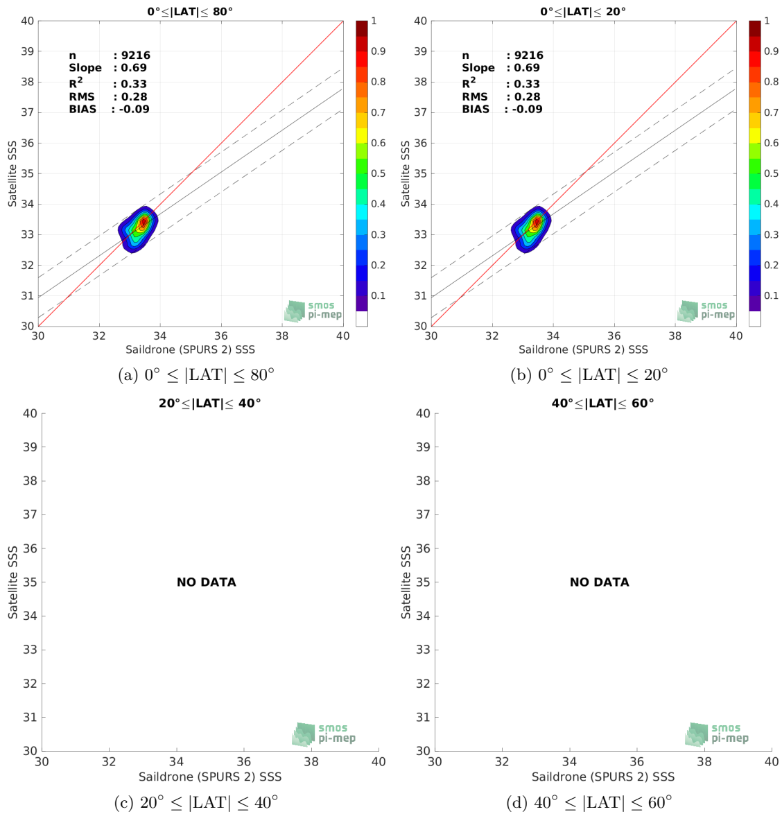
Figure 9: Contour maps of the concentration of SMAP SSS L3 v5 - 8-Day running (RSS) SSS (y-axis) versus Saildrone (SPURS 2) SSS (x-axis) at match-up pairs for different latitude bands. For each plot, the red line shows x=y . The black thin and dashed lines indicate a linear fit through the data cloud and the \pm 95\% confidence levels, respectively. The number match-up pairs n , the slope and R^2 coefficient of the linear fit, the root mean square (RMS) and the mean bias between satellite and in situ data are indicated for each latitude band in each plots.
