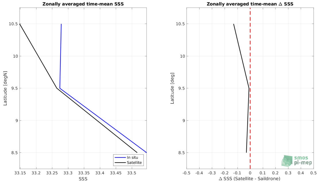
Figure 7: Left panel: Zonal mean SSS from SMAP SSS L3 v5 - 8-Day running (RSS) satellite product (black) and from Sairdrone (blue). Right panel: Zonal mean of \Delta SSS (Satellite - Sairdrone) for all the collected Pi-MEP match-up pairs estimated over the full satellite product period.
