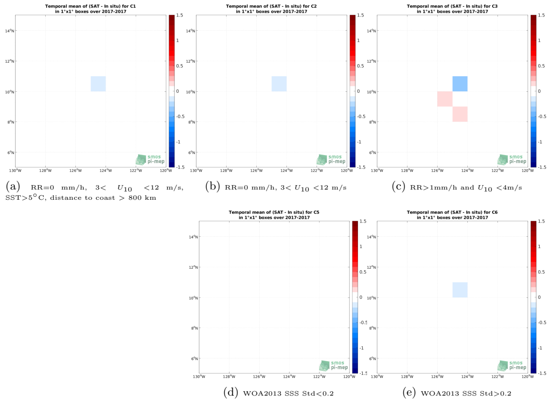
Figure 11: Temporal mean gridded over spatial boxes of size 1^\circ \times 1^\circ of \Delta SSS (SMAP SSS L3 v5 - 8-Day running (RSS) - Saildrone) for 5 different subdatasets corresponding to:RR=0 mm/h, 3 < U_{10} < 12 m/s, SST >5^\circ C, distance to coast > 800 km (a), RR=0 mm/h, 3 < U_{10} < 12 m/s (b), RR >1 mm/h and U_{10} < 4 m/s (c), WOA2013 SSS Std <0.2 (d), WOA2013 SSS Std >0.2 (e).
