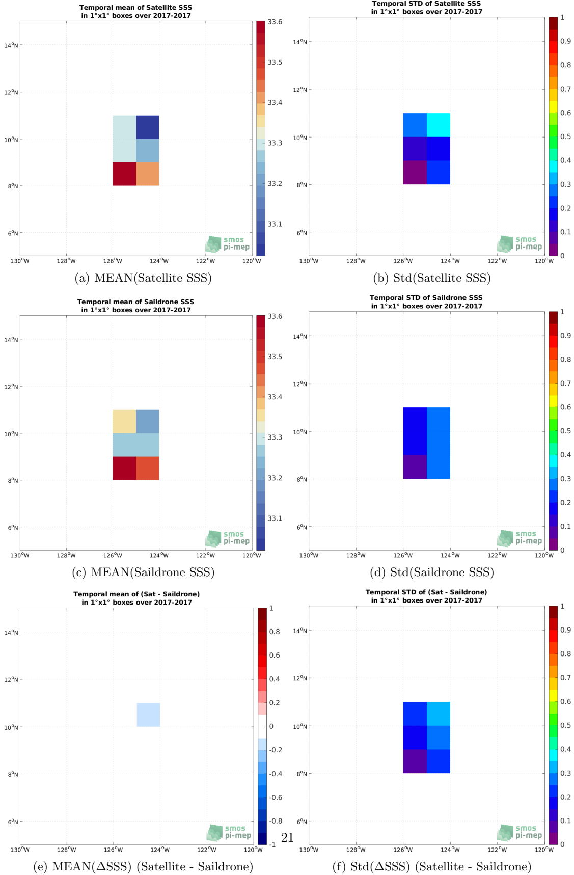
Figure 5: Temporal mean (left) and Std (right) of SSS from SMAP SSS L3 v5 - 8-Day running (RSS) (top), Saildrone (middle), and of \Delta SSS (Satellite - Saildrone). Only match-up pairs are used to generate these maps.
