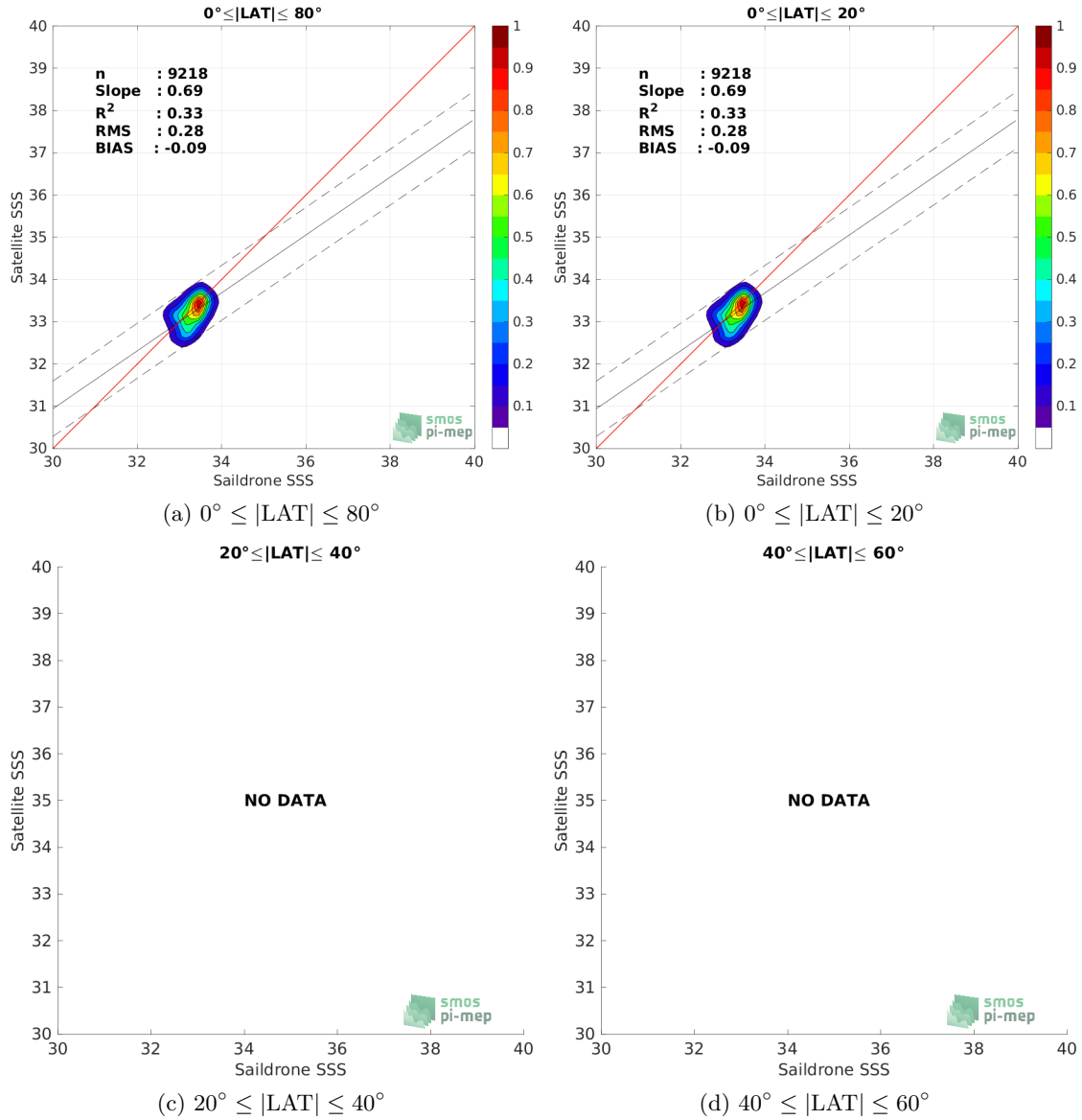
Figure 8: Contour maps of the concentration of SMAP SSS L3 v5 - 8-Day running (RSS) SSS (y-axis) versus Saildrone SSS (x-axis) at match-up pairs for different latitude bands. For each plot, the red line shows x=y . The black thin and dashed lines indicate a linear fit through the data cloud and the \pm 95\% confidence levels, respectively. The number match-up pairs n , the slope and R^2 coefficient of the linear fit, the root mean square (RMS) and the mean bias between satellite and in situ data are indicated for each latitude band in each plots.
