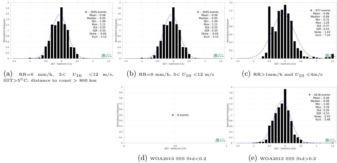
Figure 12: Normalized histogram of \Delta SSS (SMAP SSS L3 v5 - 8-Day running (RSS) - Sairdrone) for 5 different subdatasets corresponding to: RR=0 mm/h, 3 < U_{10} < 12 m/s, SST > 5°C, distance to coast > 800 km (a), RR=0 mm/h, 3 < U_{10} < 12 m/s (b), RR > 1mm/h and U_{10} < 4 m/s (c), WOA2013 SSS Std < 0.2 (d), WOA2013 SSS Std > 0.2 (e).
