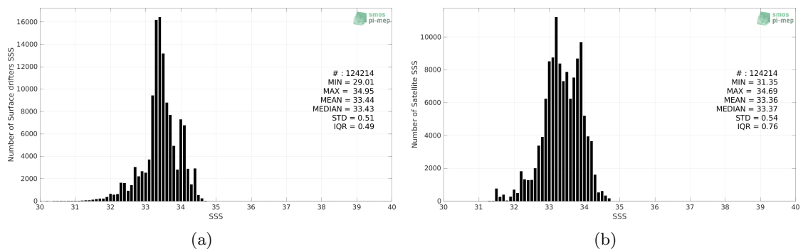
Figure 2: Histograms of SSS from Surface drifters (a) and SMAP SSS L3 v5 - 8-Day running (RSS) (b) considering all match-up pairs per bins of 0.1 over the SPURS 2 Pi-MEP region and for the full satellite product period.
