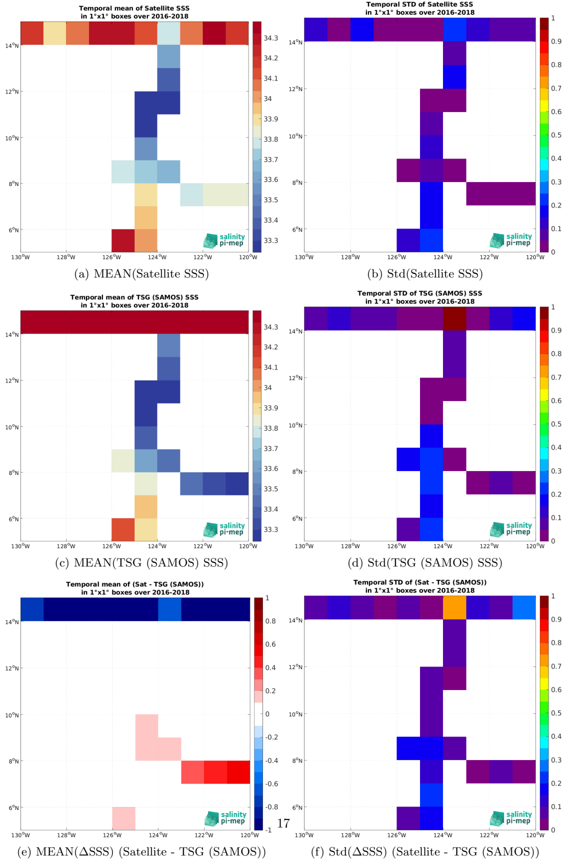
Figure 7: Temporal mean (left) and Std (right) of SSS from SMAP SSS L3 v5.0 - 8-Day running (JPL) (top), TSG (SAMOS) (middle), and of \Delta SSS (Satellite - TSG (SAMOS)). Only match-up pairs are used to generate these maps.
