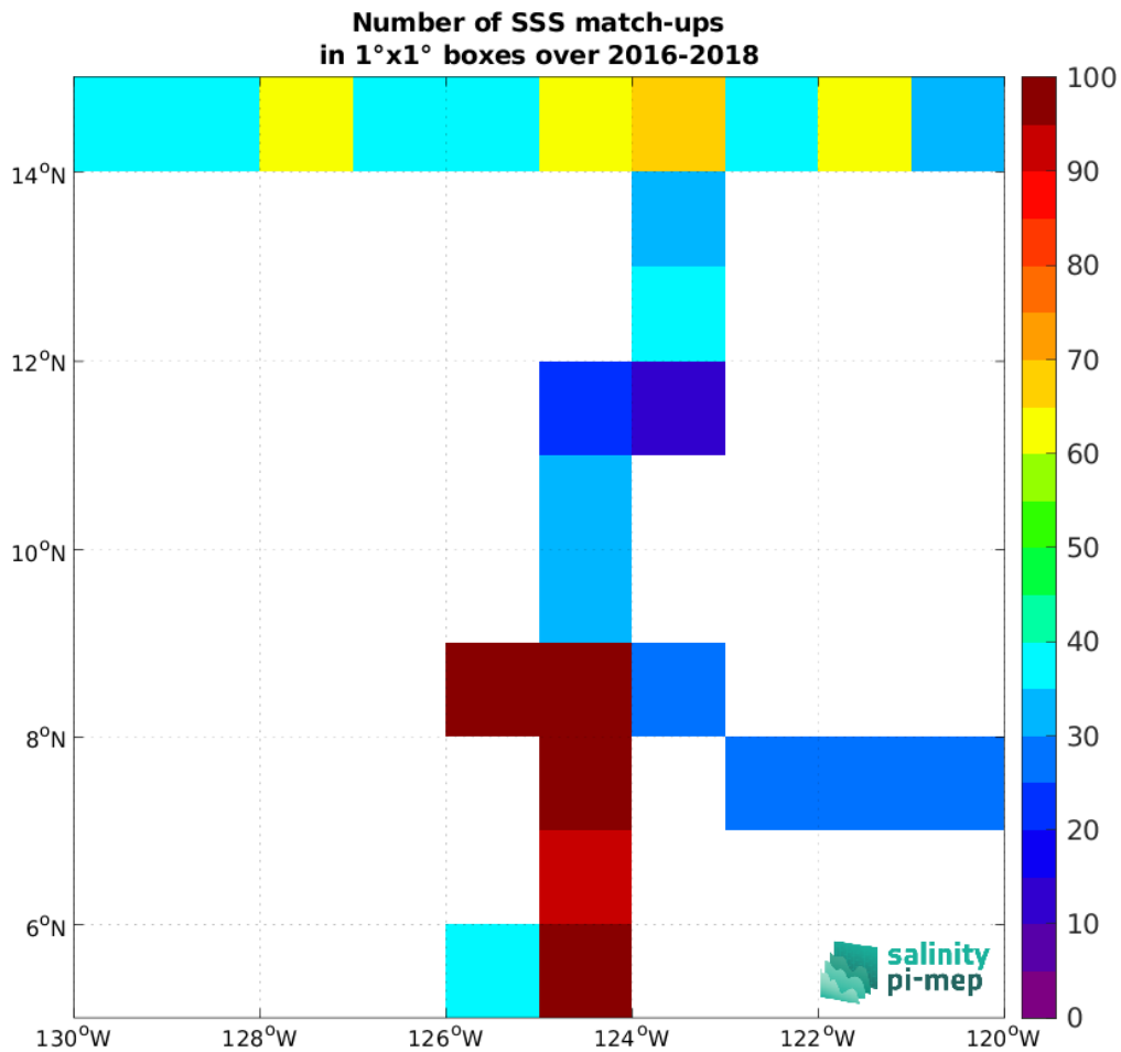
Figure 4: Number of SSS match-ups between TSG (SAMOS) SSS and the SMAP SSS L3 v5.0 - 8-Day running (JPL) SSS product for the SPURS 2 Pi-MEP region over 1^\circ \times 1^\circ boxes and for the full satellite product period.
