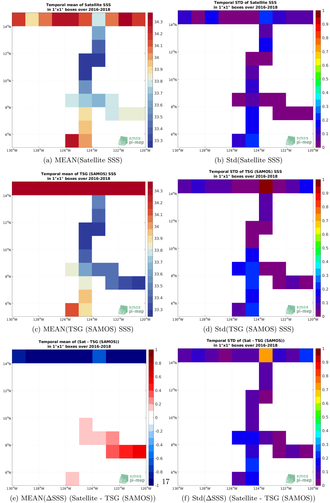
Figure 6: Temporal mean (left) and Std (right) of SSS from SMAP SSS L3 v5.0 - 8-Day running (JPL) (top), TSG (SAMOS) (middle), and of \Delta SSS (Satellite - TSG (SAMOS)). Only match-up pairs are used to generate these maps.
