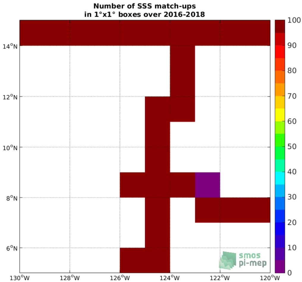
Figure 4: Number of SSS match-ups between TSG (SAMOS) SSS and the SMAP SSS L3 v5.0 - 8-Day running (JPL) SSS product for the SPURS 2 Pi-MEP region over 1°×1° boxes and for the full satellite product period.
