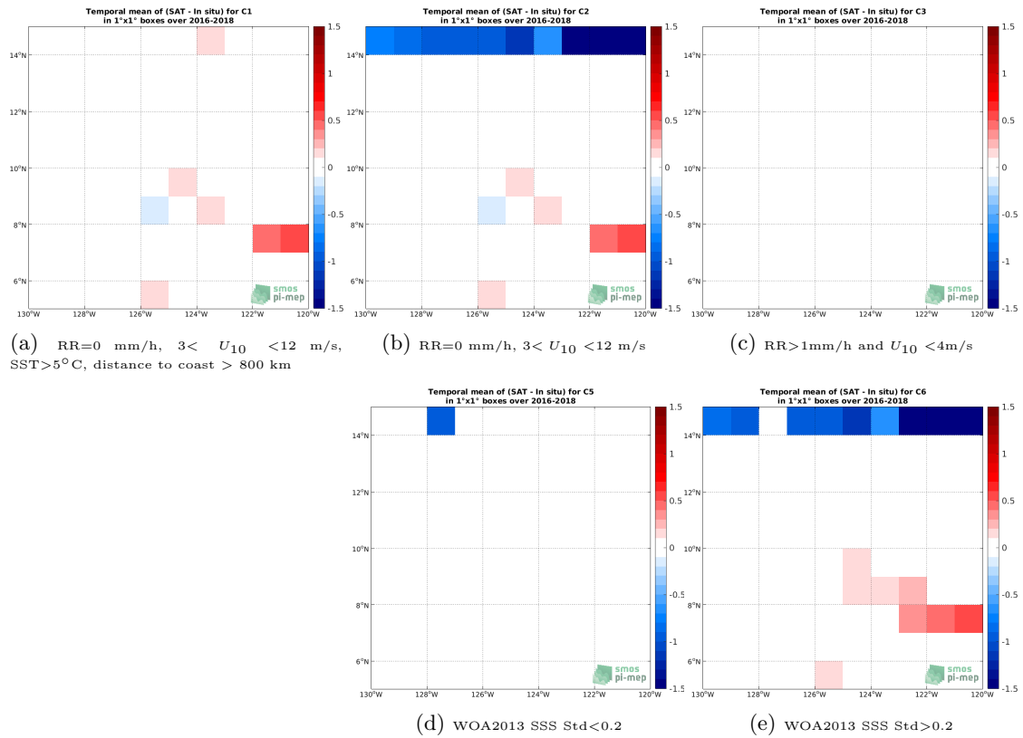
Figure 12: Temporal mean gridded over spatial boxes of size 1^\circ \times 1^\circ of \Delta\text{SSS} (SMAP SSS L3 v5.0 - 8-Day running (JPL) - TSG (SAMOS)) for 5 different subdatasets corresponding to:RR=0 mm/h, 3 < U_{10} < 12 m/s, SST >5^\circ\text{C} , distance to coast > 800 km (a), RR=0 mm/h, 3 < U_{10} < 12 m/s (b), RR >1 mm/h and U_{10} < 4 m/s (c), WOA2013 SSS Std <0.2 (d), WOA2013 SSS Std >0.2 (e).
