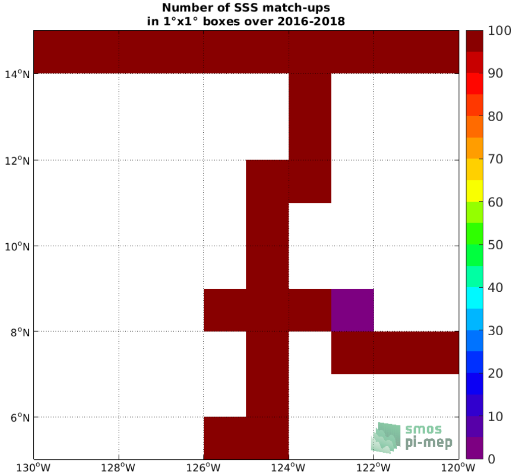
Figure 4: Number of SSS match-ups between TSG (SAMOS) SSS and the SMAP SSS L3 v5.0 - 8-Day running (JPL) SSS product for the SPURS 2 Pi-MEP region over 1°x1° boxes and for the full satellite product period.
