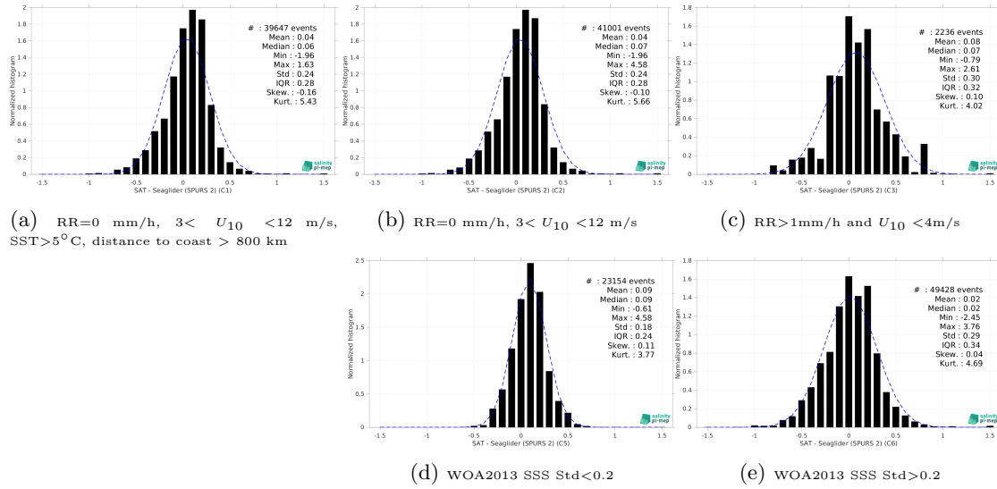
Figure 15: Normalized histogram of \Delta SSS (SMAP SSS L3 v5.0 - 8-Day running (JPL) - Seaglider (SPURS 2)) for 5 different subdatasets corresponding to: RR=0 mm/h, 3 < U_{10} < 12 m/s, SST > 5°C, distance to coast > 800 km (a), RR=0 mm/h, 3 < U_{10} < 12 m/s (b), RR > 1mm/h and U_{10} < 4 m/s (c), WOA2013 SSS Std < 0.2 (d), WOA2013 SSS Std > 0.2 (e).
