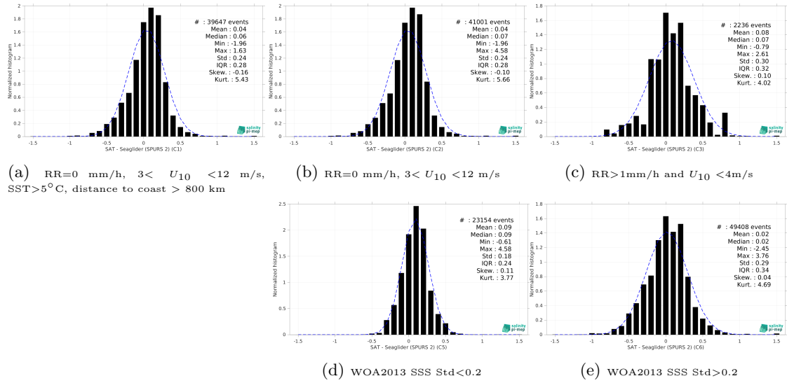
Figure 15: Normalized histogram of \Delta SSS (SMAP SSS L3 v5.0 - 8-Day running (JPL) - Seaglider (SPURS 2)) for 5 different subdatasets corresponding to: RR=0 mm/h, 3 < U_{10} < 12 m/s, SST>5°C, distance to coast > 800 km (a), RR=0 mm/h, 3 < U_{10} < 12 m/s (b), RR>1mm/h and U_{10} < 4 m/s (c), WOA2013 SSS Std<0.2 (d), WOA2013 SSS Std>0.2 (e).
