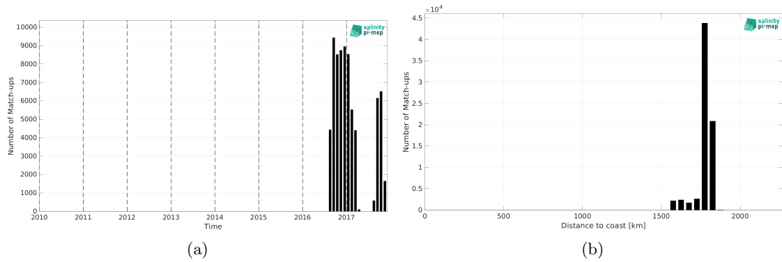
Figure 2: Number of match-ups between Seaglider (SPURS 2) and SMAP SSS L3 v5.0 - 8-Day running (JPL) SSS as a function of time (a) and as function of the distance to coast (b) over the SPURS 2 Pi-MEP region and for the full satellite product period.
