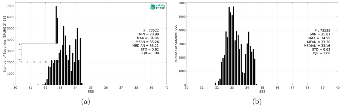
Figure 3: Histograms of SSS from Seaglider (SPURS 2) (a) and SMAP SSS L3 v5.0 - 8-Day running (JPL) (b) considering all match-up pairs per bins of 0.1 over the SPURS 2 Pi-MEP region and for the full satellite product period.
