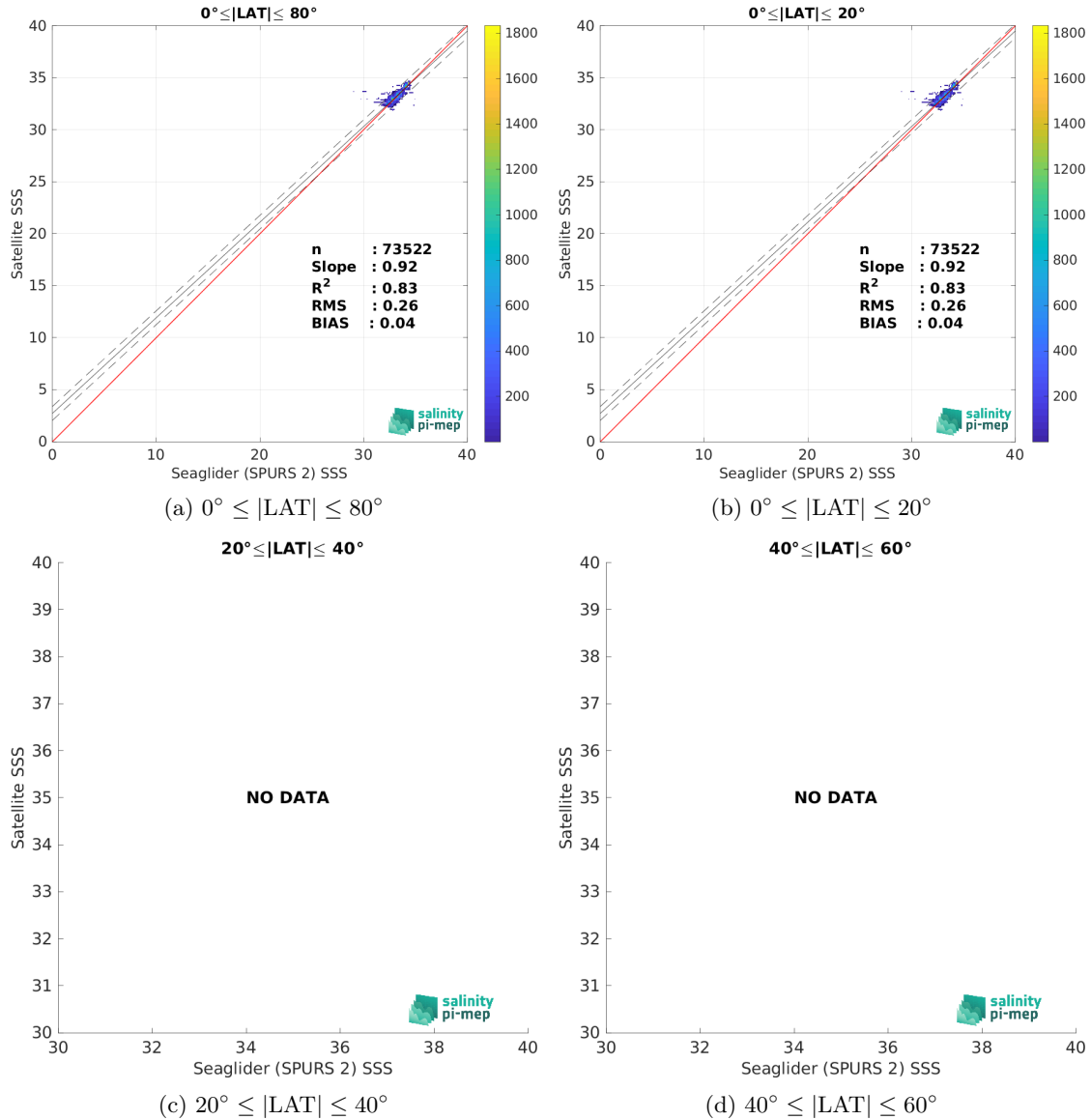
Figure 10: Contour maps of the concentration of SMAP SSS L3 v5.0 - 8-Day running (JPL) SSS (y-axis) versus Seaglider (SPURS 2) SSS (x-axis) at match-up pairs for different latitude bands. For each plot, the red line shows x=y . The black thin and dashed lines indicate a linear fit through the data cloud and the \pm 95\% confidence levels, respectively. The number match-up pairs n , the slope and R^2 coefficient of the linear fit, the root mean square (RMS) and the mean bias between satellite and in situ data are indicated for each latitude band in each plots.
