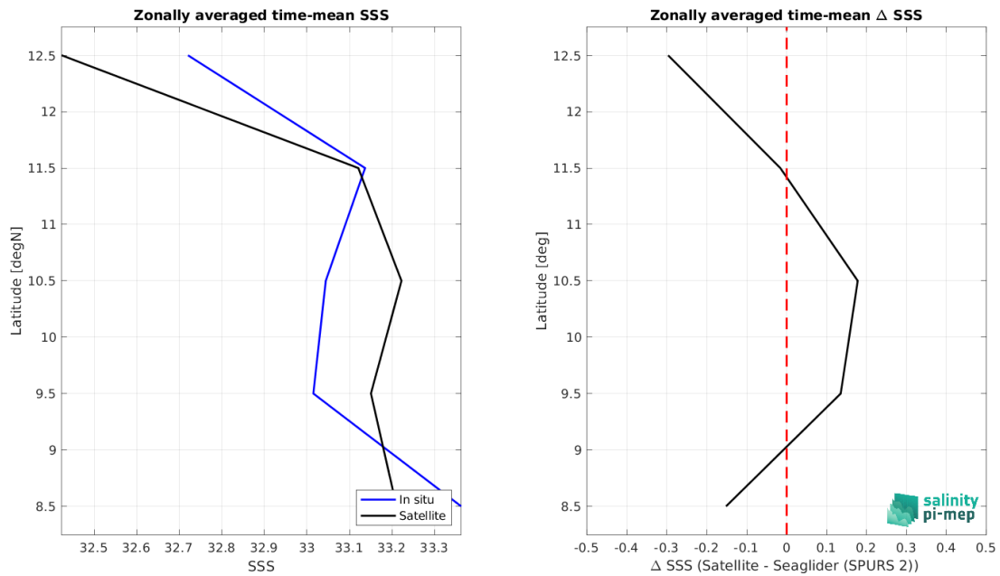
Figure 9: Left panel: Zonal mean SSS from SMAP SSS L3 v5.0 - 8-Day running (JPL) satellite product (black) and from Seaglider (SPURS 2) (blue). Right panel: Zonal mean of \Delta SSS (Satellite - Seaglider (SPURS 2)) for all the collected Pi-MEP match-up pairs estimated over the full satellite product period.
