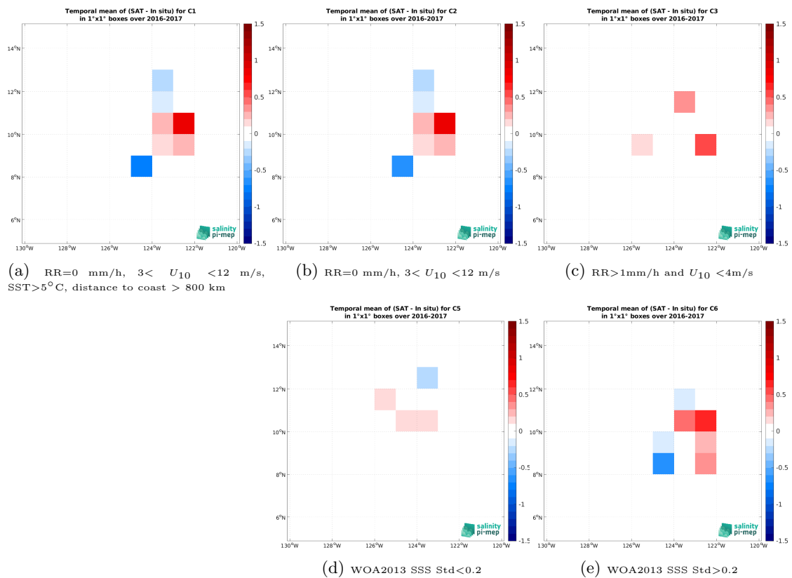
Figure 14: Temporal mean gridded over spatial boxes of size 1^\circ \times 1^\circ of \Delta SSS (SMAP SSS L3 v5.0 - 8-Day running (JPL) - Seaglider (SPURS 2)) for 5 different subdatasets corresponding to: RR=0 mm/h, 3 < U_{10} < 12 m/s, SST > 5°C, distance to coast > 800 km (a), RR=0 mm/h, 3 < U_{10} < 12 m/s (b), RR > 1mm/h and U_{10} < 4 m/s (c), WOA2013 SSS Std < 0.2 (d), WOA2013 SSS Std > 0.2 (e).
