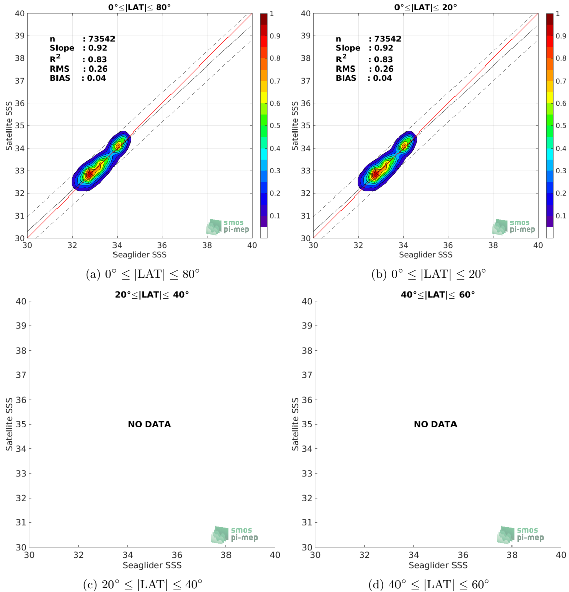
Figure 8: Contour maps of the concentration of SMAP SSS L3 v5.0 - 8-Day running (JPL) SSS (y-axis) versus Seaglider SSS (x-axis) at match-up pairs for different latitude bands. For each plot, the red line shows x=y . The black thin and dashed lines indicate a linear fit through the data cloud and the \pm 95\% confidence levels, respectively. The number match-up pairs n , the slope and R^2 coefficient of the linear fit, the root mean square (RMS) and the mean bias between satellite and in situ data are indicated for each latitude band in each plots.
