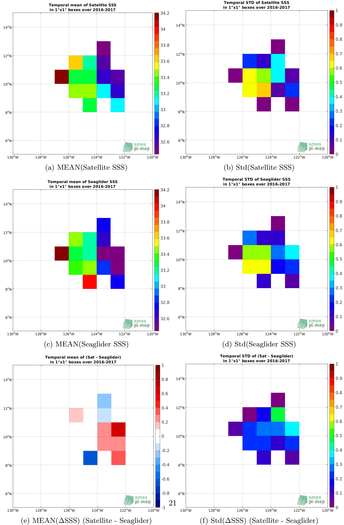
Figure 5: Temporal mean (left) and Std (right) of SSS from SMAP SSS L3 v5.0 - 8-Day running (JPL) (top), Seaglider (middle), and of \Delta SSS (Satellite - Seaglider). Only match-up pairs are used to generate these maps.
