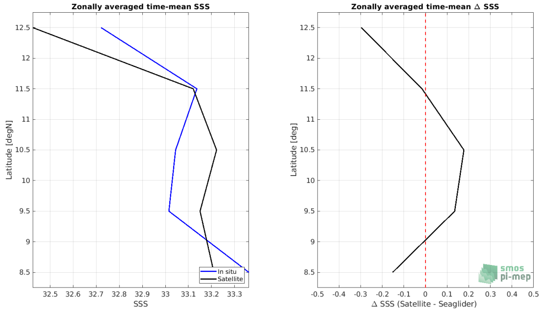
Figure 7: Left panel: Zonal mean SSS from SMAP SSS L3 v5.0 - 8-Day running (JPL) satellite product (black) and from Seaglider (blue). Right panel: Zonal mean of \Delta SSS (Satellite - Seaglider) for all the collected Pi-MEP match-up pairs estimated over the full satellite product period.
