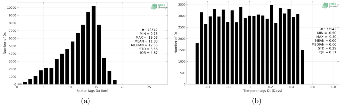
Figure 4: Histograms of the spatial (a) and temporal (b) lags between the location/time of the Seaglider measurement and the date of the corresponding SMAP SSS L3 v5.0 - 8-Day running (JPL) SSS pixel.
