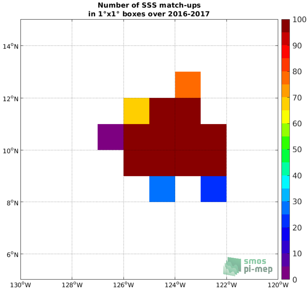
Figure 3: Number of SSS match-ups between Seagliders SSS and the SMAP SSS L3 v5.0 - 8-Day running (JPL) SSS product for the SPURS 2 Pi-MEP region over 1°x1° boxes and for the full satellite product period.
