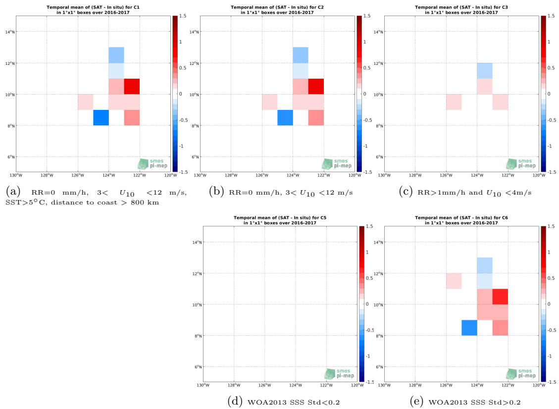
Figure 11: Temporal mean gridded over spatial boxes of size 1^\circ \times 1^\circ of \Delta SSS (SMAP SSS L3 v5.0 - 8-Day running (JPL) - Seaglider) for 5 different subdatasets corresponding to:RR=0 mm/h, 3 < U_{10} < 12 m/s, SST >5^\circ\text{C} , distance to coast > 800 km (a), RR=0 mm/h, 3 < U_{10} < 12 m/s (b), RR >1 mm/h and U_{10} < 4 m/s (c), WOA2013 SSS Std <0.2 (d), WOA2013 SSS Std >0.2 (e).
