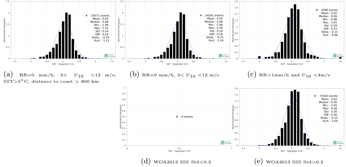
Figure 12: Normalized histogram of \Delta SSS (SMAP SSS L3 v5.0 - 8-Day running (JPL) - Seaglider) for 5 different subdatasets corresponding to: RR=0 mm/h, 3 < U_{10} < 12 m/s, SST > 5°C, distance to coast > 800 km (a), RR=0 mm/h, 3 < U_{10} < 12 m/s (b), RR > 1mm/h and U_{10} < 4 m/s (c), WOA2013 SSS Std < 0.2 (d), WOA2013 SSS Std > 0.2 (e).
