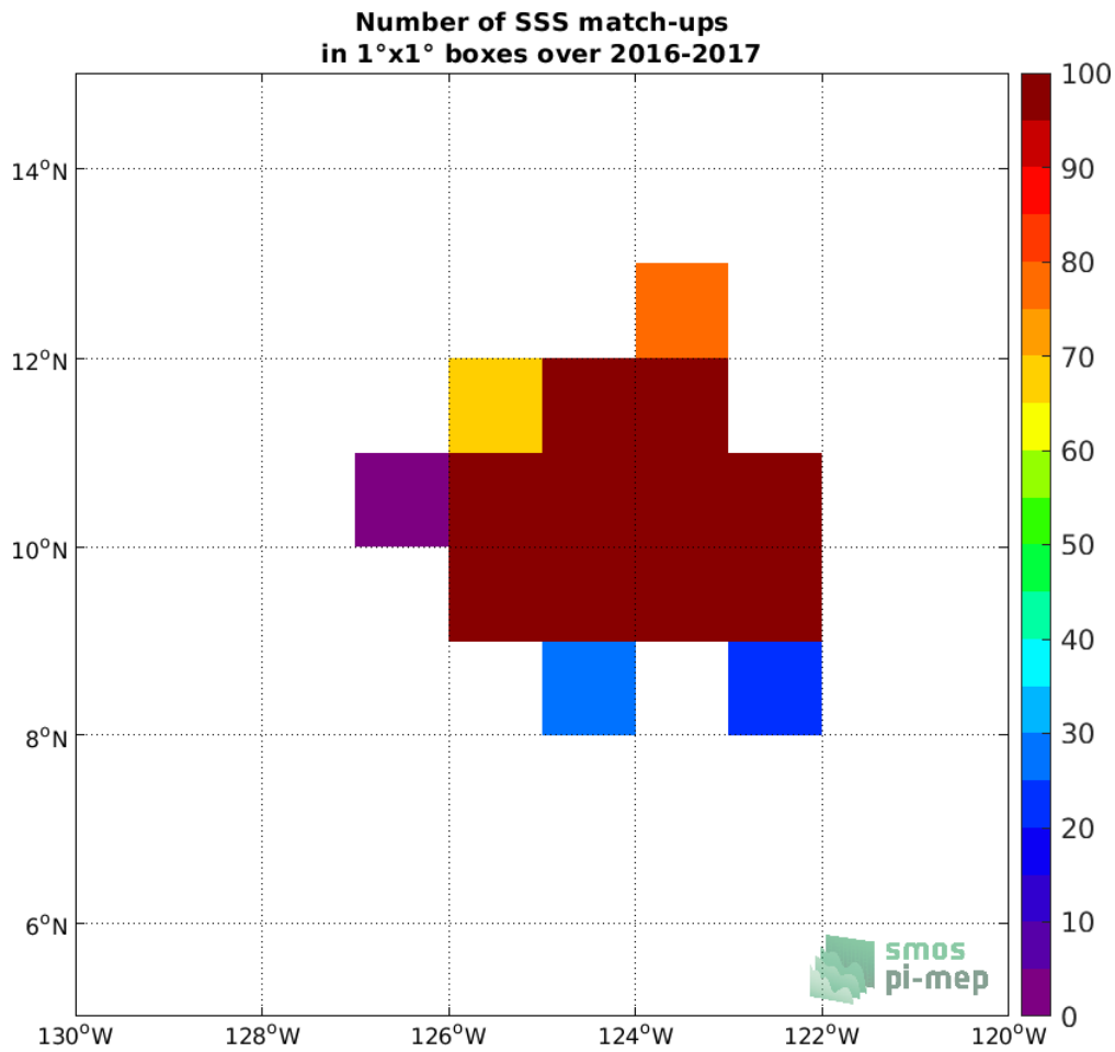
Figure 3: Number of SSS match-ups between Seaglider SSS and the SMAP SSS L3 v5.0 - 8-Day running (JPL) SSS product for the SPURS 2 Pi-MEP region over 1°x1° boxes and for the full satellite product period.
