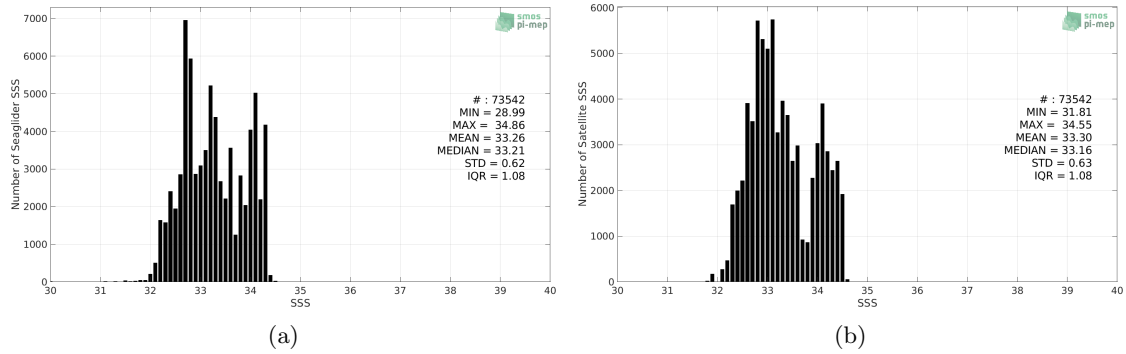
Figure 2: Histograms of SSS from Seagliders (a) and SMAP SSS L3 v5.0 - 8-Day running (JPL) (b) considering all match-up pairs per bins of 0.1 over the SPURS 2 Pi-MEP region and for the full satellite product period.
