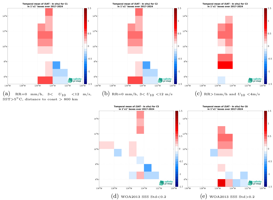
Figure 14: Temporal mean gridded over spatial boxes of size 1^\circ \times 1^\circ of \Delta\text{SSS} (SMAP SSS L3 v5.0 - 8-Day running (JPL) - Sairdrone) for 5 different subdatasets corresponding to:RR=0 mm/h, 3 < U_{10} < 12 m/s, SST>5°C, distance to coast > 800 km (a), RR=0 mm/h, 3 < U_{10} < 12 m/s (b), RR>1mm/h and U_{10} < 4 m/s (c), WOA2013 SSS Std<0.2 (d), WOA2013 SSS Std>0.2 (e).
