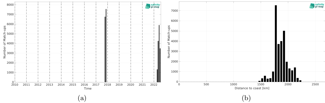
Figure 2: Number of match-ups between Saildrone and SMAP SSS L3 v5.0 - 8-Day running (JPL) SSS as a function of time (a) and as function of the distance to coast (b) over the SPURS 2 Pi-MEP region and for the full satellite product period.
