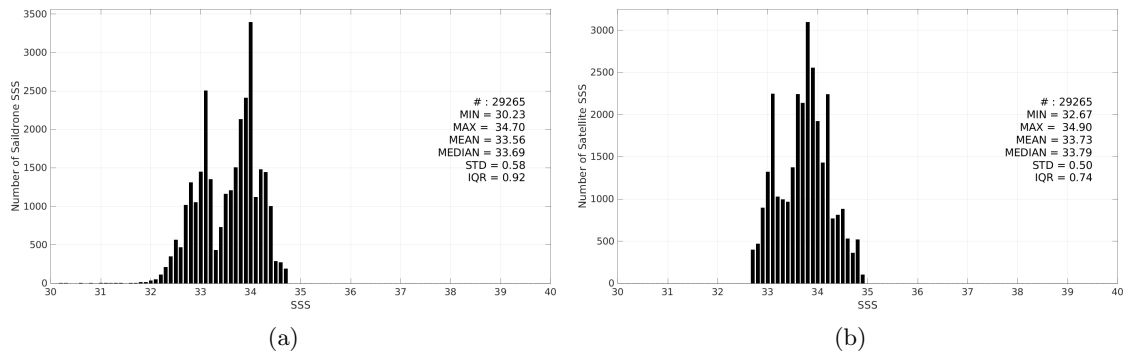
Figure 3: Histograms of SSS from Saildrone (a) and SMAP SSS L3 v5.0 - 8-Day running (JPL) (b) considering all match-up pairs per bins of 0.1 over the SPURS 2 Pi-MEP region and for the full satellite product period.
