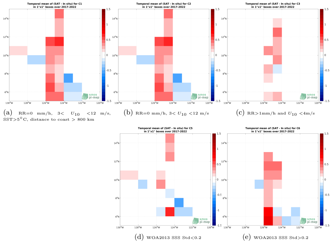
Figure 12: Temporal mean gridded over spatial boxes of size 1^\circ \times 1^\circ of \Delta SSS (SMAP SSS L3 v5.0 - 8-Day running (JPL) - Saifdrone) for 5 different subdatasets corresponding to:RR=0 mm/h, 3 < U_{10} < 12 m/s, SST >5^\circ\text{C} , distance to coast > 800 km (a), RR=0 mm/h, 3 < U_{10} < 12 m/s (b), RR >1 mm/h and U_{10} < 4 m/s (c), WOA2013 SSS Std <0.2 (d), WOA2013 SSS Std >0.2 (e).
