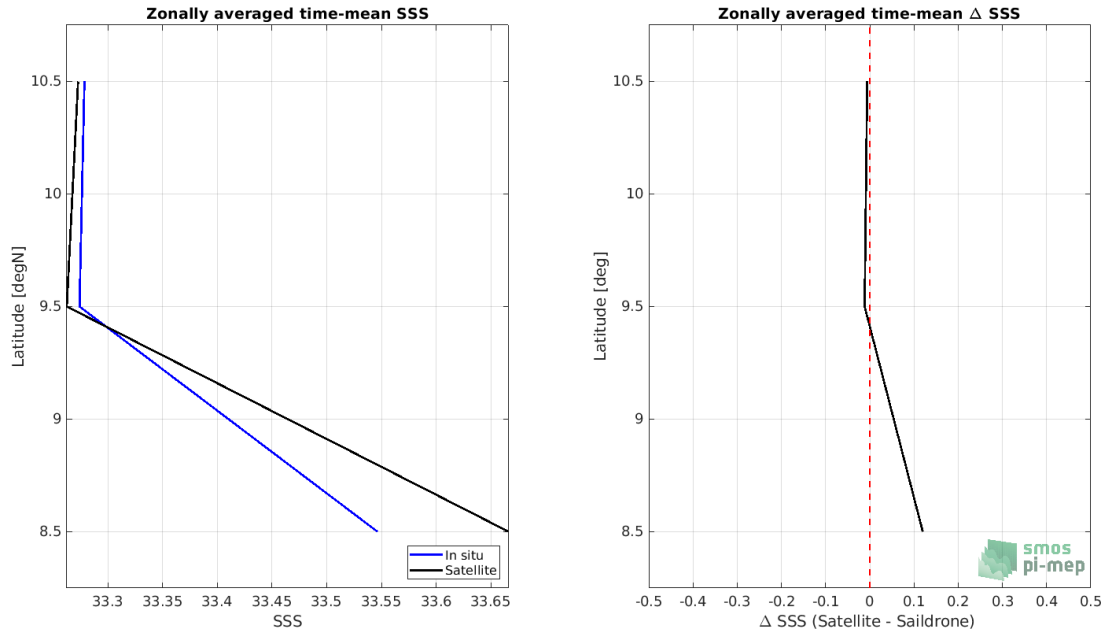
Figure 7: Left panel: Zonal mean SSS from SMAP SSS L3 v5.0 - 8-Day running (JPL) satellite product (black) and from Sairdrone (blue). Right panel: Zonal mean of \Delta SSS (Satellite - Sairdrone) for all the collected Pi-MEP match-up pairs estimated over the full satellite product period.
