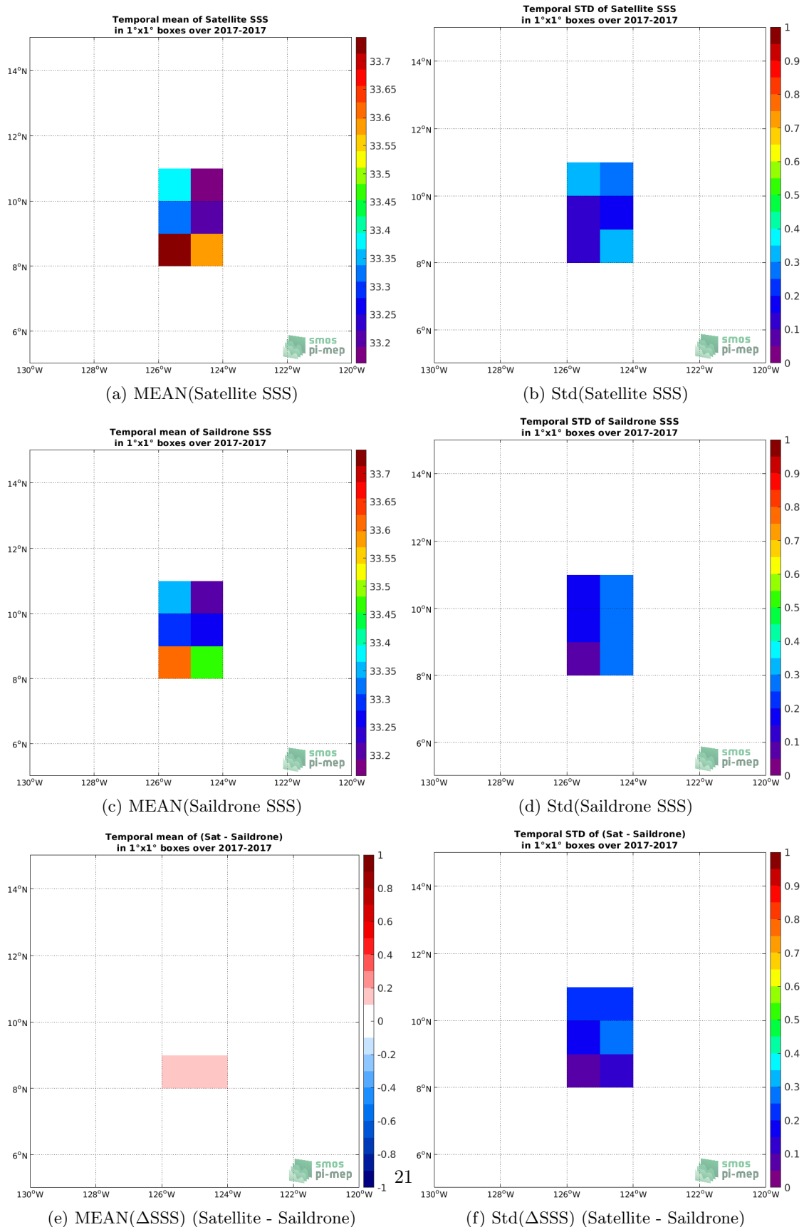
Figure 5: Temporal mean (left) and Std (right) of SSS from SMAP SSS L3 v5.0 - 8-Day running (JPL) (top), Saildrone (middle), and of \Delta SSS (Satellite - Saildrone). Only match-up pairs are used to generate these maps.
