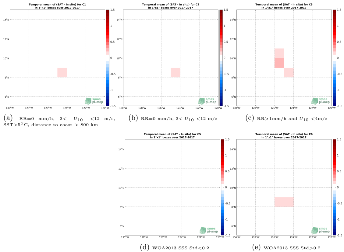
Figure 11: Temporal mean gridded over spatial boxes of size 1^\circ \times 1^\circ of \Delta\text{SSS} (SMAP SSS L3 v5.0 - 8-Day running (JPL) - Saildrone) for 5 different subdatasets corresponding to:RR=0 mm/h, 3 < U_{10} < 12 m/s, SST >5^\circ\text{C} , distance to coast > 800 km (a), RR=0 mm/h, 3 < U_{10} < 12 m/s (b), RR >1 mm/h and U_{10} < 4 m/s (c), WOA2013 SSS Std <0.2 (d), WOA2013 SSS Std >0.2 (e).
