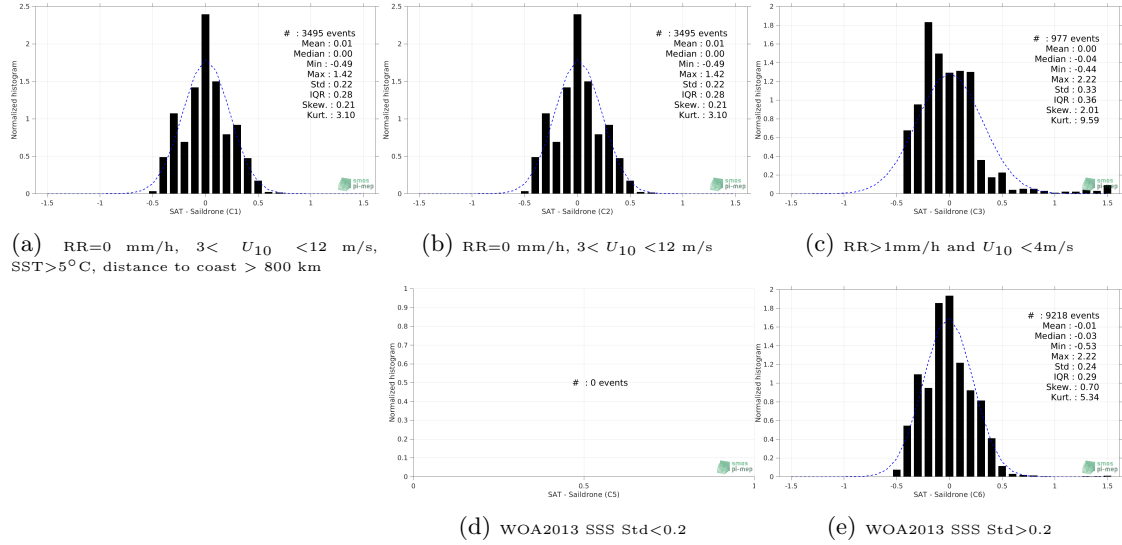
Figure 12: Normalized histogram of \Delta SSS (SMAP SSS L3 v5.0 - 8-Day running (JPL) - Saildrone) for 5 different subdatasets corresponding to: RR=0 mm/h, 3 < U_{10} < 12 m/s, SST > 5°C, distance to coast > 800 km (a), RR=0 mm/h, 3 < U_{10} < 12 m/s (b), RR > 1mm/h and U_{10} < 4 m/s (c), WOA2013 SSS Std < 0.2 (d), WOA2013 SSS Std > 0.2 (e).
