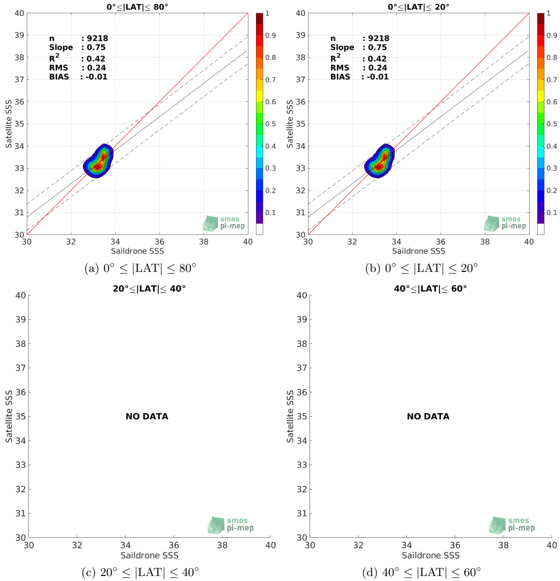
Figure 8: Contour maps of the concentration of SMAP SSS L3 v5.0 - 8-Day running (JPL) SSS (y-axis) versus Saildrone SSS (x-axis) at match-up pairs for different latitude bands. For each plot, the red line shows x=y . The black thin and dashed lines indicate a linear fit through the data cloud and the \pm 95\% confidence levels, respectively. The number match-up pairs n , the slope and R^2 coefficient of the linear fit, the root mean square (RMS) and the mean bias between satellite and in situ data are indicated for each latitude band in each plots.
