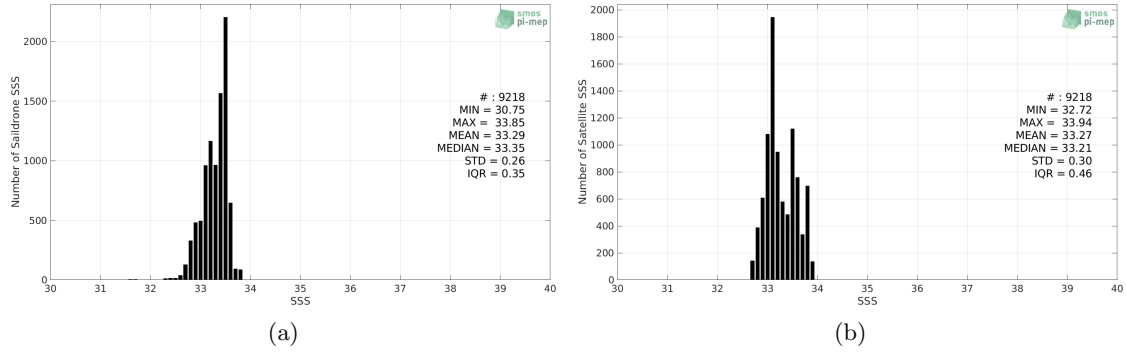
Figure 2: Histograms of SSS from Sairdrone (a) and SMAP SSS L3 v5.0 - 8-Day running (JPL) (b) considering all match-up pairs per bins of 0.1 over the SPURS 2 Pi-MEP region and for the full satellite product period.
