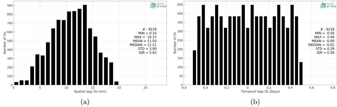
Figure 4: Histograms of the spatial (a) and temporal (b) lags between the location/time of the Saildrone measurement and the date of the corresponding SMAP SSS L3 v5.0 - 8-Day running (JPL) SSS pixel.
