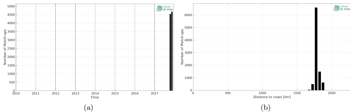
Figure 1: Number of match-ups between Saildrone and SMAP SSS L3 v5.0 - 8-Day running (JPL) SSS as a function of time (a) and as function of the distance to coast (b) over the SPURS 2 Pi-MEP region and for the full satellite product period.
