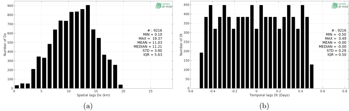
Figure 5: Histograms of the spatial (a) and temporal (b) lags between the time of the Sairdrone measurements and the date of the corresponding SMAP SSS L3 v5.0 - 8-Day running (JPL) SSS product.
