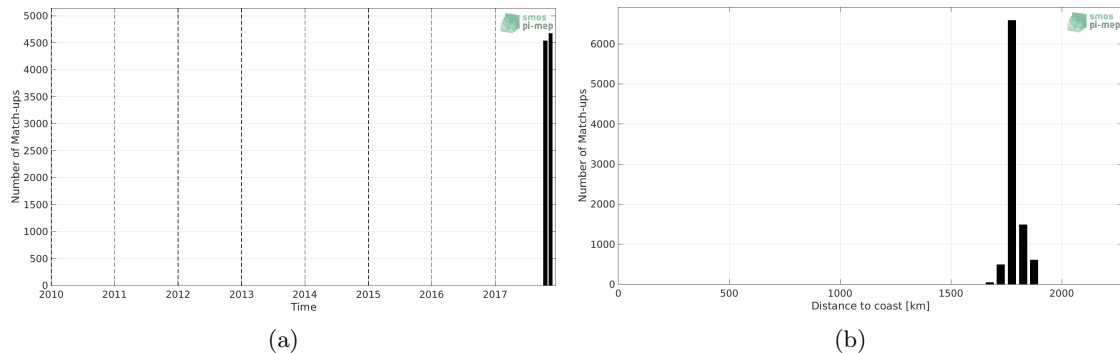
Figure 1: Number of match-ups between Sairdrone and SMAP SSS L3 v5.0 - 8-Day running (JPL) SSS as a function of time (a) and as function of the distance to coast (b) over the SPURS 2 Pi-MEP region and for the full satellite product period.
