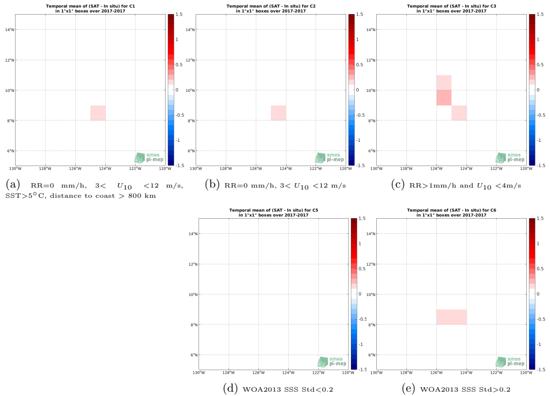
Figure 12: Temporal mean gridded over spatial boxes of size 1^\circ \times 1^\circ of \Delta SSS (SMAP SSS L3 v5.0 - 8-Day running (JPL) - Saildrone) for 5 different subdatasets corresponding to:RR=0 mm/h, 3 < U_{10} < 12 m/s, SST >5^\circ\text{C} , distance to coast > 800 km (a), RR=0 mm/h, 3 < U_{10} < 12 m/s (b), RR >1 mm/h and U_{10} < 4 m/s (c), WOA2013 SSS Std <0.2 (d), WOA2013 SSS Std >0.2 (e).
