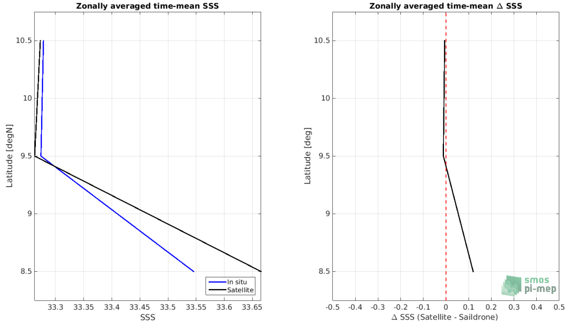
Figure 8: Left panel: Zonal mean SSS from SMAP SSS L3 v5.0 - 8-Day running (JPL) satellite product (black) and from Saikdrone (blue). Right panel: Zonal mean of \Delta SSS (Satellite - Saikdrone) for all the collected Pi-MEP match-up pairs estimated over the full satellite product period.
