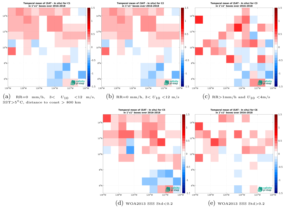
Figure 11: Temporal mean gridded over spatial boxes of size 1^\circ \times 1^\circ of \Delta\text{SSS} (SMAP SSS L3 v5.0 - 8-Day running (JPL) - Surface drifters) for 5 different subdatasets corresponding to:RR=0 mm/h, 3 < U_{10} < 12 m/s, SST >5^\circ\text{C} , distance to coast > 800 km (a), RR=0 mm/h, 3 < U_{10} < 12 m/s (b), RR >1 mm/h and U_{10} < 4 m/s (c), WOA2013 SSS Std <0.2 (d), WOA2013 SSS Std >0.2 (e).
