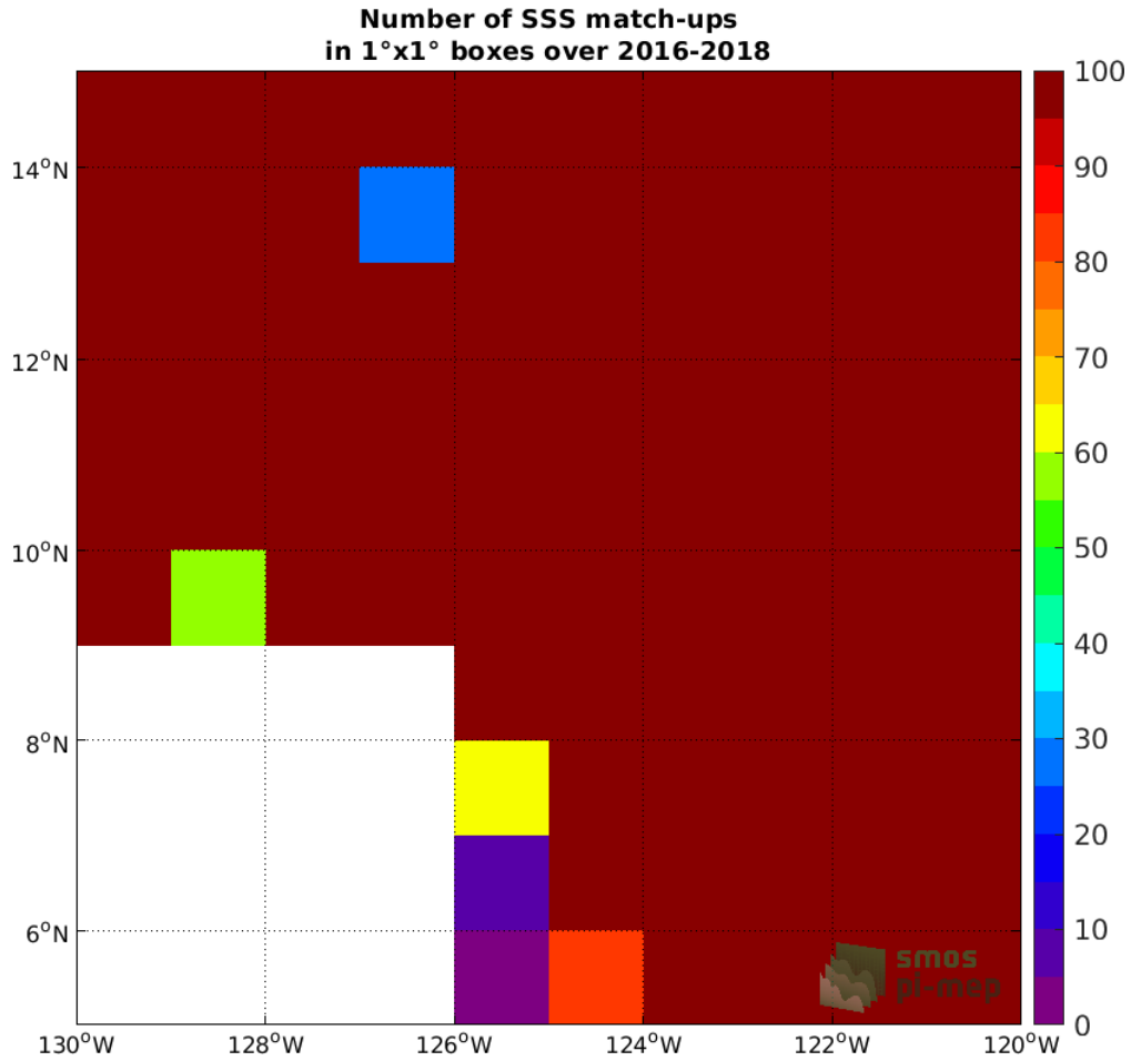
Figure 3: Number of SSS match-ups between Surface drifters SSS and the SMAP SSS L3 v5.0 - 8-Day running (JPL) SSS product for the SPURS 2 Pi-MEP region over 1^\circ \times 1^\circ boxes and for the full satellite product period.
