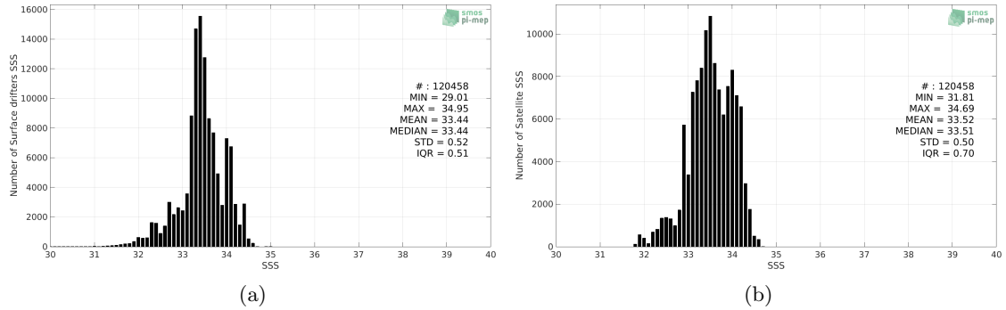
Figure 2: Histograms of SSS from Surface drifters (a) and SMAP SSS L3 v5.0 - 8-Day running (JPL) (b) considering all match-up pairs per bins of 0.1 over the SPURS 2 Pi-MEP region and for the full satellite product period.
