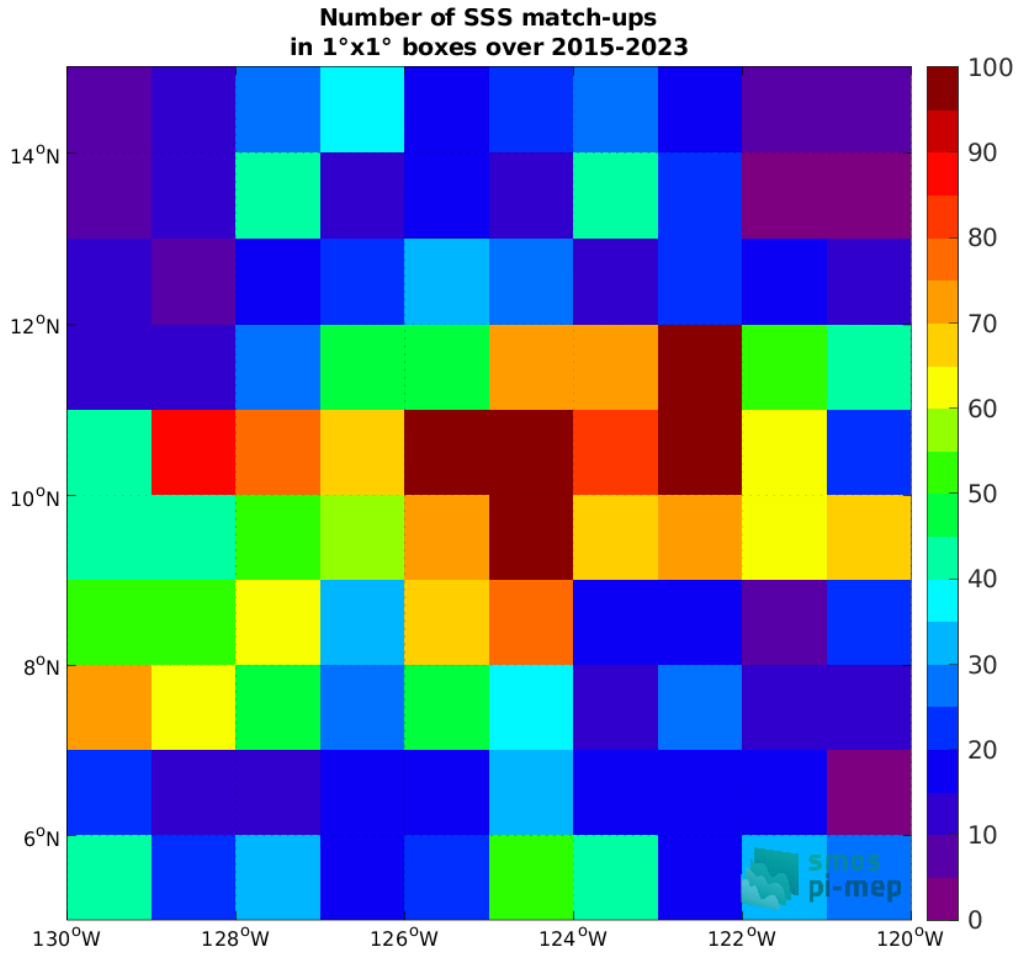
Figure 4: Number of SSS match-ups between Argo SSS and the SMAP SSS L3 v5.0 - 8-Day running (JPL) SSS product for the SPURS 2 Pi-MEP region over 1°x1° boxes and for the full satellite product period.
