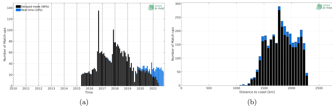
Figure 1: Number of match-ups between Argo and SMAP SSS L3 v5.0 - 8-Day running (JPL) SSS as a function of time (a) and as function of the distance to coast (b) over the SPURS 2 Pi-MEP region and for the full satellite product period.
