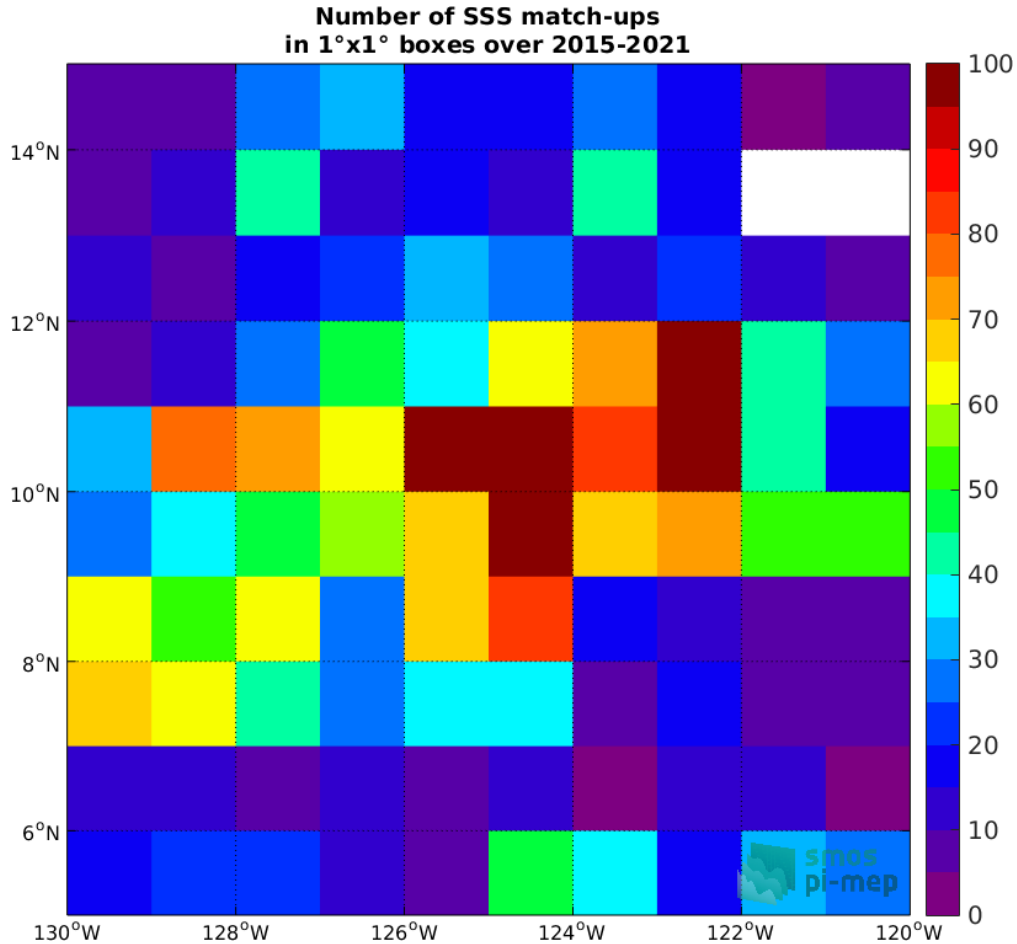
Figure 4: Number of SSS match-ups between Argo SSS and the SMAP SSS L3 v5.0 - 8-Day running (JPL) SSS product for the SPURS 2 Pi-MEP region over 1^\circ \times 1^\circ boxes and for the full satellite product period.
