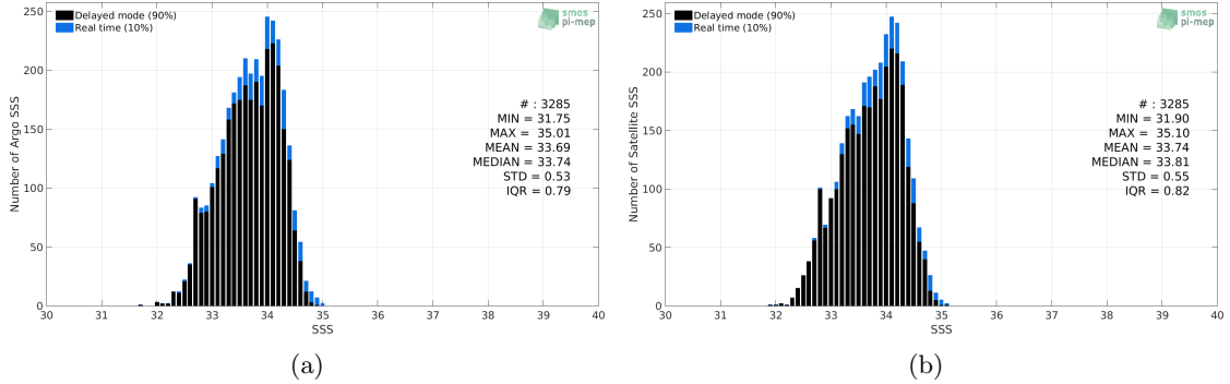
Figure 2: Histograms of SSS from Argo (a) and SMAP SSS L3 v5.0 - 8-Day running (JPL) (b) considering all match-up pairs per bins of 0.1 over the SPURS 2 Pi-MEP region and for the full satellite product period.
