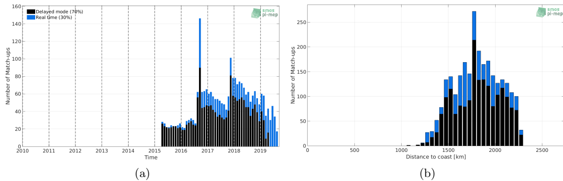
Figure 1: Number of match-ups between Argo and SMAP-L3-JPL-V4.3-MONTHLY-60KM SSS as a function of time (a) and as function of the distance to coast (b) over the SPURS 2 Pi-MEP region and for the full satellite product period.
