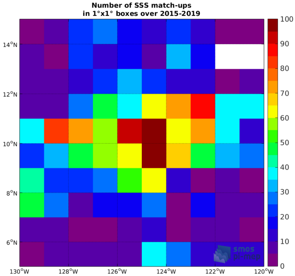
Figure 4: Number of SSS match-ups between Argo SSS and the SMAP-L3-JPL-V4.3-MONTHLY-60KM SSS product for the SPURS 2 Pi-MEP region over 1°x1° boxes and for the full satellite product period.
