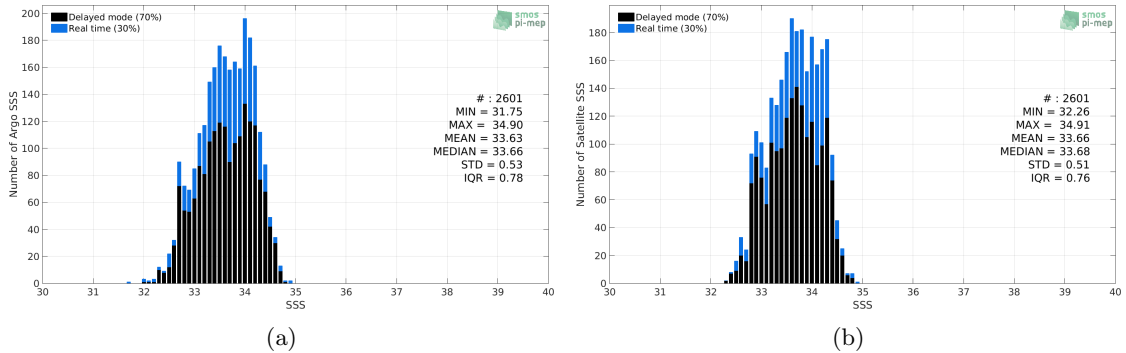
Figure 2: Histograms of SSS from Argo (a) and SMAP-L3-JPL-V4.3-MONTHLY-60KM (b) considering all match-up pairs per bins of 0.1 over the SPURS 2 Pi-MEP region and for the full satellite product period.
