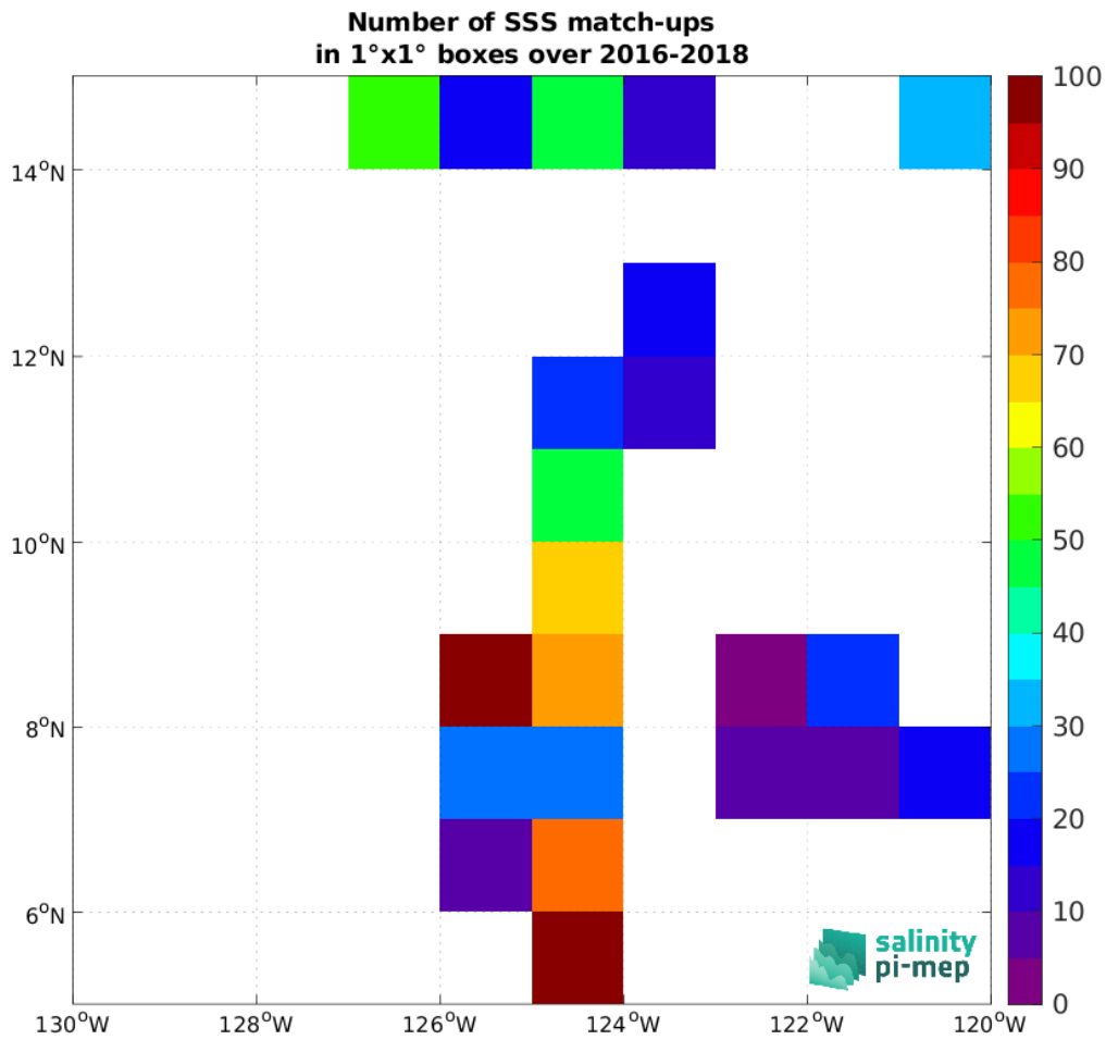
Figure 5: Number of SSS match-ups between TSG (SAMOS) SSS and the SMAP SSS L2 v6 (RSS) SSS product for the SPURS 2 Pi-MEP region over 1°x1° boxes and for the full satellite product period.
