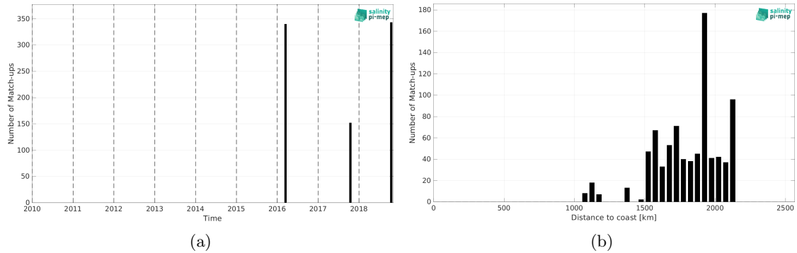
Figure 2: Number of match-ups between TSG (SAMOS) and SMAP SSS L2 v6 (RSS) SSS as a function of time (a) and as function of the distance to coast (b) over the SPURS 2 Pi-MEP region and for the full satellite product period.
