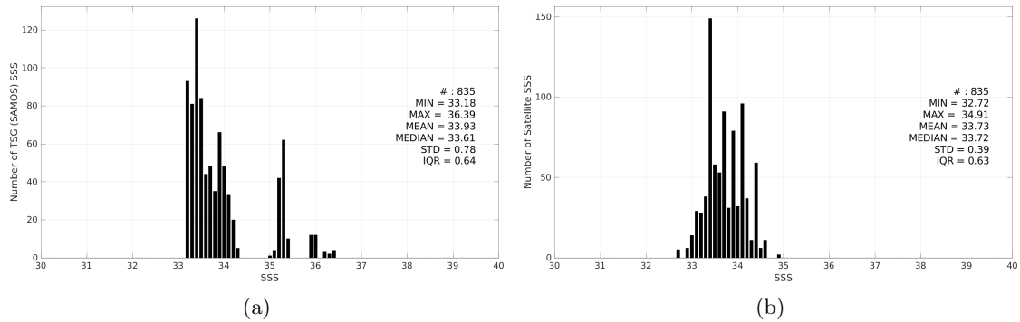
Figure 3: Histograms of SSS from TSG (SAMOS) (a) and SMAP SSS L2 v6 (RSS) (b) considering all match-up pairs per bins of 0.1 over the SPURS 2 Pi-MEP region and for the full satellite product period.
