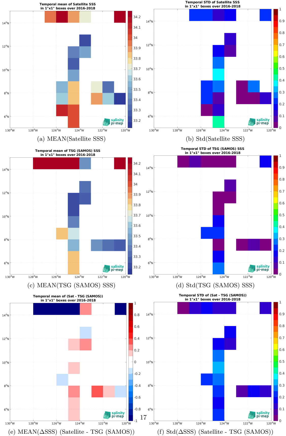
Figure 7: Temporal mean (left) and Std (right) of SSS from SMAP SSS L2 v6 (RSS) (top), TSG (SAMOS) (middle), and of \Delta SSS (Satellite - TSG (SAMOS)). Only match-up pairs are used to generate these maps.
