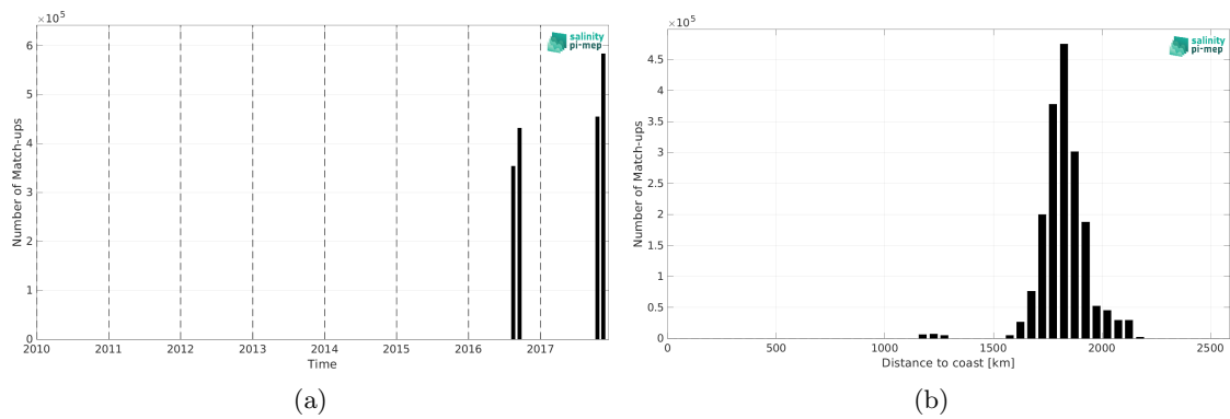
Figure 2: Number of match-ups between Salinity Snake (SPURS 2) and SMAP SSS L2 v6 (RSS) SSS as a function of time (a) and as function of the distance to coast (b) over the SPURS 2 Pi-MEP region and for the full satellite product period.
