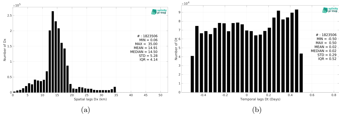
Figure 6: Histograms of the spatial (a) and temporal (b) lags between the location/time of the Salinity Snake (SPURS 2) measurement and the date of the corresponding SMAP SSS L2 v6 (RSS) SSS pixel.
