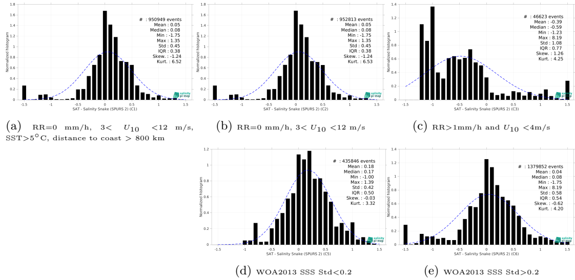
Figure 15: Normalized histogram of \Delta SSS (SMAP SSS L2 v6 (RSS) - Salinity Snake (SPURS 2)) for 5 different subdatasets corresponding to: RR=0 mm/h, 3 < U_{10} < 12 m/s, SST > 5°C, distance to coast > 800 km (a), RR=0 mm/h, 3 < U_{10} < 12 m/s (b), RR > 1mm/h and U_{10} < 4 m/s (c), WOA2013 SSS Std < 0.2 (d), WOA2013 SSS Std > 0.2 (e).
