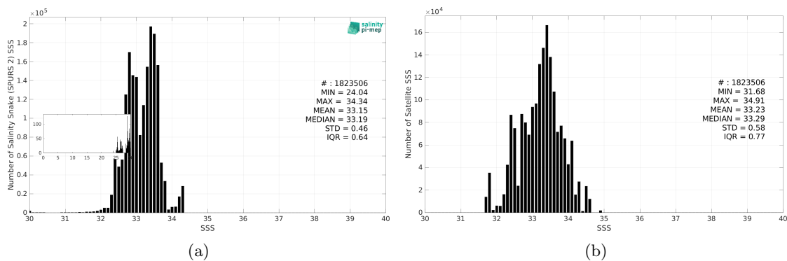
Figure 3: Histograms of SSS from Salinity Snake (SPURS 2) (a) and SMAP SSS L2 v6 (RSS) (b) considering all match-up pairs per bins of 0.1 over the SPURS 2 Pi-MEP region and for the full satellite product period.
