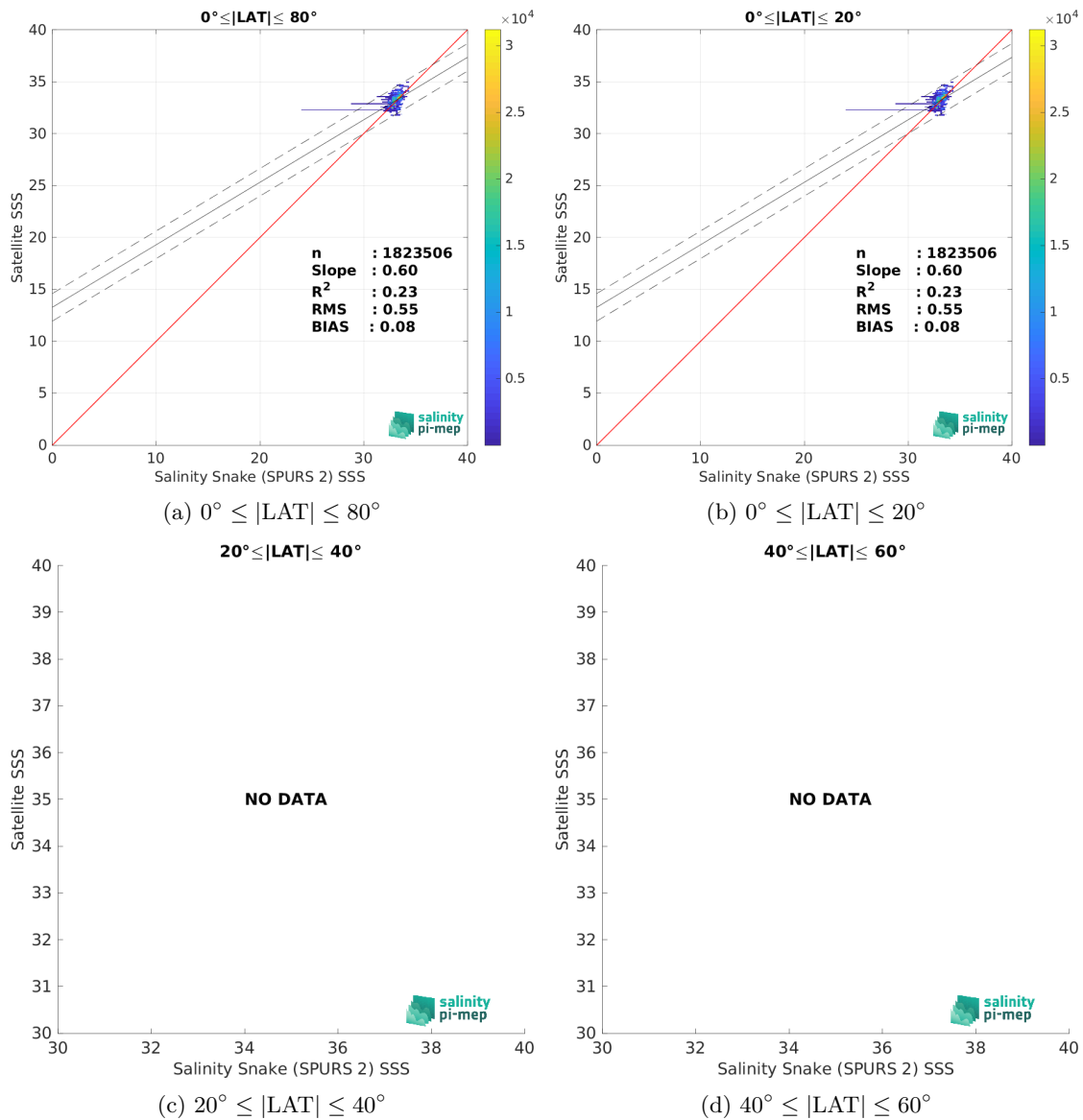
Figure 10: Contour maps of the concentration of SMAP SSS L2 v6 (RSS) SSS (y-axis) versus Salinity Snake (SPURS 2) SSS (x-axis) at match-up pairs for different latitude bands. For each plot, the red line shows x=y . The black thin and dashed lines indicate a linear fit through the data cloud and the \pm 95\% confidence levels, respectively. The number match-up pairs n , the slope and R^2 coefficient of the linear fit, the root mean square (RMS) and the mean bias between satellite and in situ data are indicated for each latitude band in each plots.
