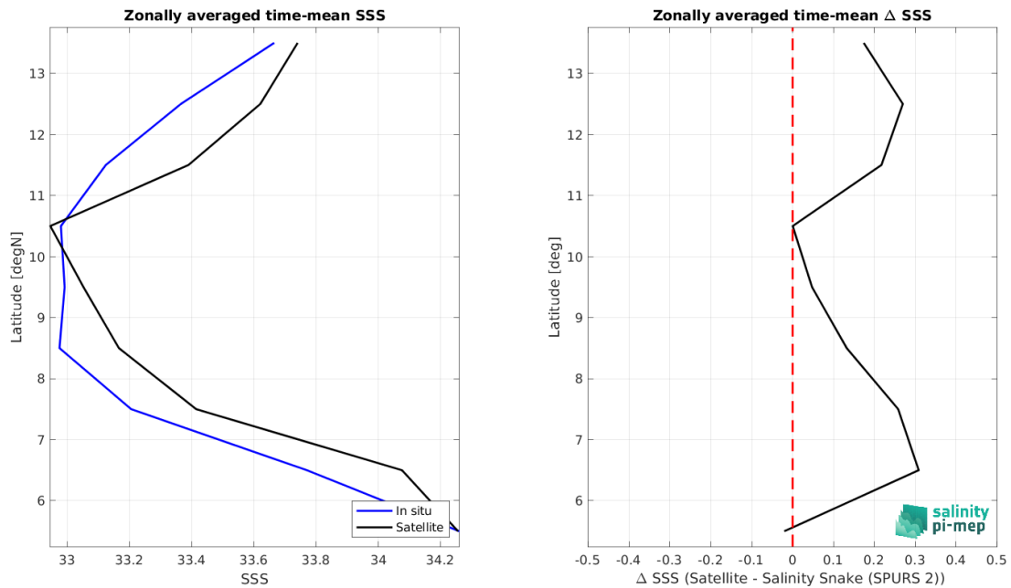
Figure 9: Left panel: Zonal mean SSS from SMAP SSS L2 v6 (RSS) satellite product (black) and from Salinity Snake (SPURS 2) (blue). Right panel: Zonal mean of \Delta SSS (Satellite - Salinity Snake (SPURS 2)) for all the collected Pi-MEP match-up pairs estimated over the full satellite product period.
