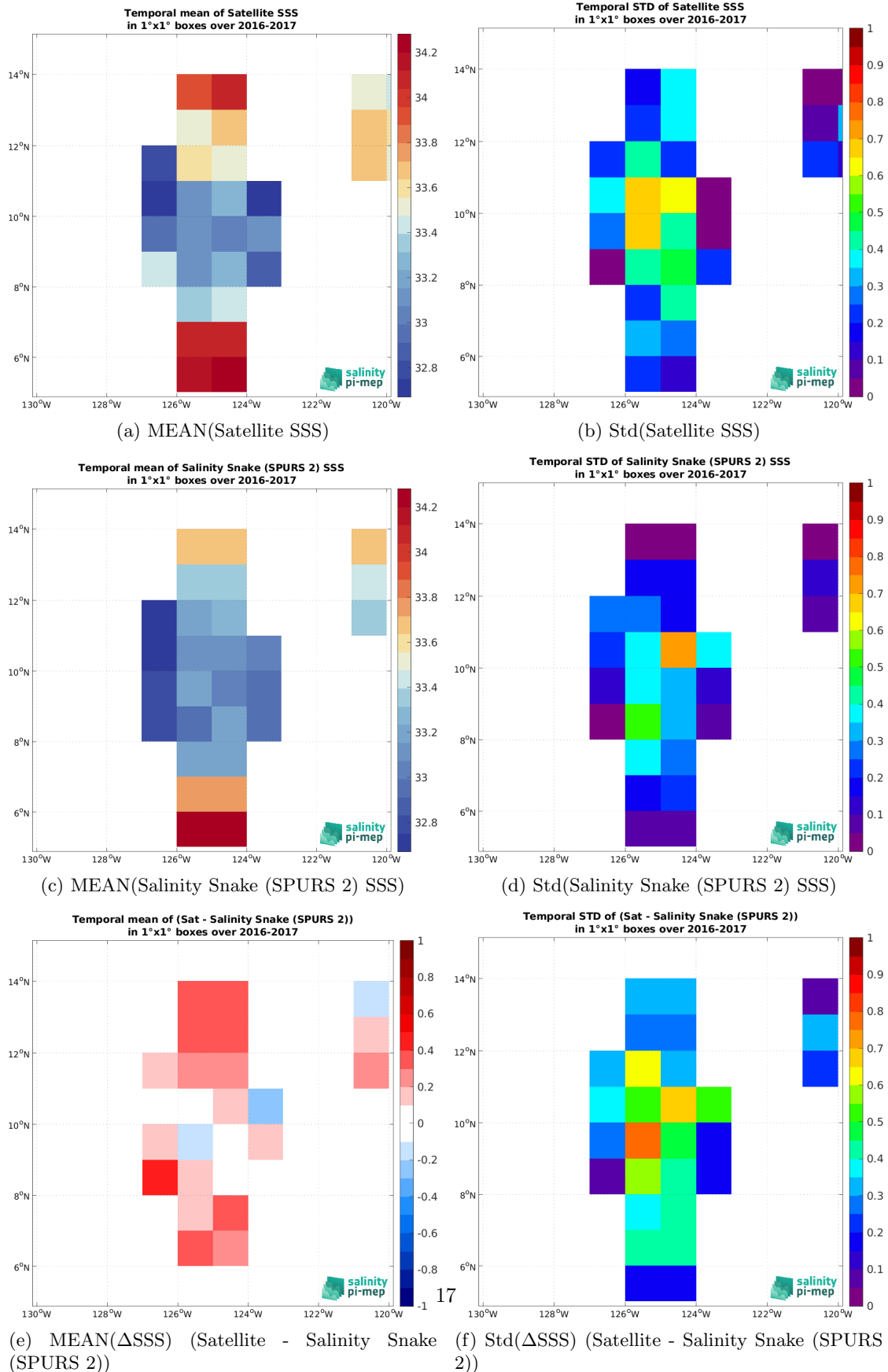
Figure 7: Temporal mean (left) and Std (right) of SSS from SMAP SSS L2 v6 (RSS) (top), Salinity Snake (SPURS 2) (middle), and of \Delta SSS (Satellite - Salinity Snake (SPURS 2)). Only match-up pairs are used to generate these maps.
