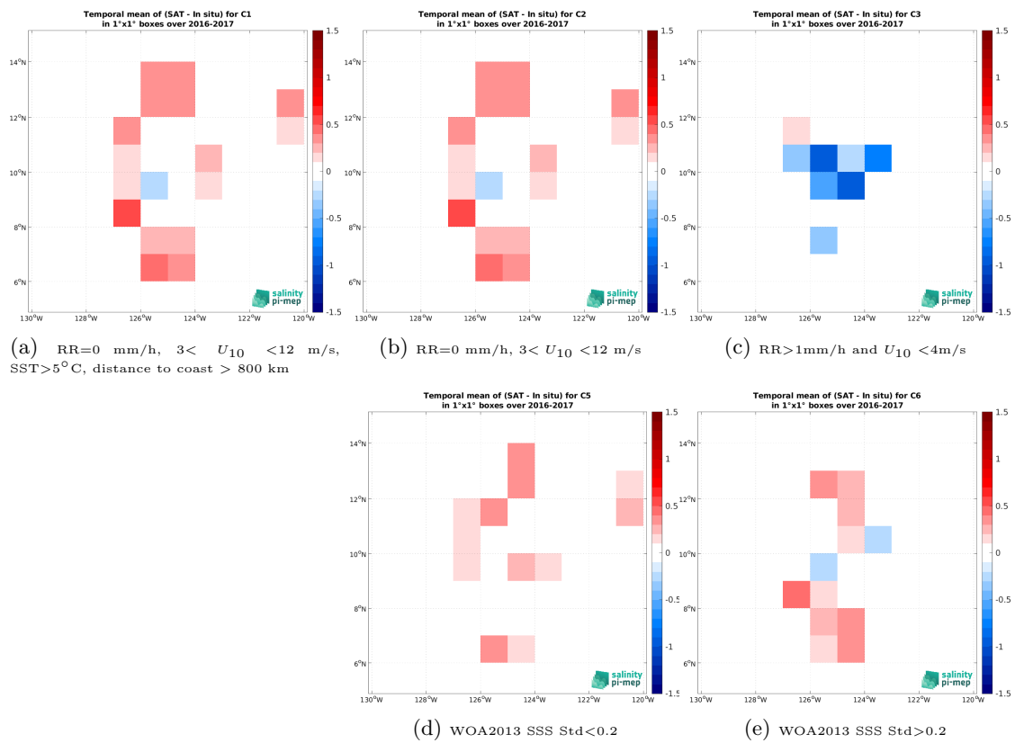
Figure 14: Temporal mean gridded over spatial boxes of size 1^\circ \times 1^\circ of \Delta\text{SSS} (SMAP SSS L2 v6 (RSS) - Salinity Snake (SPURS 2)) for 5 different subdatasets corresponding to:RR=0 mm/h, 3 < U_{10} < 12 m/s, SST>5°C, distance to coast > 800 km (a), RR=0 mm/h, 3 < U_{10} < 12 m/s (b), RR>1mm/h and U_{10} < 4 m/s (c), WOA2013 SSS Std<0.2 (d), WOA2013 SSS Std>0.2 (e).
