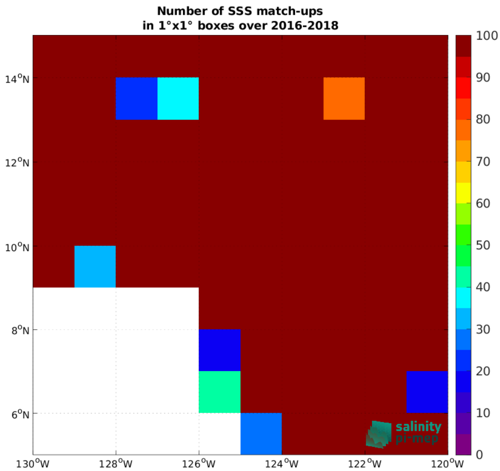
Figure 4: Number of SSS match-ups between Surface drifters SSS and the SMAP SSS L2 v6 (RSS) SSS product for the SPURS 2 Pi-MEP region over 1°x1° boxes and for the full satellite product period.
