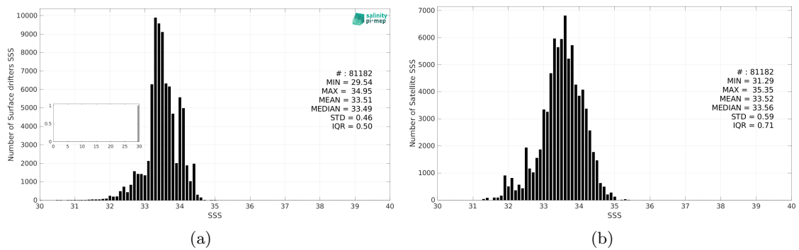
Figure 3: Histograms of SSS from Surface drifters (a) and SMAP SSS L2 v6 (RSS) (b) considering all match-up pairs per bins of 0.1 over the SPURS 2 Pi-MEP region and for the full satellite product period.
