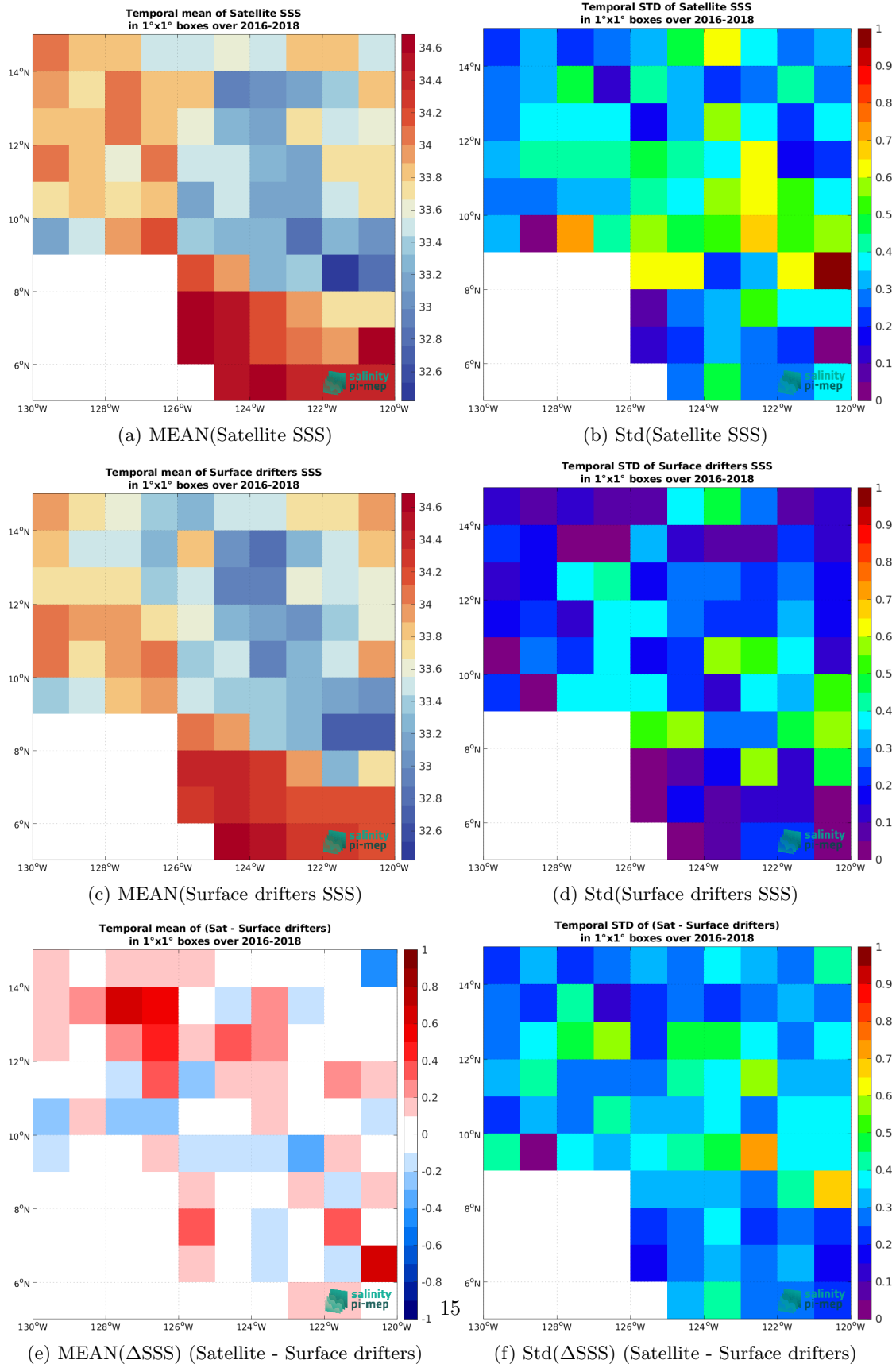
Figure 6: Temporal mean (left) and Std (right) of SSS from SMAP SSS L2 v6 (RSS) (top), Surface drifters (middle), and of \Delta SSS (Satellite - Surface drifters). Only match-up pairs are used to generate these maps.
