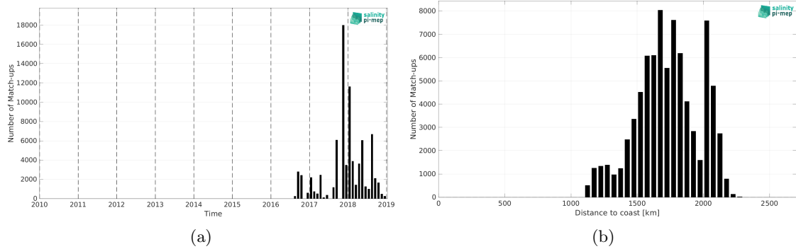
Figure 2: Number of match-ups between Surface drifters and SMAP SSS L2 v6 (RSS) SSS as a function of time (a) and as function of the distance to coast (b) over the SPURS 2 Pi-MEP region and for the full satellite product period.
