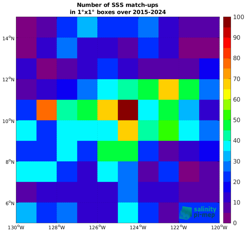
Figure 5: Number of SSS match-ups between Argo SSS and the SMAP SSS L2 v6 - 40 km (RSS) SSS product for the SPURS 2 Pi-MEP region over 1°x1° boxes and for the full satellite product period.
