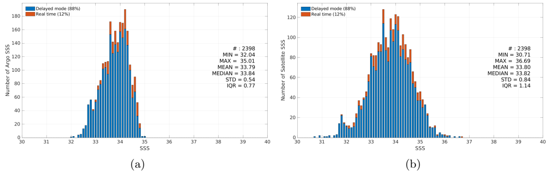
Figure 3: Histograms of SSS from Argo (a) and SMAP SSS L2 v6 - 40 km (RSS) (b) considering all match-up pairs per bins of 0.1 over the SPURS 2 Pi-MEP region and for the full satellite product period.
