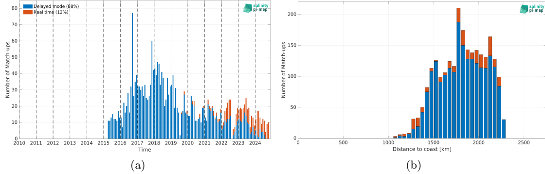
Figure 2: Number of match-ups between Argo and SMAP SSS L2 v6 - 40 km (RSS) SSS as a function of time (a) and as function of the distance to coast (b) over the SPURS 2 Pi-MEP region and for the full satellite product period.
